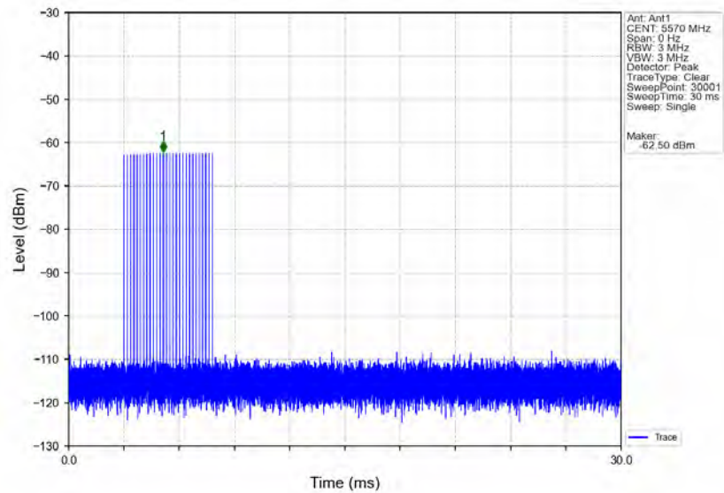
Signal Calibration_802.11ax(HEW160)_2C_5570MHz_RadarType3_Trial0
