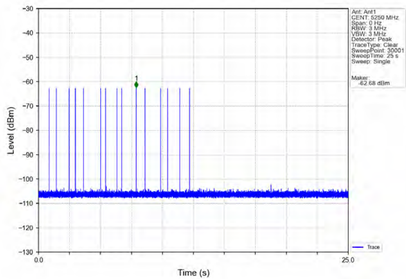
Signal Calibration_802.11ax(HEW160)_2A_5250MHz_RadarType5_Trial0
