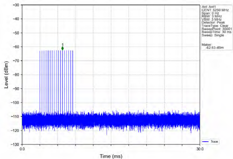
Signal Calibration_802.11ax(HEW160)_2A_5250MHz_RadarType3_Trial0
