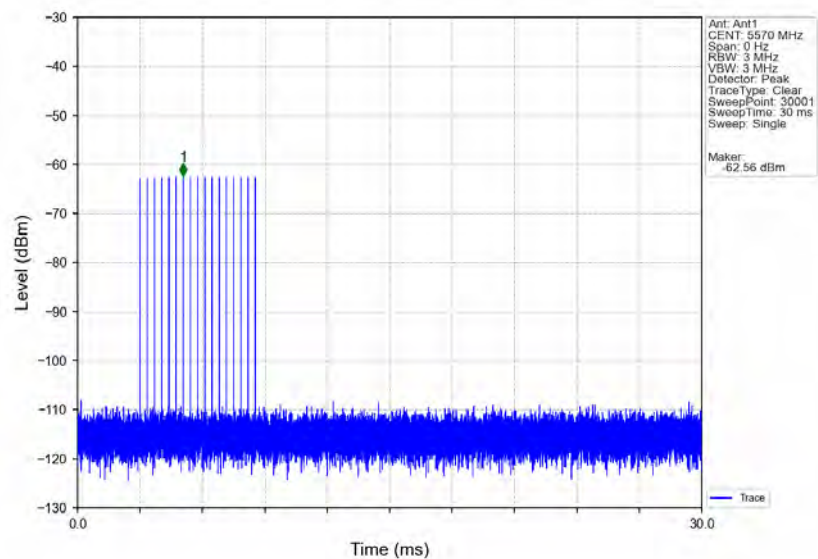
Signal Calibration_802.11ax(HEW160)_2C_5570MHz_RadarType3_Trial0
