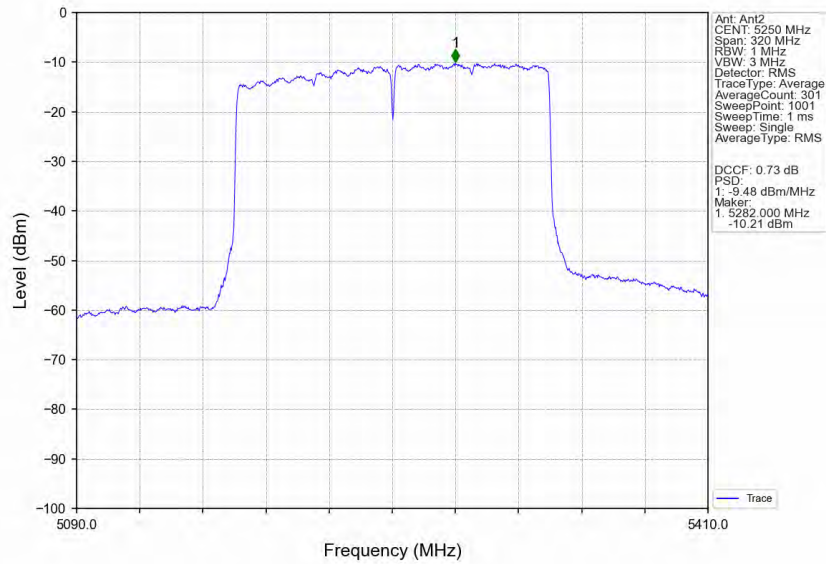
802.11ax(HEW160) MCH 5250MHz 2xRU996 Left MIMO NTNV
