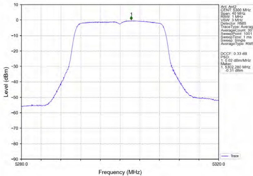
802.11ac(VHT20) MCH_5300MHz_Ant2_NTNV
