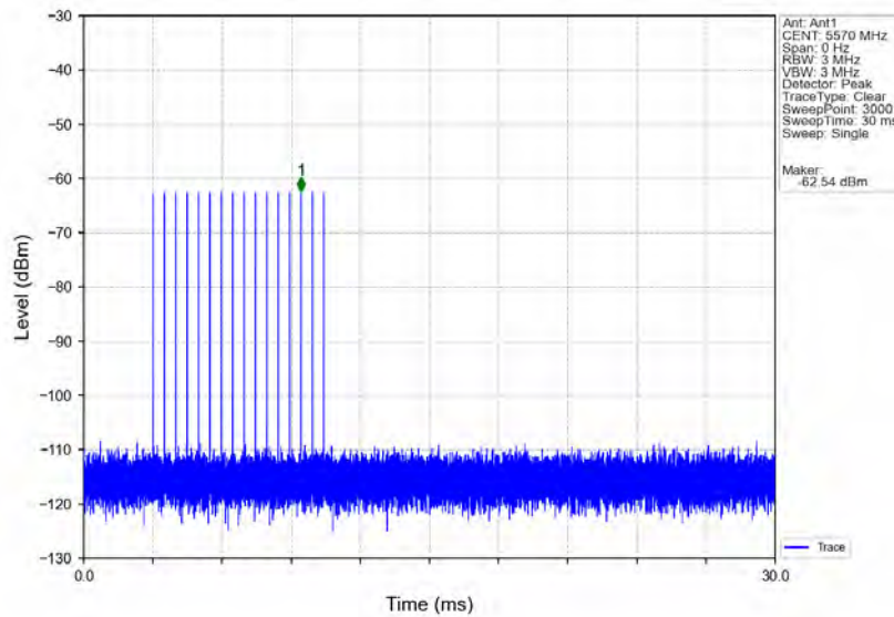
Signal Calibration_802.11ax(HEW160)_2C_5570MHz_RadarType5_Trial0
