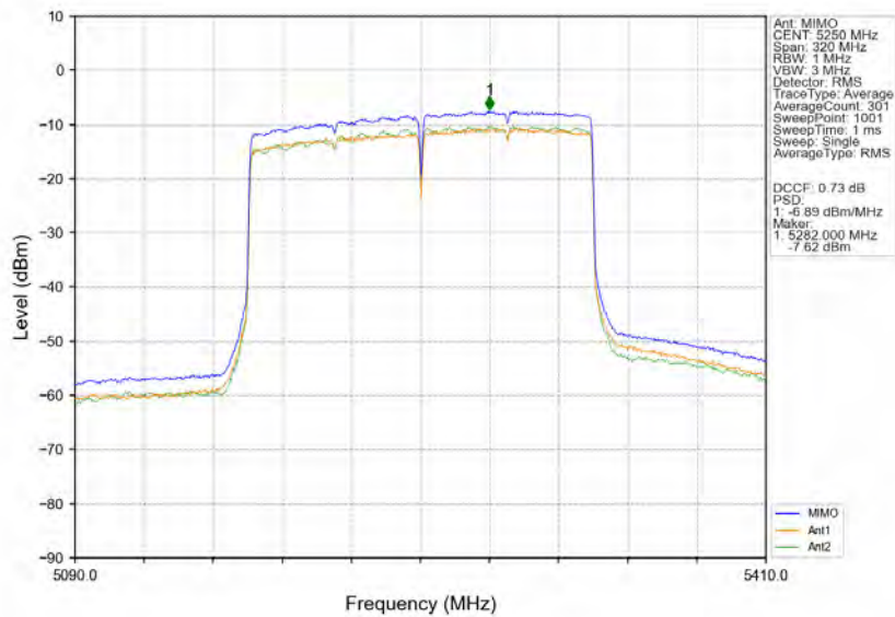
802.11ax(HEW160) MCH 5250MHz 2xRU996 Left MIMO NTNV
