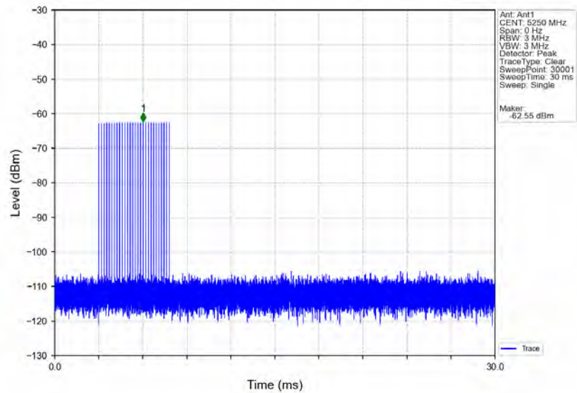
Signal Calibration_802.11ax(HEW160)_2A_5250MHz_RadarType3_Trial0
