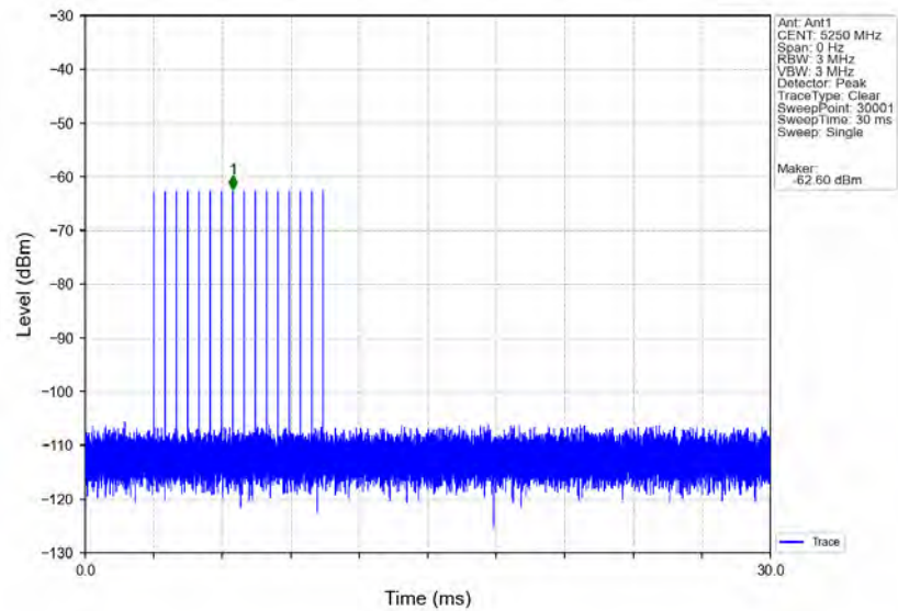
Signal Calibration_802.11ax(HEW160)_2A_5250MHz_RadarType5_Trial0
