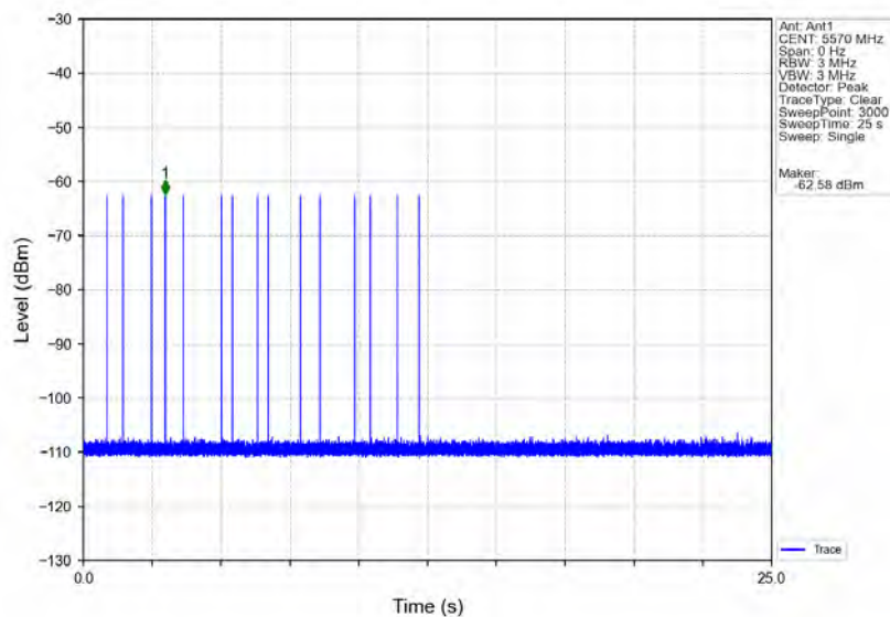
Signal Calibration_802.11ax(HEW160)_2C_5570MHz_RadarType5_Trial0
