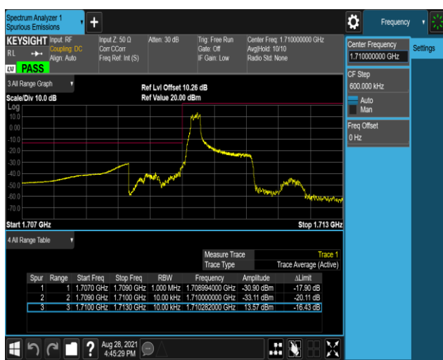
Band4-1.4MHz-QPSK-19957-6RB#0
