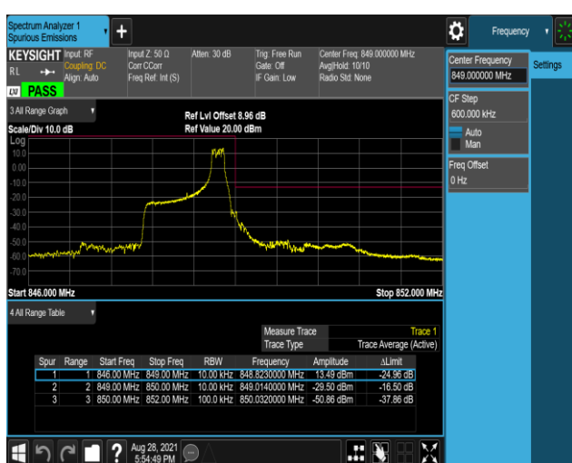
Band5-1.4MHz-QPSK-20643-1RB#5
