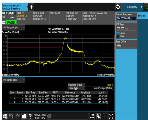
Band5-1.4MHz-16QAM-20647-6RB#0
