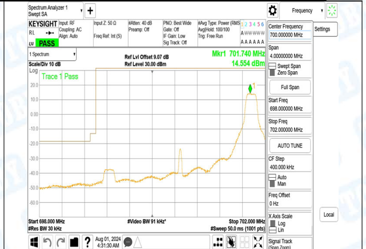
Band12_3MHz_QPSK_23165_1RB#0
