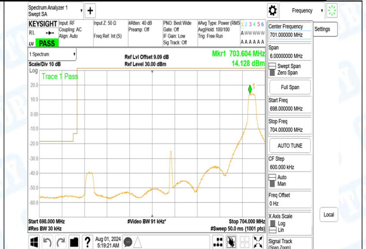
Band12_5MHz_16QAM_23155_1RB#0
