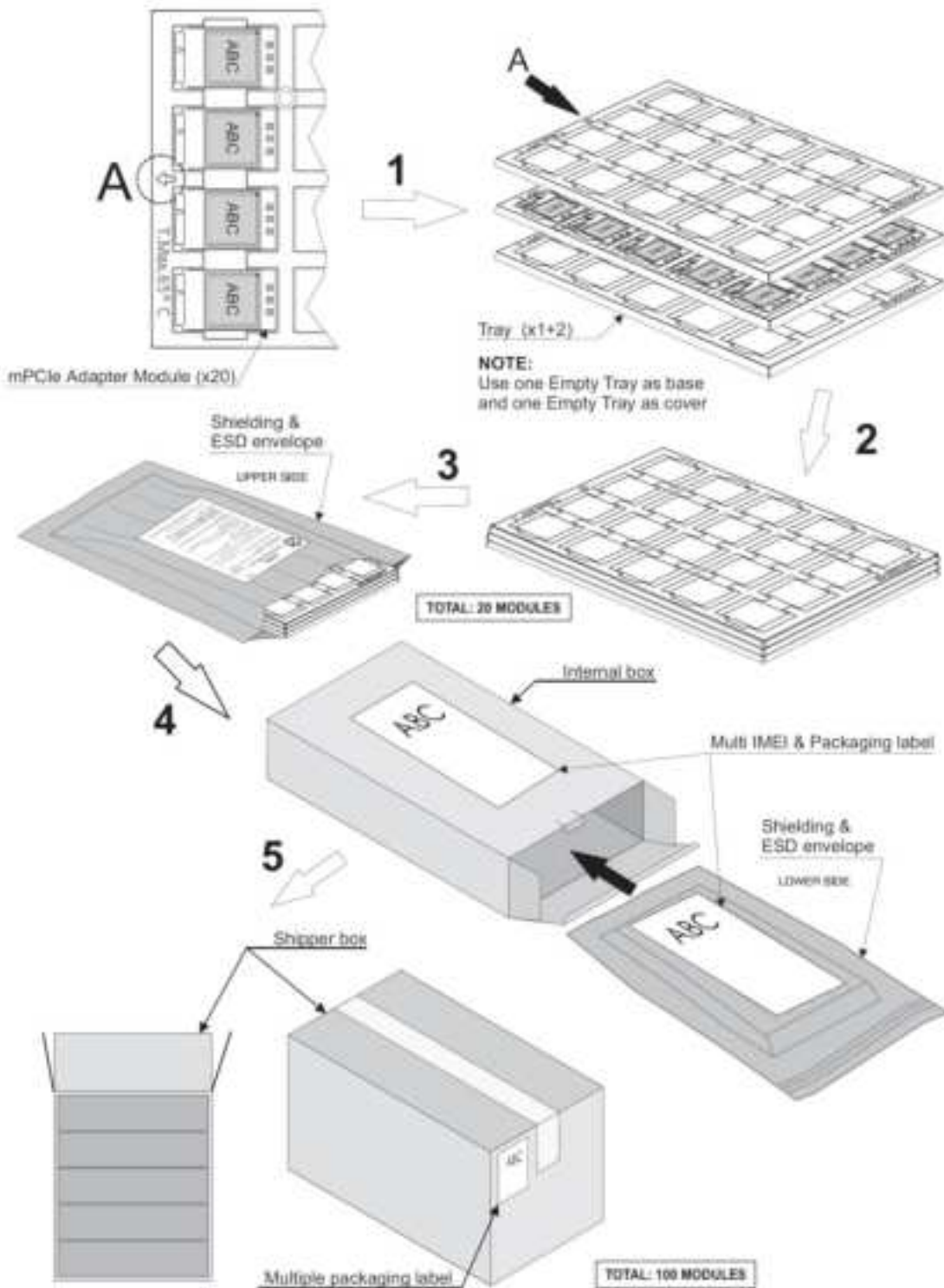
Figure 8: Tray Packaging
