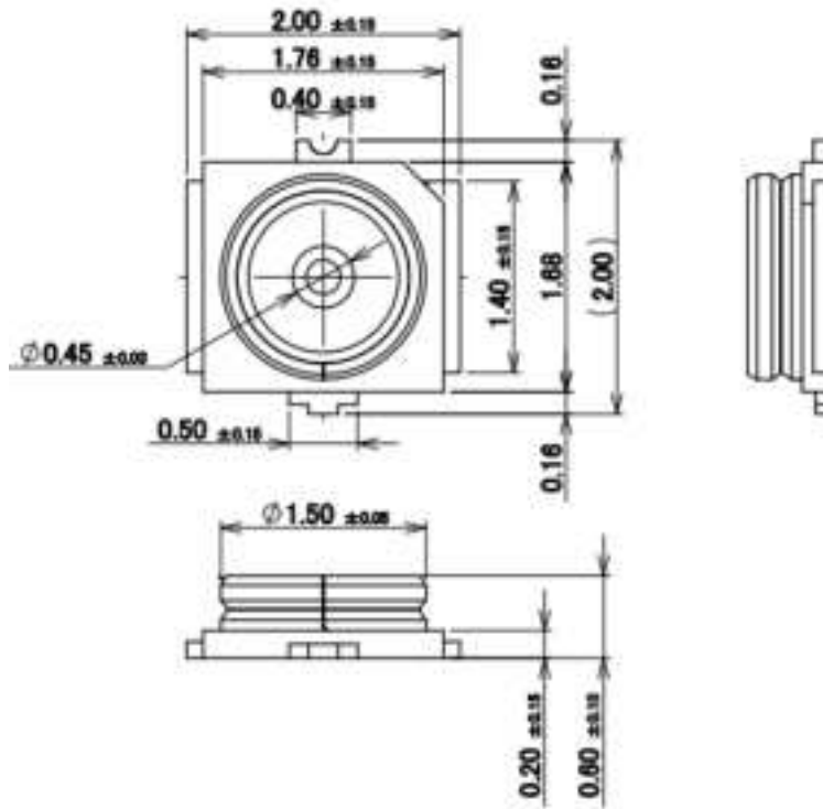
Figure 4: MHF-4 RF connector
