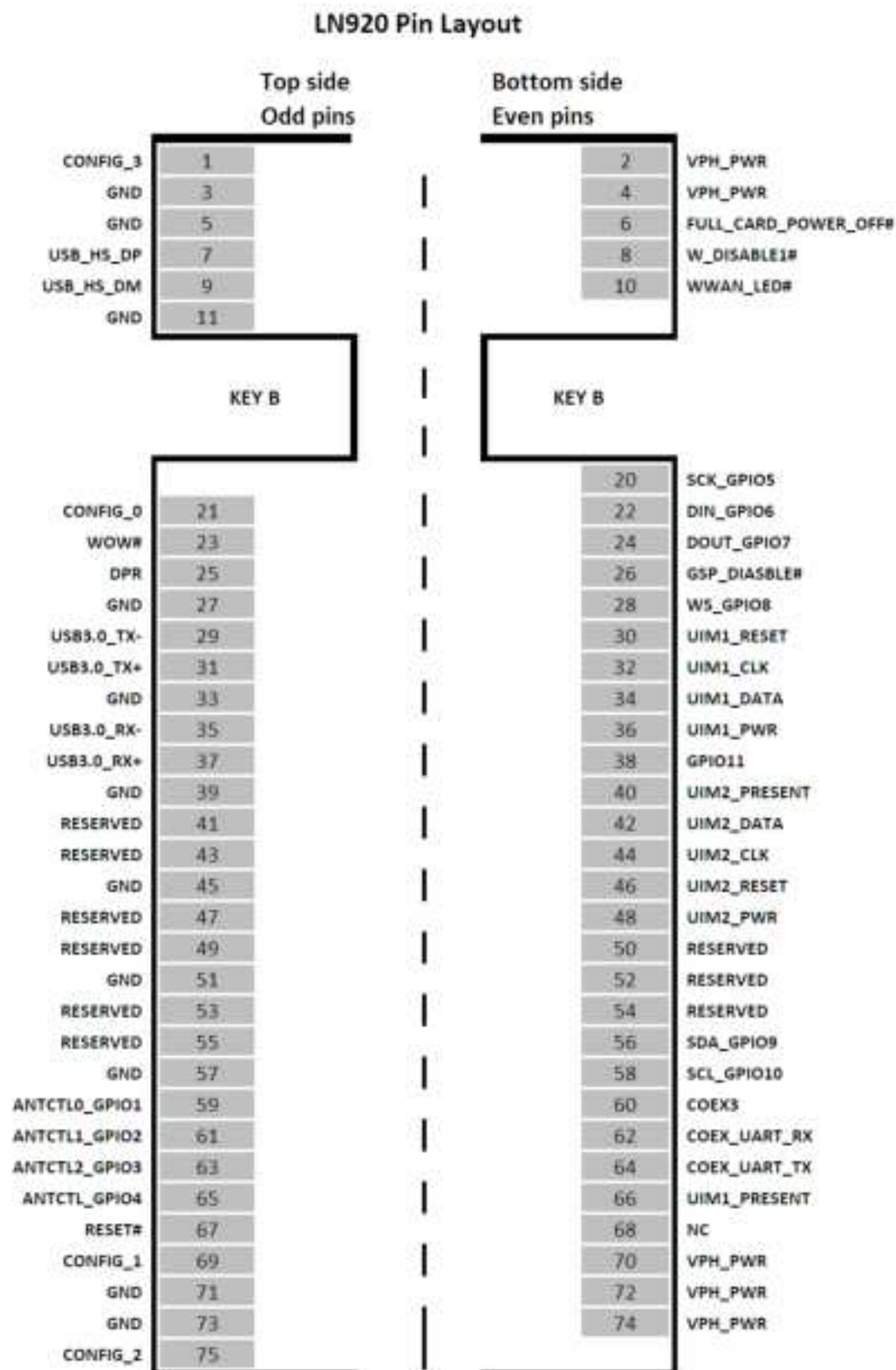
Figure 2: LN920 Pin-out
