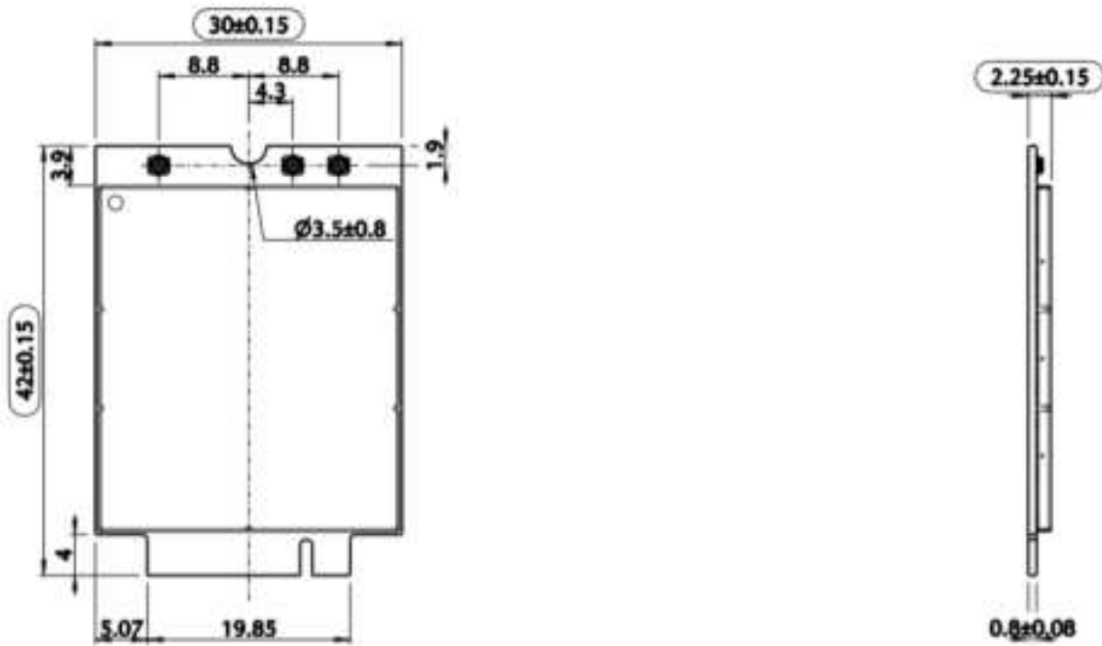
Figure 7: Mechanical Design Drawing
