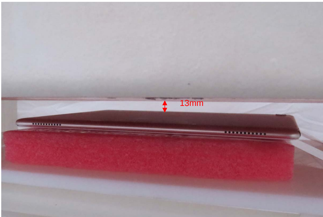
Picture 2: Back Side, the distance from handset to the bottom of the Phantom is 13mm
