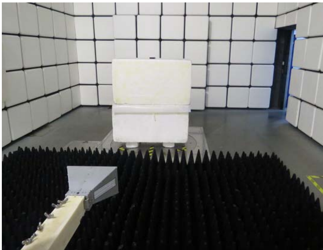
Picture 1 Radiated Emission Test Setup
