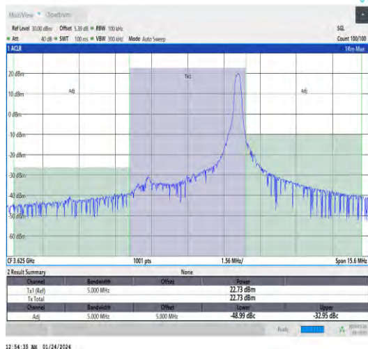
Band48-5MHz-QPSK-55990-1RB#24-PASS
