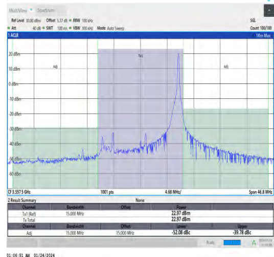
Band48-15MHz-QPSK-55315-1RB#74-PASS
