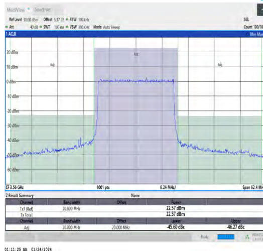
Band48-20MHz-QPSK-55340-100RB#0-PASS
