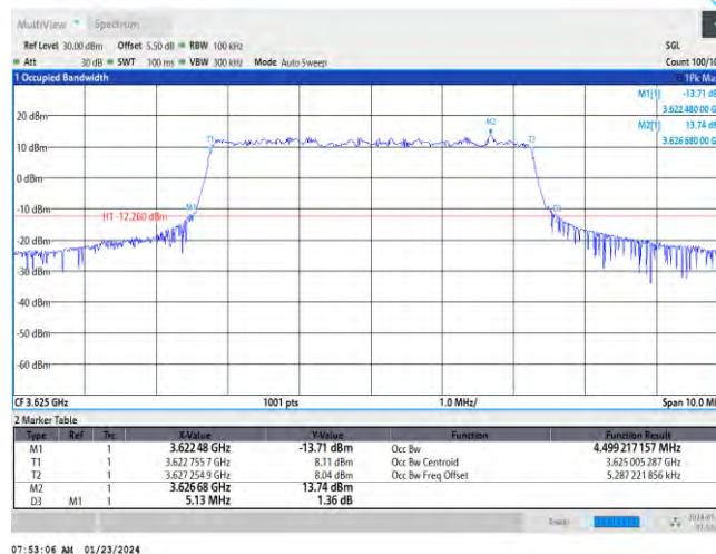
Band48-5MHz-16QAM-55990-25RB#0
