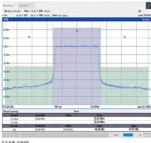
Band48-20MHz-QPSK-55990-100RB#0-PASS
