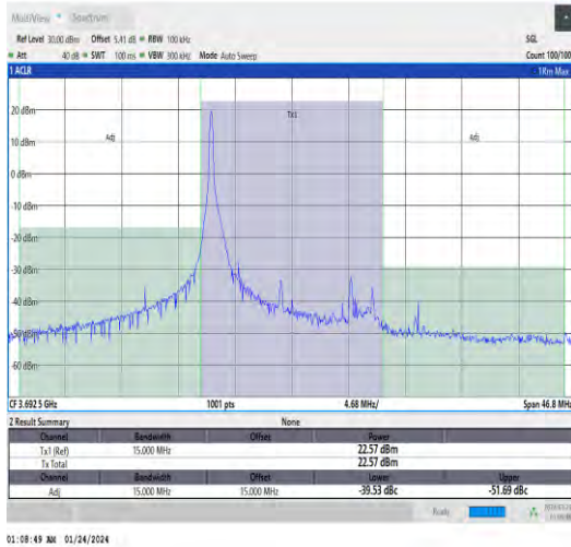
Band48-15MHz-QPSK-56665-1RB#0-PASS
