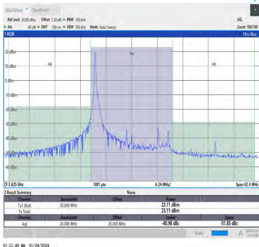
Band48-20MHz-QPSK-55990-1RB#0-PASS
