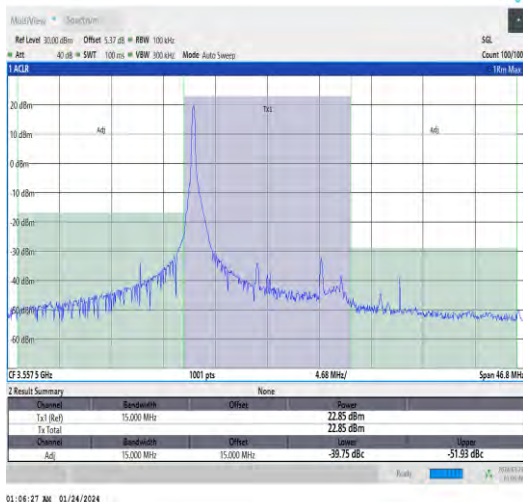
Band48-15MHz-QPSK-55315-1RB#0-PASS
