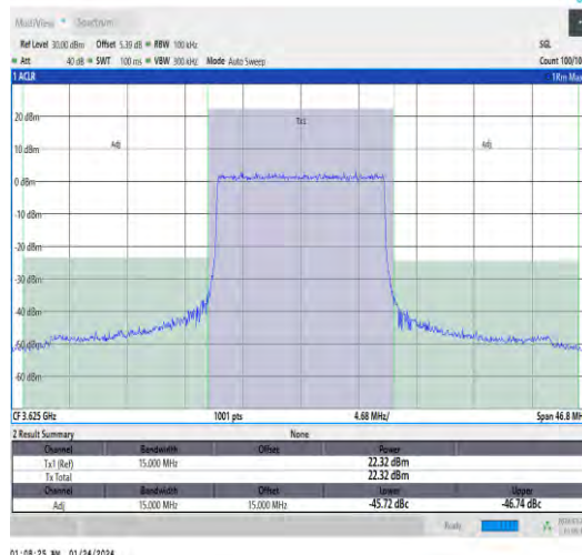
Band48-15MHz-QPSK-55990-75RB#0-PASS
