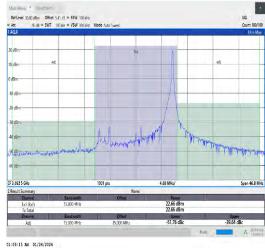
Band48-15MHz-QPSK-56665-1RB#74-PASS
