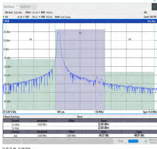
Band48-5MHz-QPSK-56715-1RB#0-PASS
