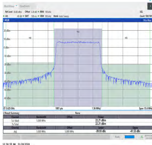
Band48-5MHz-QPSK-55990-25RB#0-PASS
