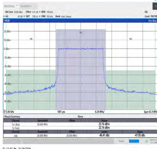
Band48-20MHz-QPSK-56640-100RB#0-PASS
