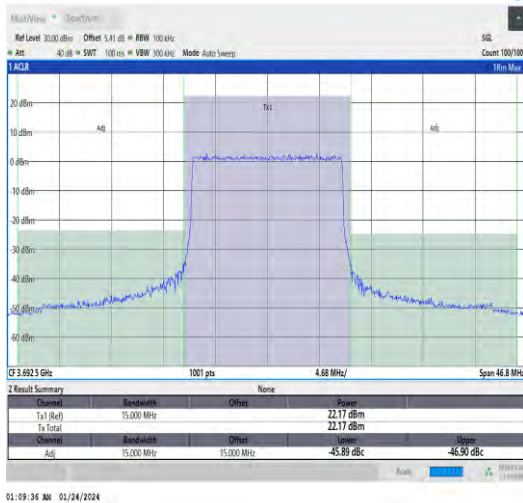
Band48-15MHz-QPSK-56665-75RB#0-PASS
