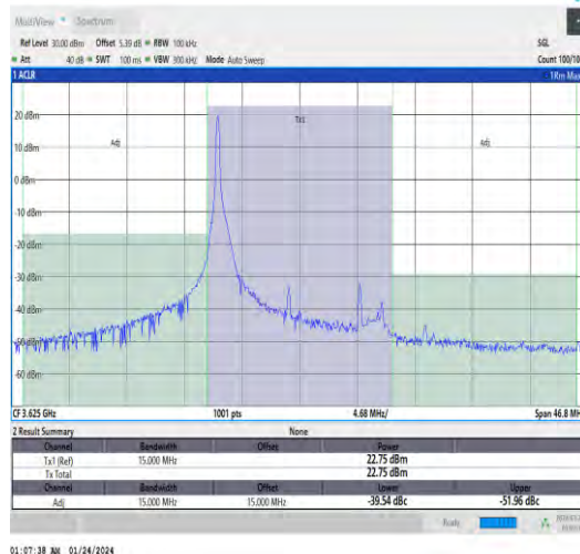
Band48-15MHz-QPSK-55990-1RB#0-PASS
