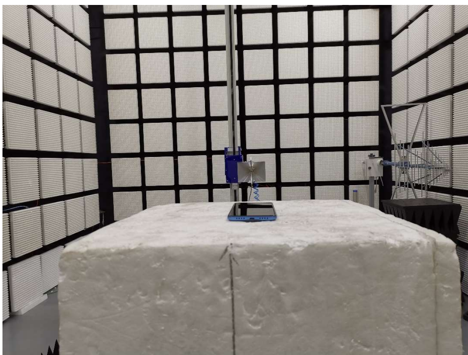
Field Strength of Spurious Radiation (3GHz - 10GHz)
