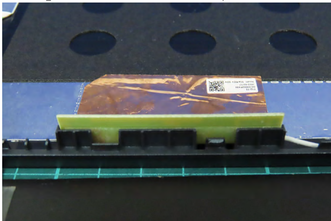
(34) EUT Photo _Antenna: SOUTHSTAR TECHNOLOGY CO.,LTD
