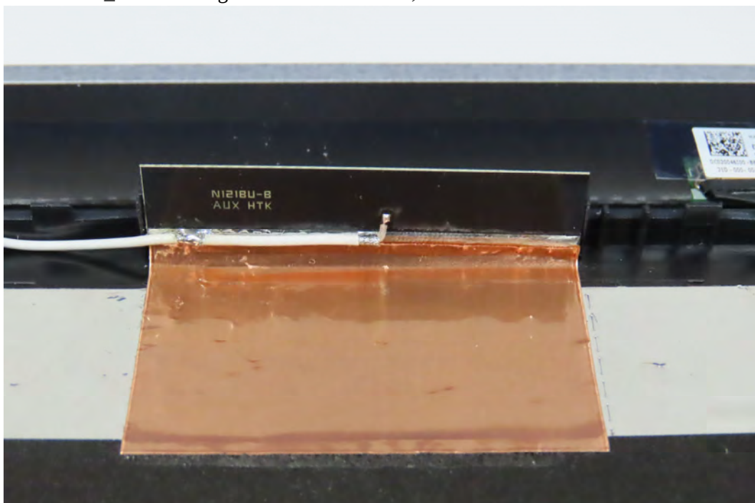
(37) EUT Photo _Antenna: High-Tek Electronics Co., Ltd.
