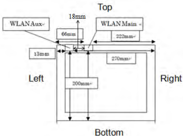
Fig.10 Antenna position of EUT (Front view of the tablet mode)
