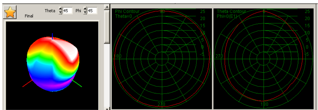
TDD-B40
