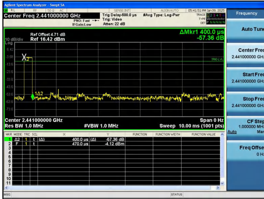
Dwell_Time_(Hopping)_NVNT_ANT1_2-DH1_2441_00_Accumulated
