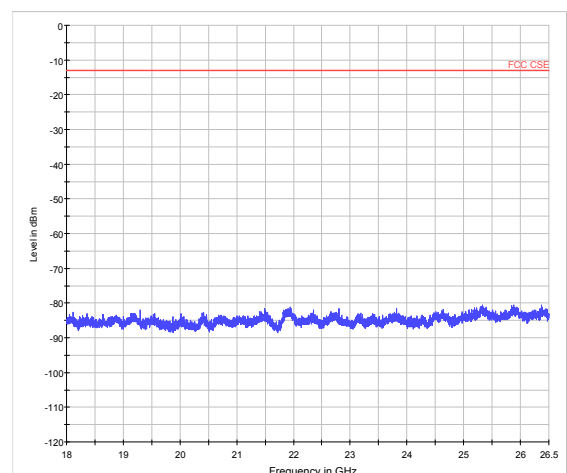
LTE Band 4 20MHz CH-High 18GHz ~26.5GHz
