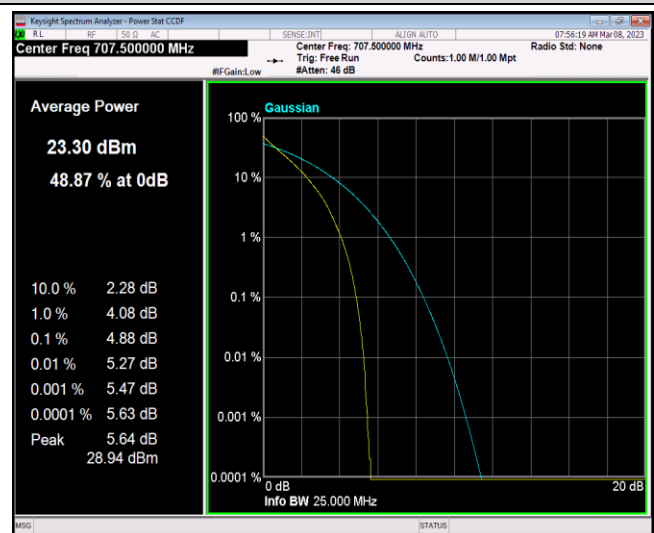
Band12-10MHz-64QAM-23095-50RB#0
