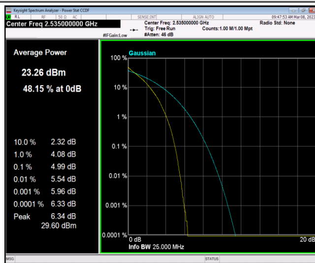
Band7-20MHz-64QAM-21100-100RB#0
