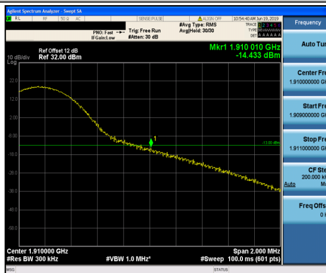
Band2_15MHz_16QAM_19125_1RB#74
