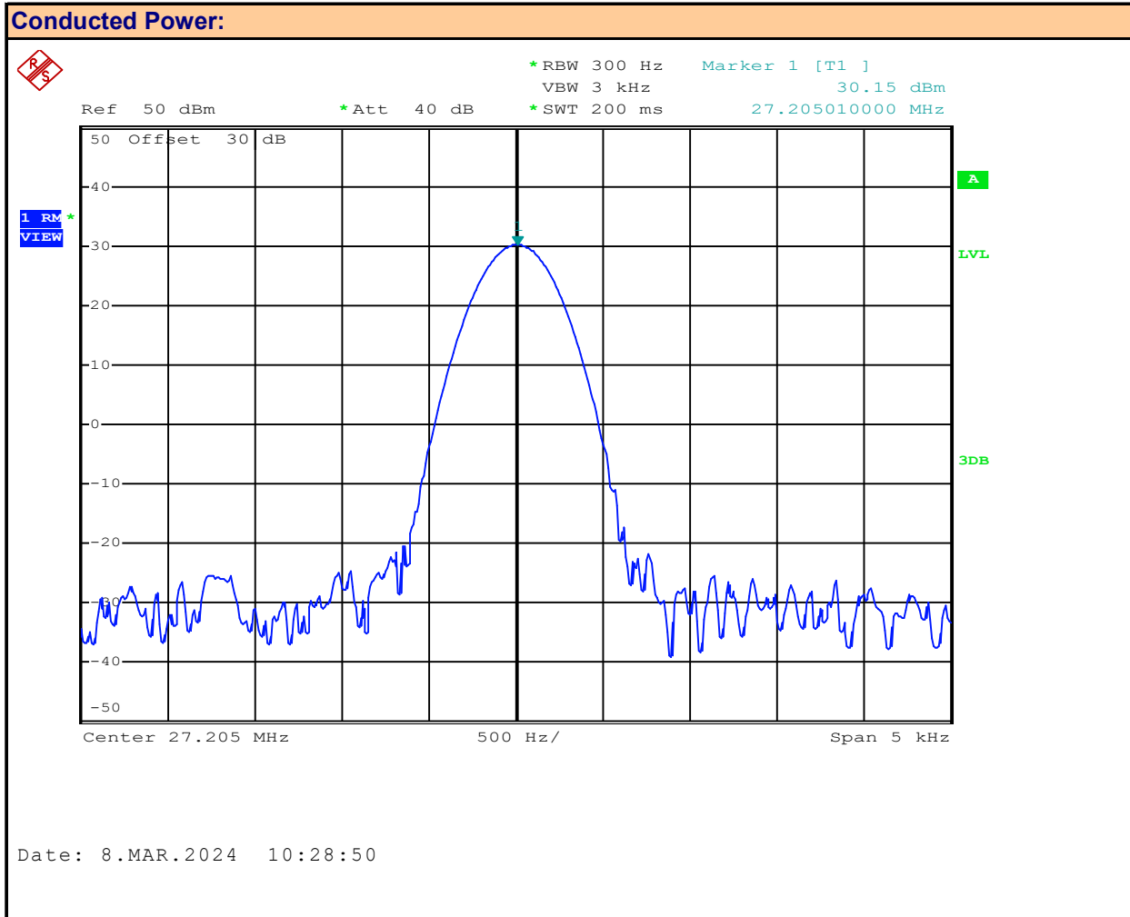
Plot 7.14 – Conducted Output Power, Channel 20, AM, 1W
