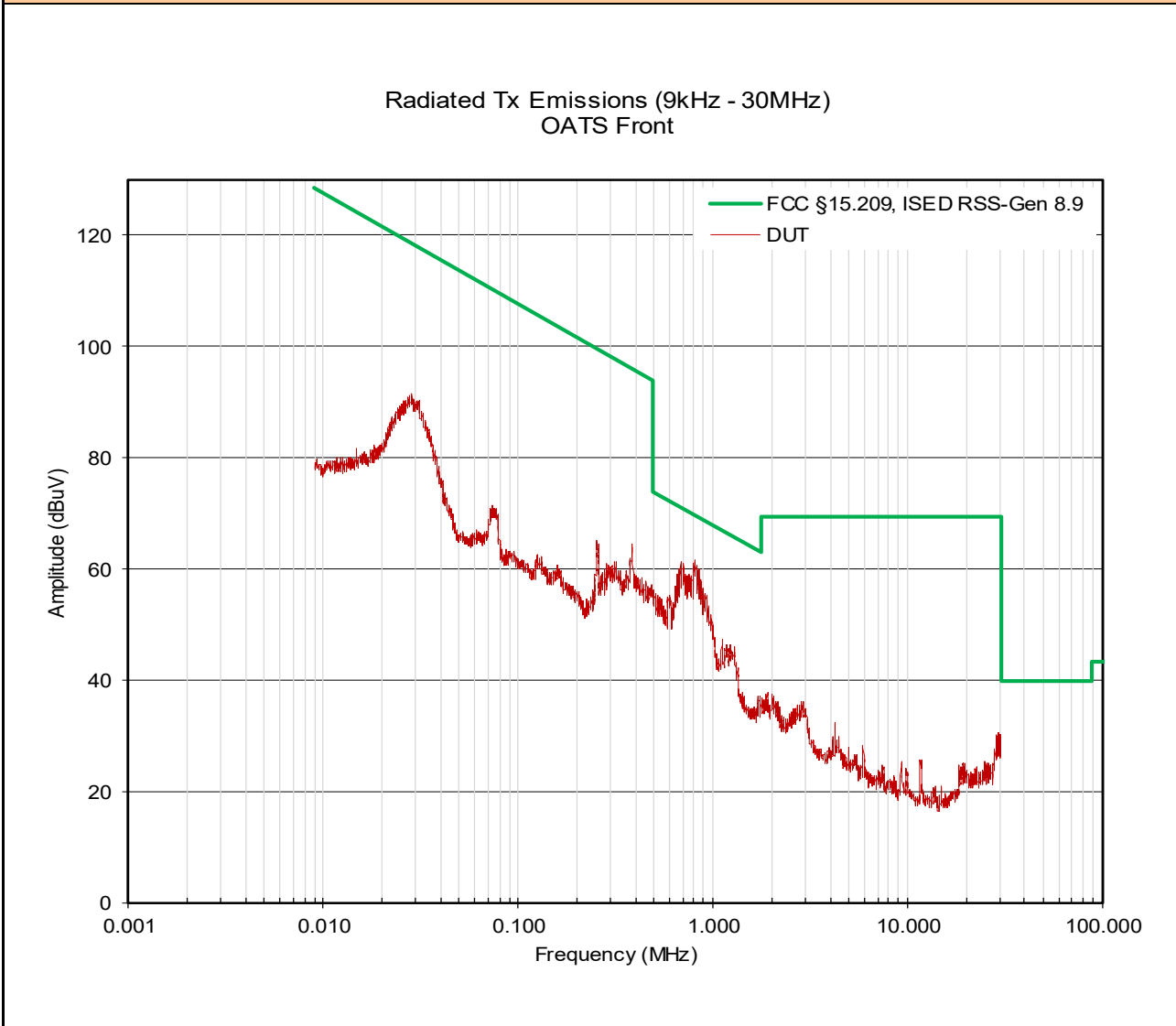
Plot 11.1 – Radiated Spurious Emissions OATS, 9kHz - 30MHz, without Accessories, Front
