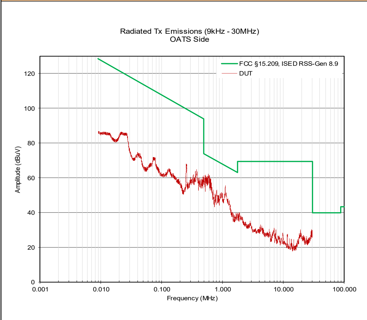
Plot 11.2 – Radiated Spurious Emissions OATS, 9kHz - 30MHz, without Accessories, Side
