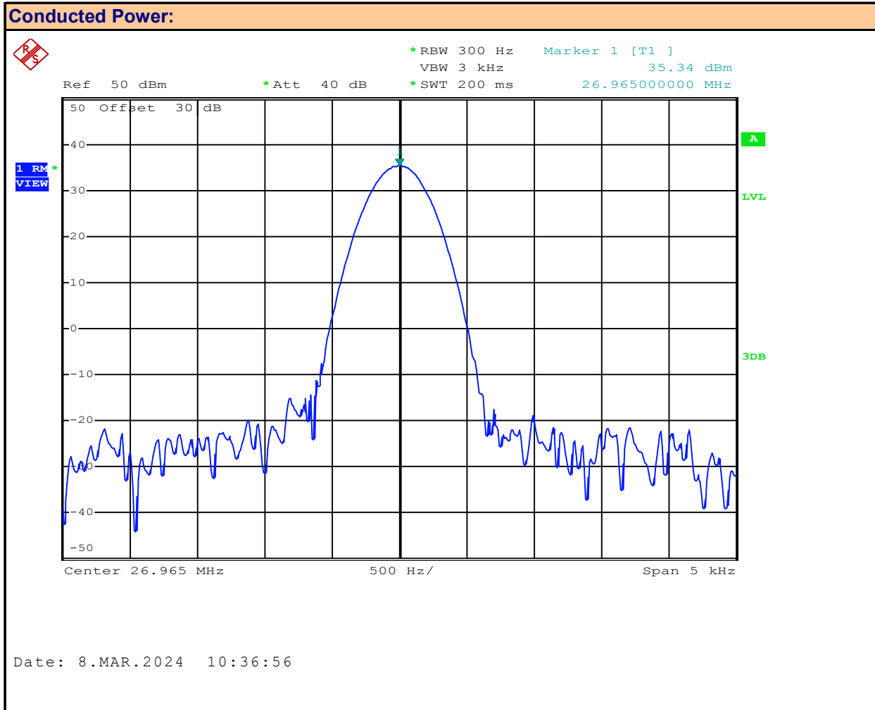
Plot 7.7 – Conducted Output Power, Channel 1, AM, 4W, External
