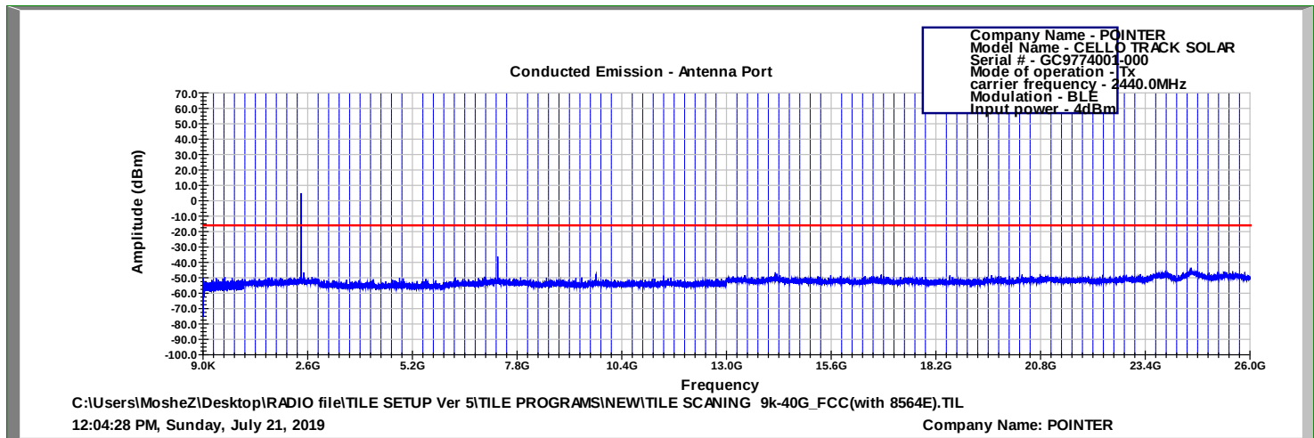
Figure 36 2440.0 MHz, BLE
