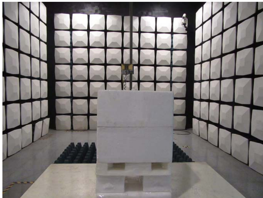
Radiated Disturbance Test Setup View (Above 1GHz)
