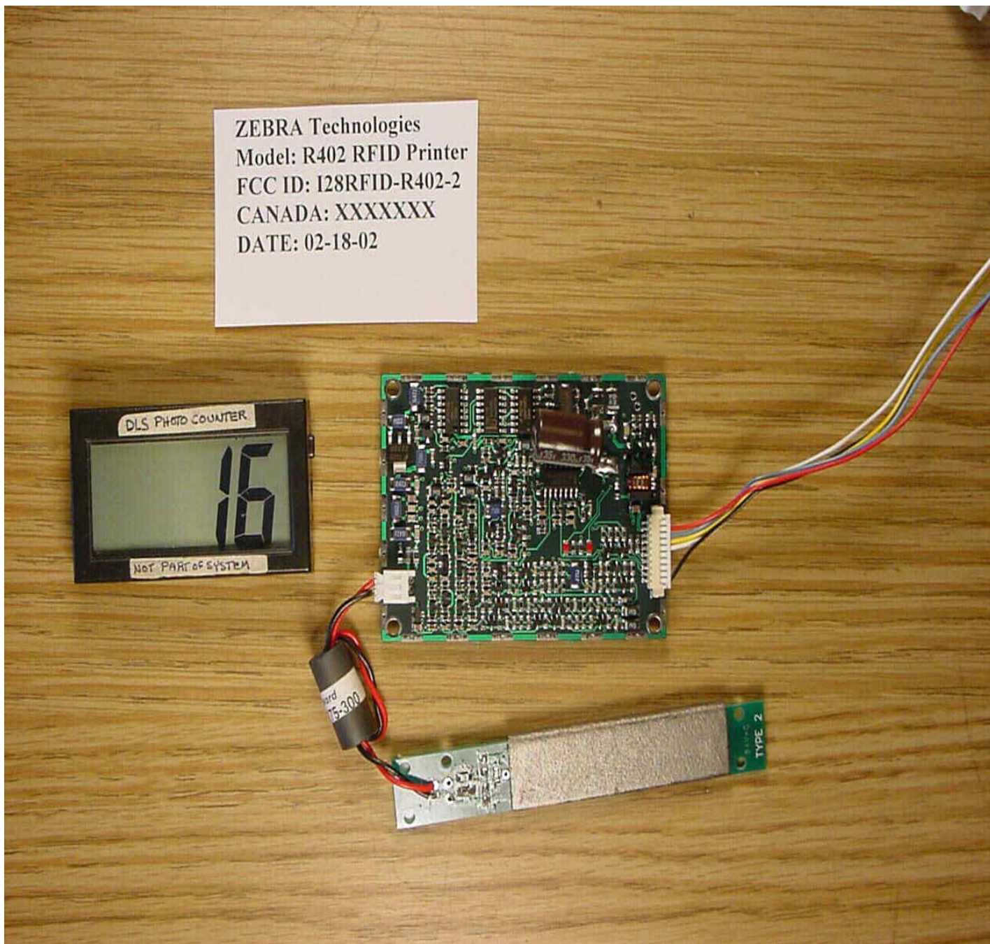
RFID Transmitter Board #102212 V1.2 and Antenna Board #52336 Rev A Together
