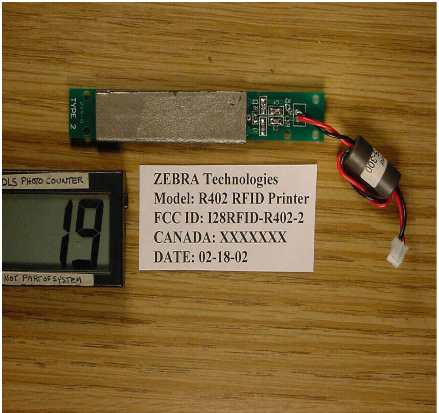
Antenna Board #52336 Rev A (Antenna Side)
