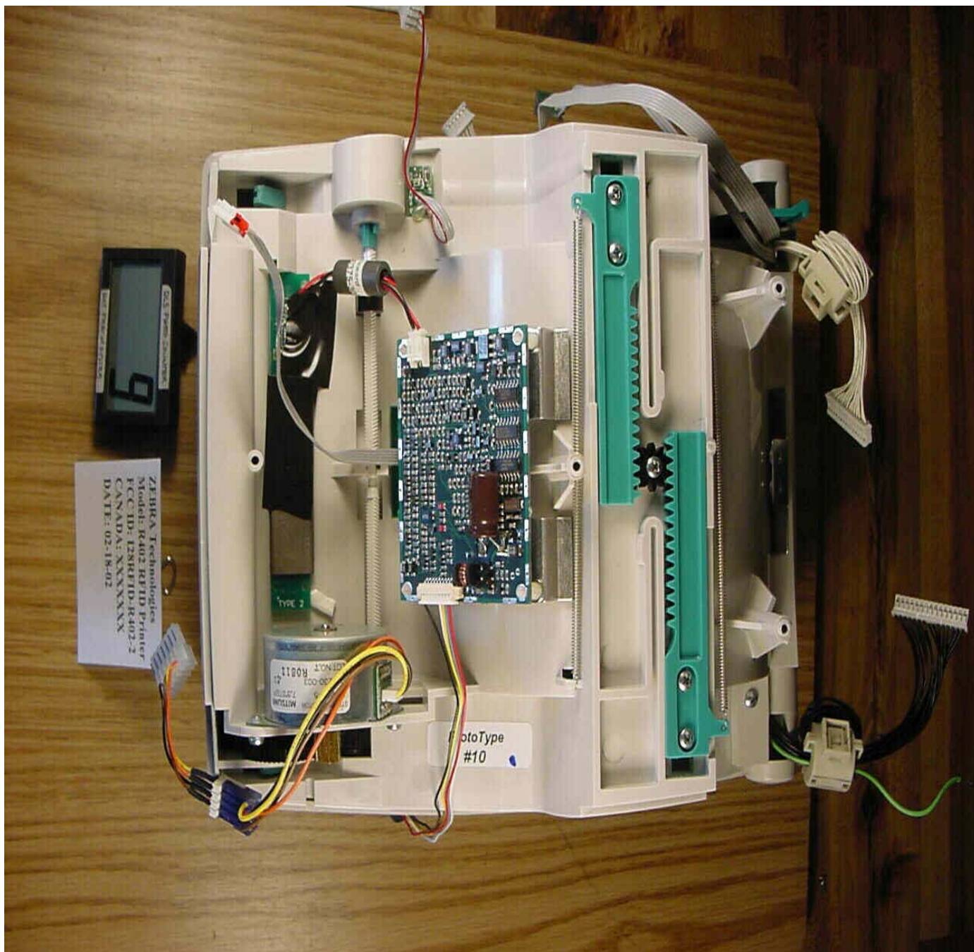
Inside Bottom Cover
