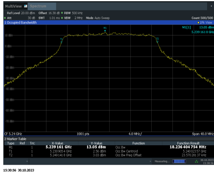
Fig.68 99% Occupied bandwidth (802.11ac-VHT20, 5240MHz)
