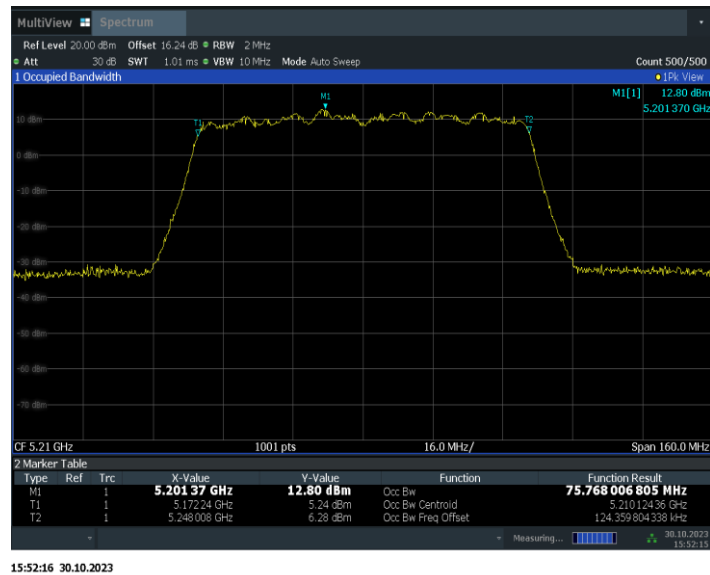
Fig.73 99% Occupied bandwidth (802.11ac-VHT80, 5210MHz)
