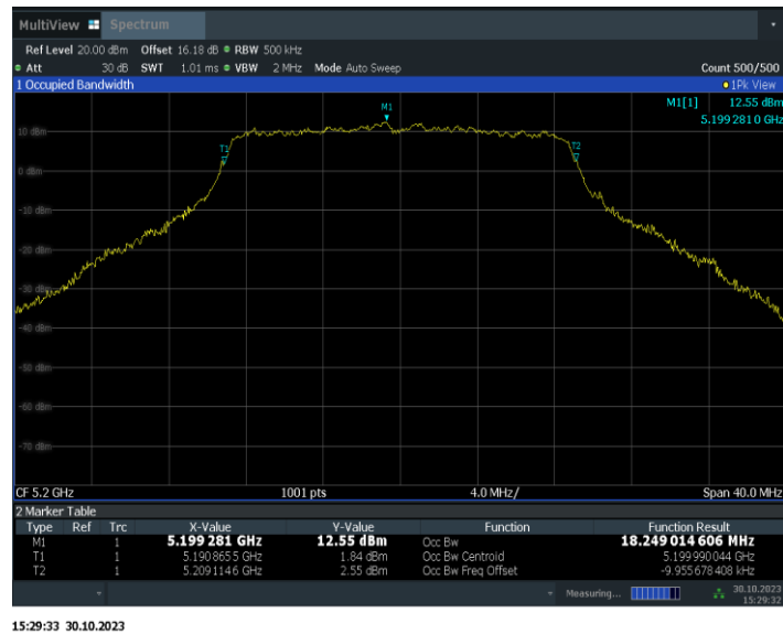
Fig.67 99% Occupied bandwidth (802.11ac-VHT20, 5200MHz)
