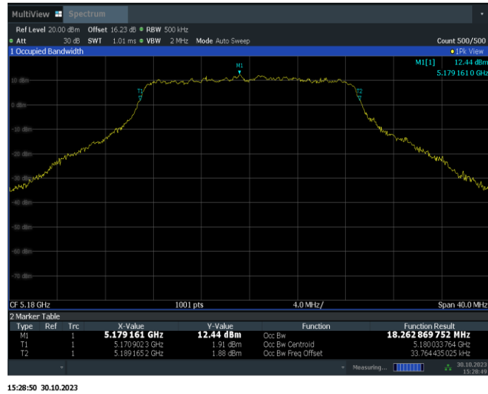
Fig.66 99% Occupied bandwidth (802.11ac-VHT20, 5180MHz)
