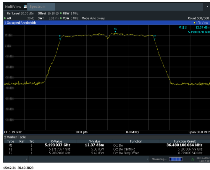
Fig.71 99% Occupied bandwidth (802.11ac-VHT40, 5190MHz)
