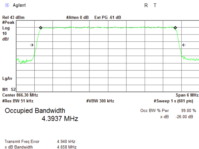
Plot 7.2.3 Occupied bandwidth test result, 64QAM, ant.0
