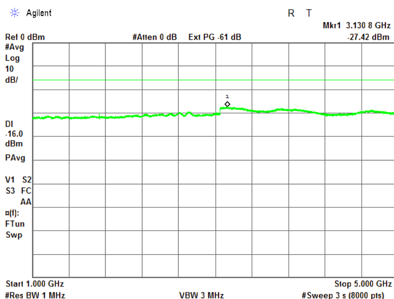
Plot 7.5.6 Spurious emission measurements in 1000 - 5000 MHz at ant.0
