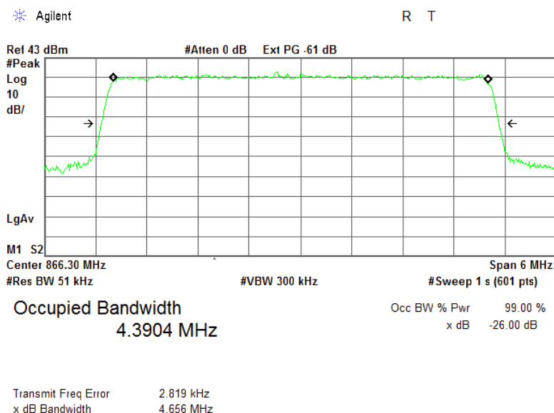
Plot 7.2.4 Occupied bandwidth test result, 64QAM, ant.1
