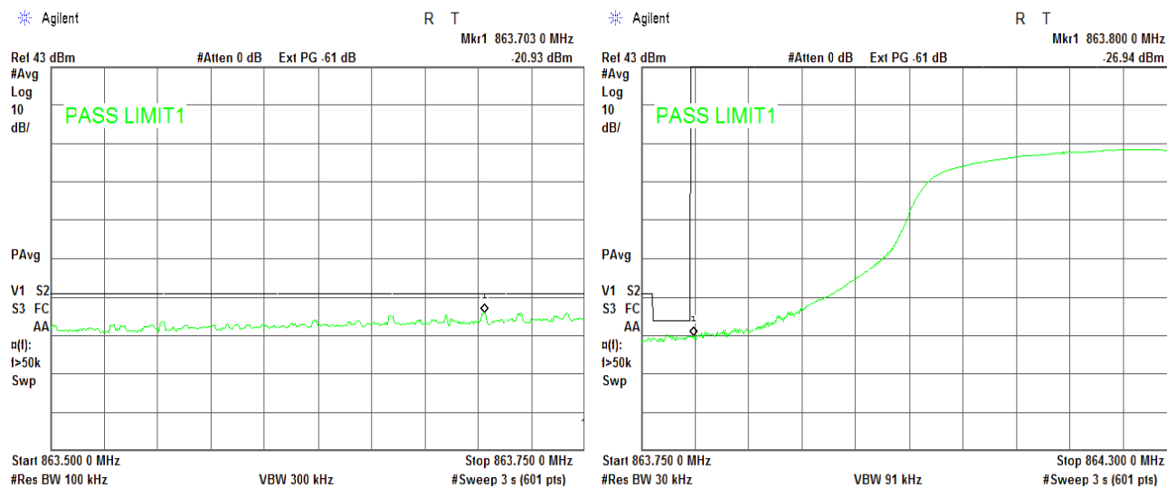
Plot 7.3.2 Emission mask test s results, QPSK, ant. 0 (continued)
