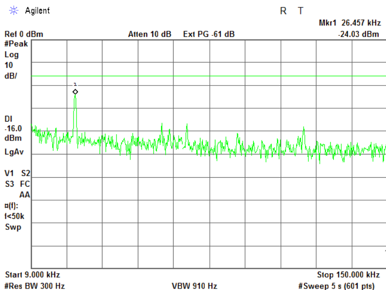
Plot 7.5.1 Spurious emission measurements in 9 - 150 kHz range at ant.0
