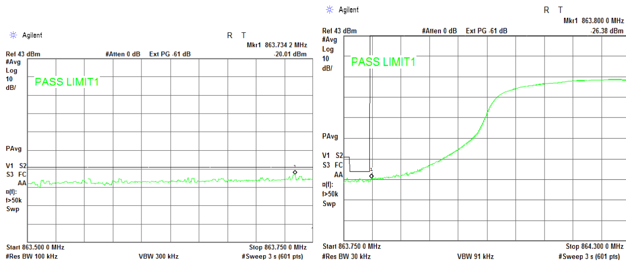
Plot 7.3.1 Emission mask test results, 64QAM, ant. 0 (continued)
