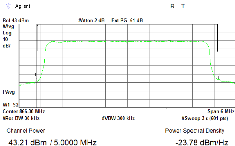
Plot 7.1.1 Peak output power test results, 64QAM, ant.0
