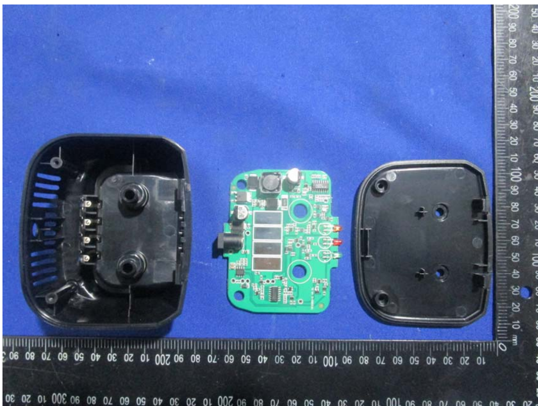
Charger Base
