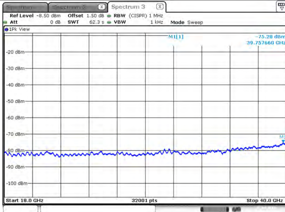
Plot on Configuration VHT20 / 5700 MHz / Average / Port 4 / 18GHz~40GHz
