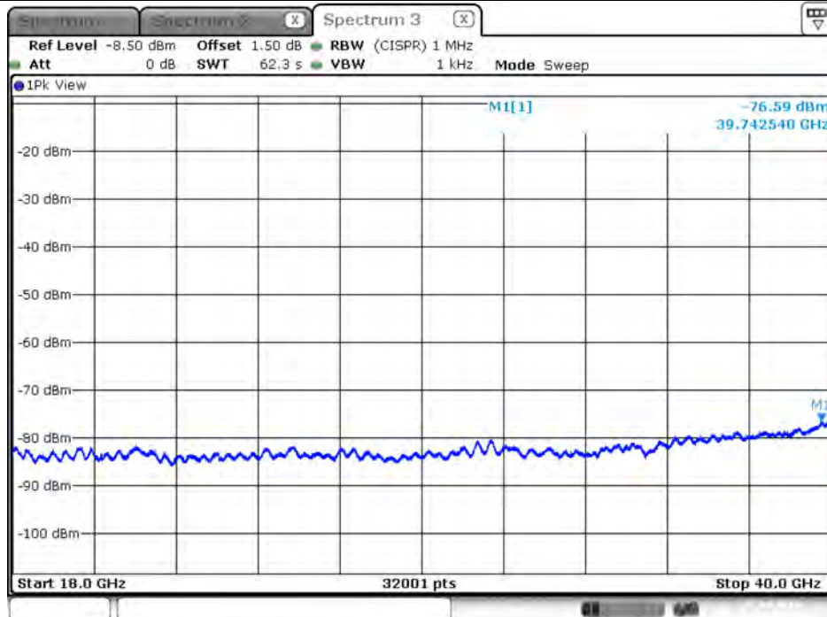
Plot on Configuration VHT40 / 5550 MHz / Average / Port 2 / 18GHz~40GHz
