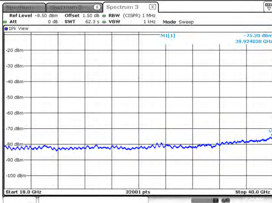
Plot on Configuration VHT20 / 5700 MHz / Average / Port 3 / 18GHz~40GHz
