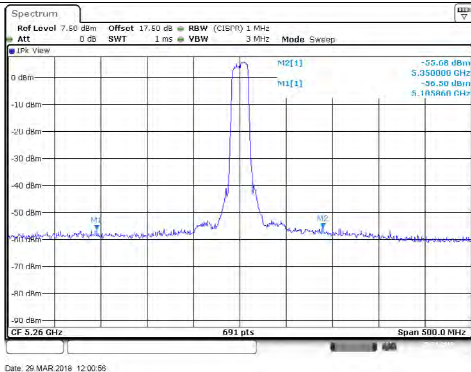
Plot on Configuration VHT20 / 5260 MHz / Peak / Port 4
