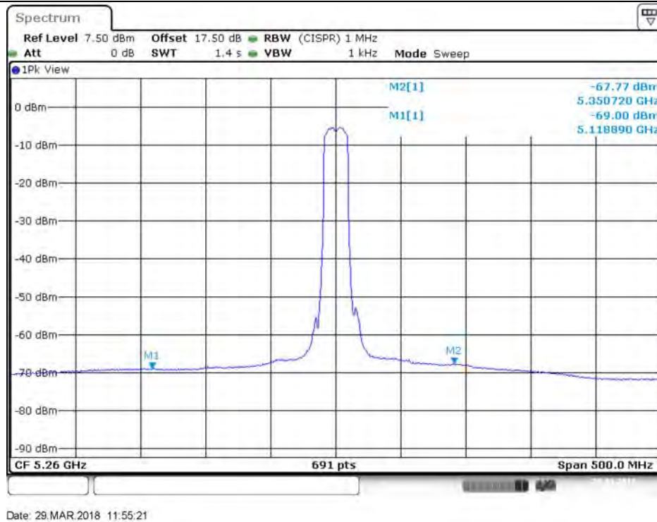
Plot on Configuration VHT20 / 5260 MHz / Average / Port 2
