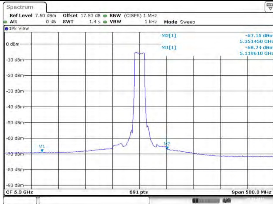
Plot on Configuration VHT20 / 5300 MHz / Average / Port 3
