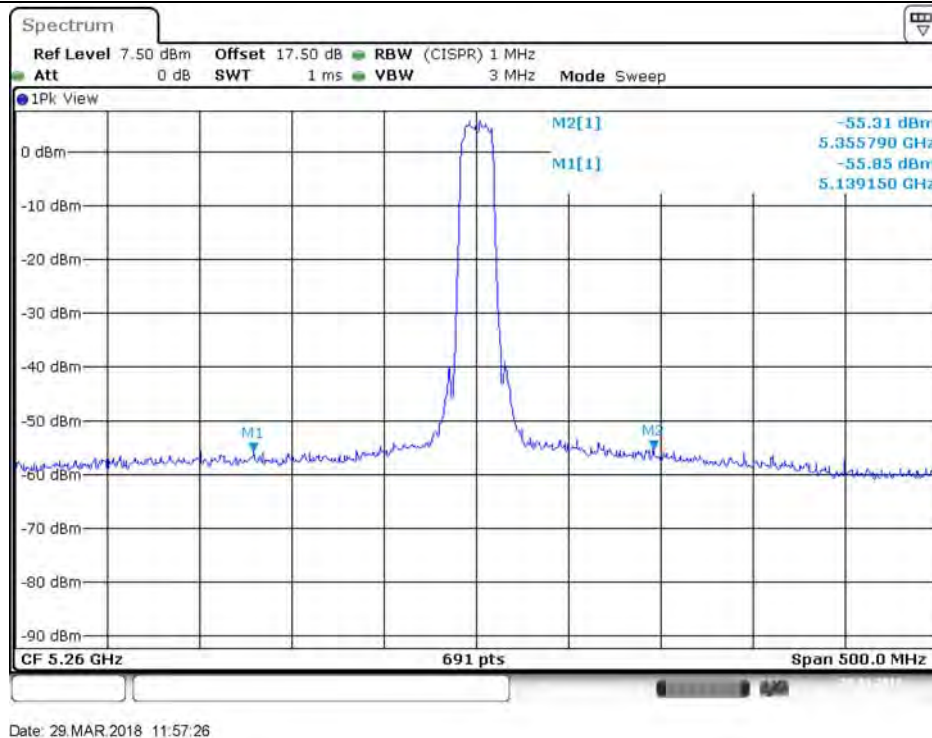
Plot on Configuration VHT20 / 5260 MHz / Peak / Port 2
