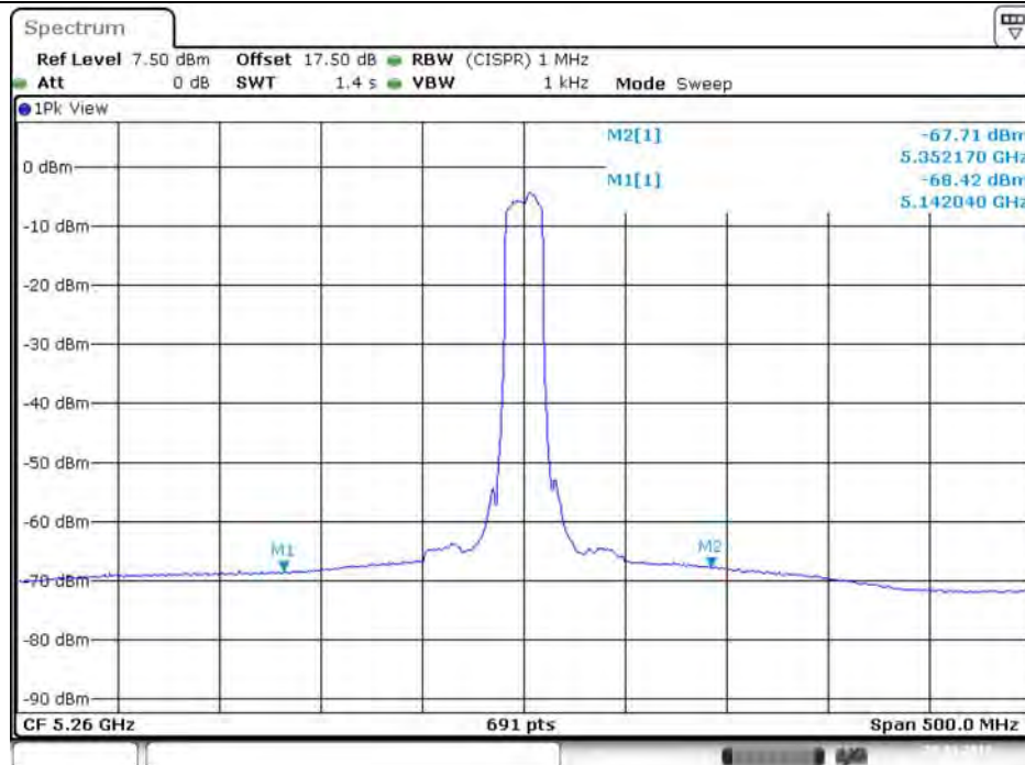
Plot on Configuration VHT20 / 5260 MHz / Average / Port 4
