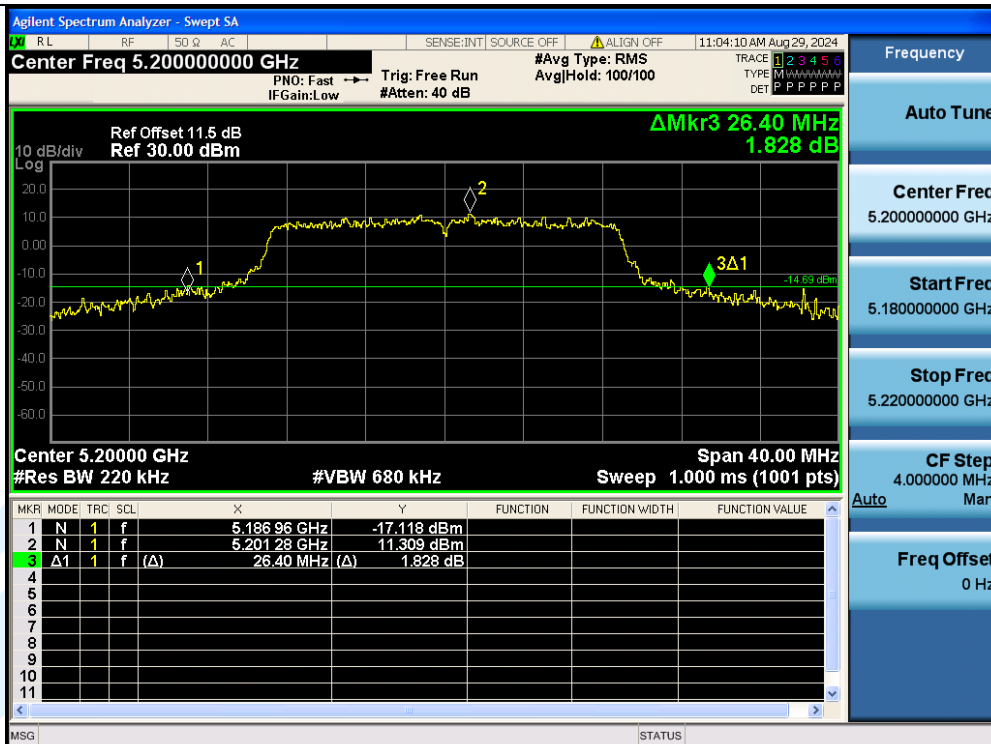
11AC20MIMO-Ant3-5200
