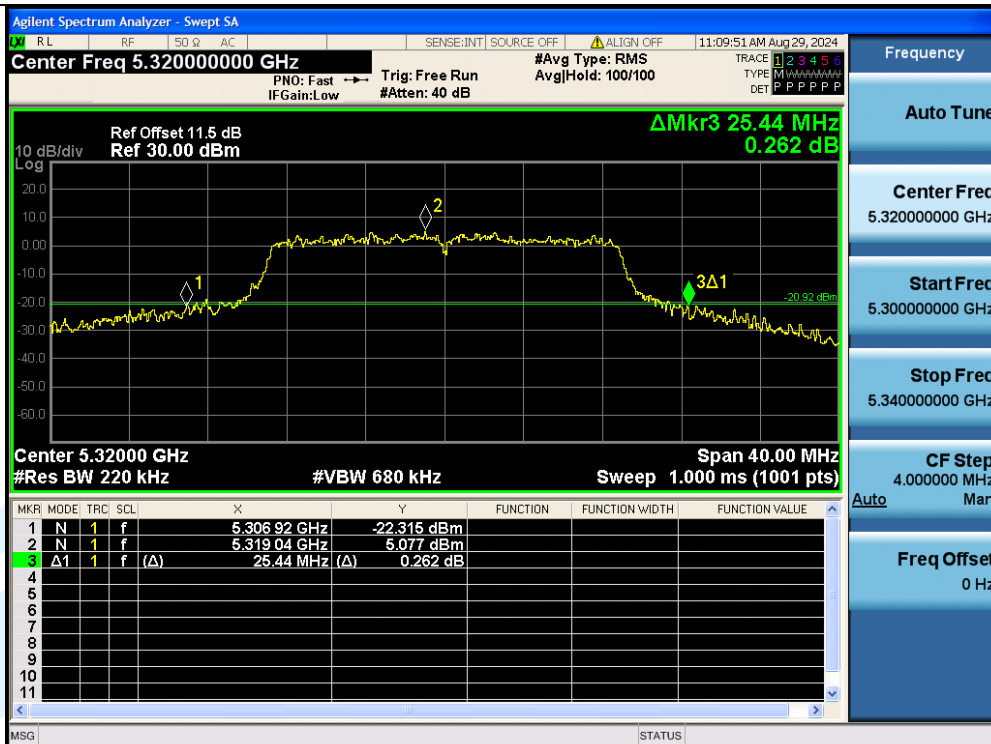
11AC20MIMO-Ant3-5320
