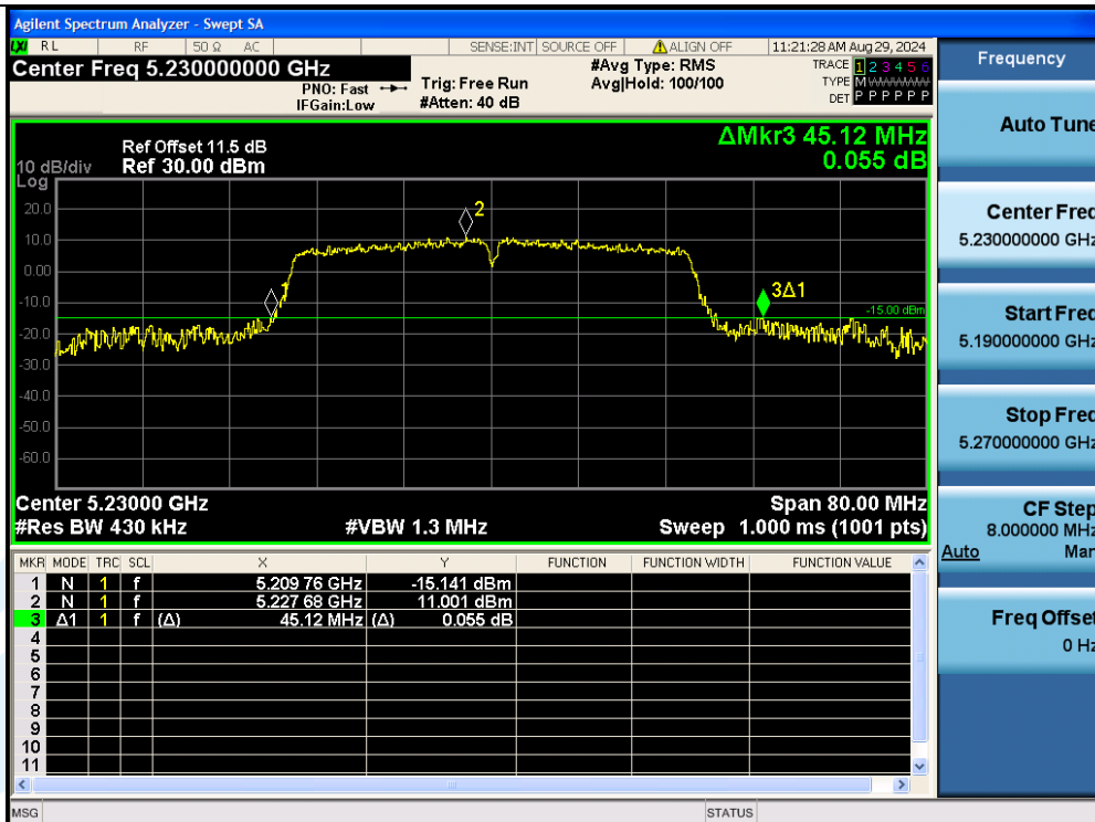
11AC40MIMO-Ant3-5230
