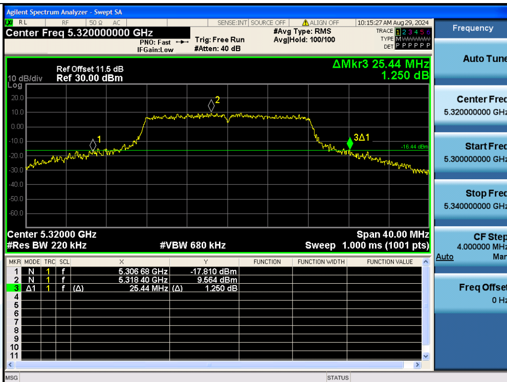
11A-Ant3-5320
