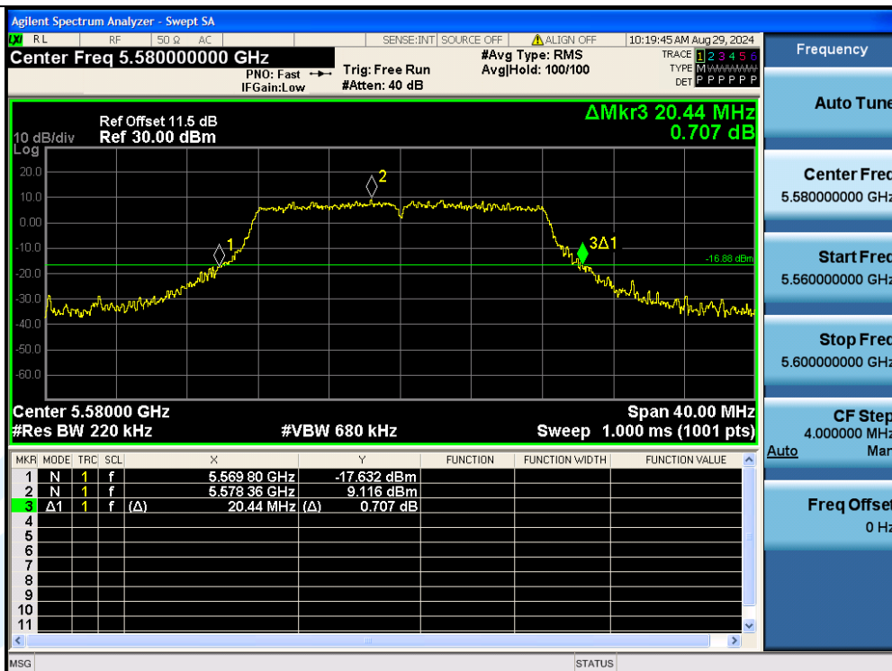
11A-Ant3-5580
