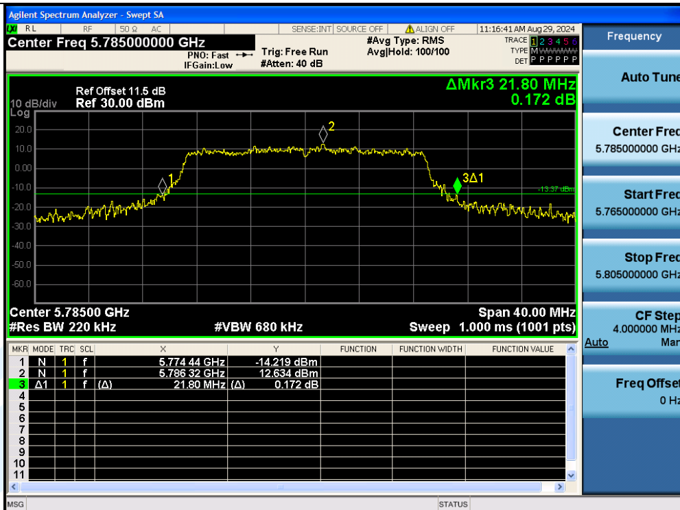
11AC20MIMO-Ant3-5785
