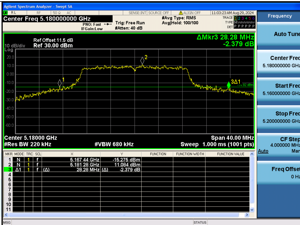
11AC20MIMO-Ant3-5180
