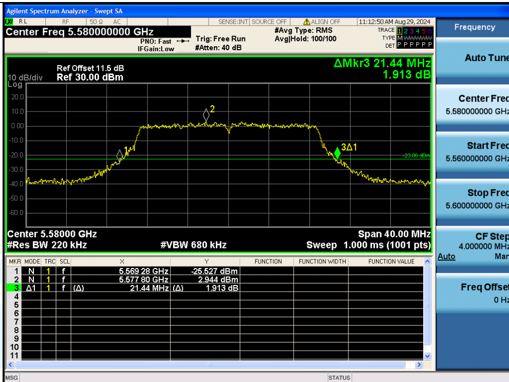
11AC20MIMO-Ant3-5580
