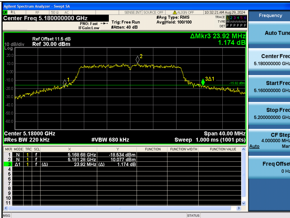
11N20MIMO-Ant3-5180
