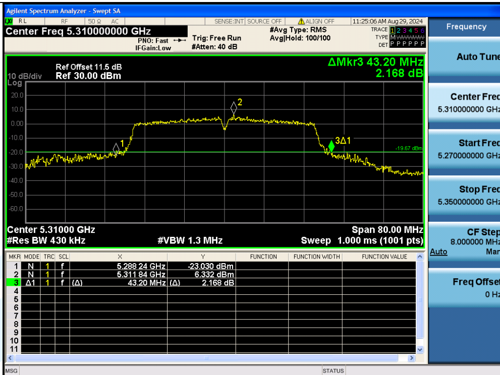
11AC40MIMO-Ant3-5310
