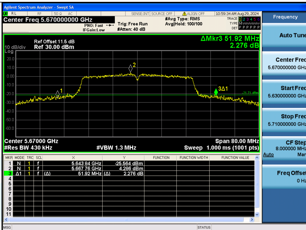
11N40MIMO-Ant3-5670
