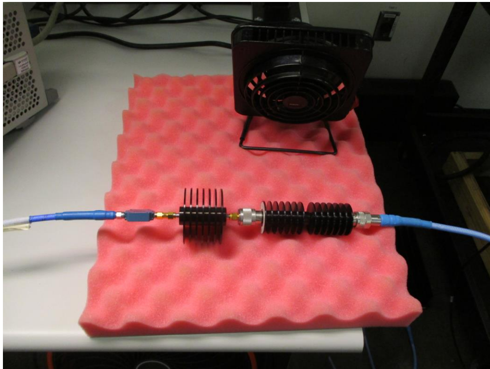
RF Configuration 4, 13 GHz to 27 GHz
