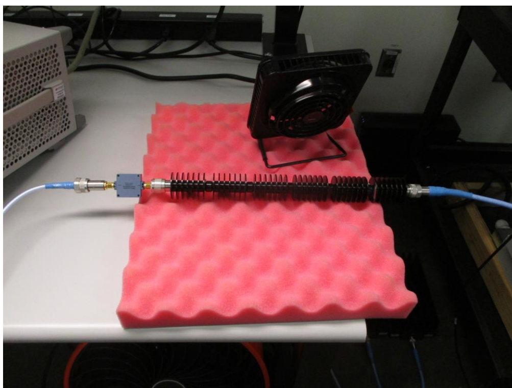
RF Configuration 3, 3.5 GHz to 13 GHz
