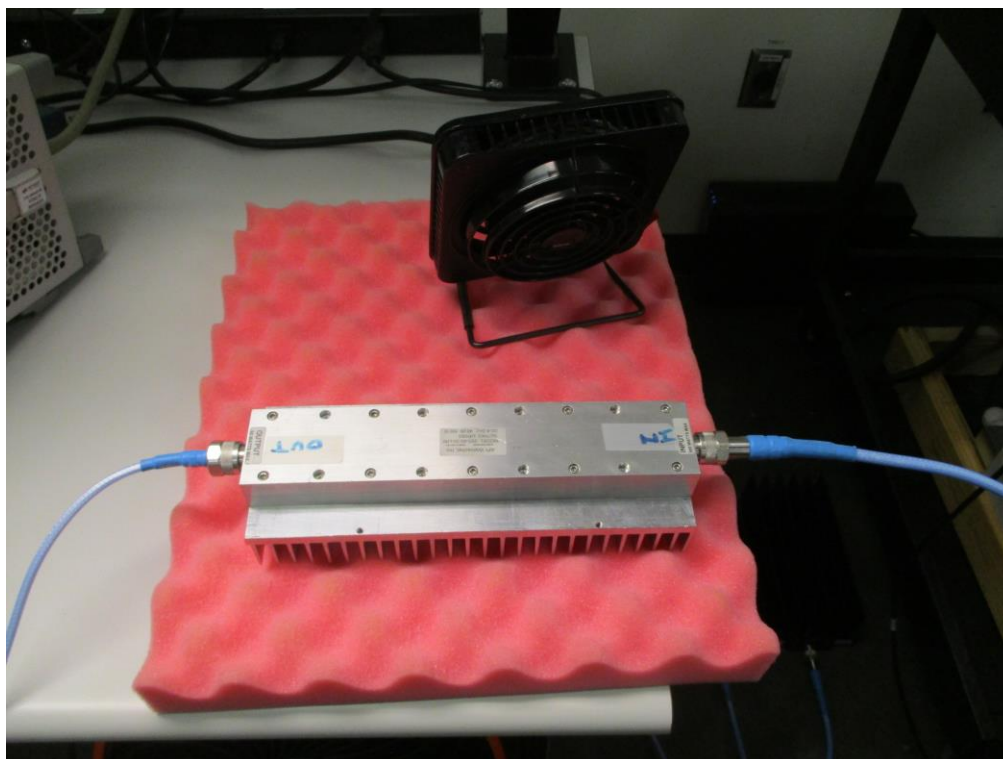
RF Configuration 2, 20 MHz to 3.5 GHz
