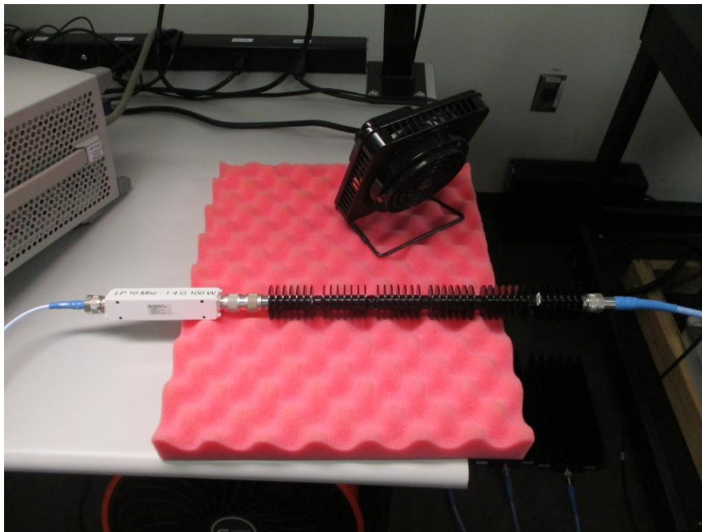
RF Configuration 1, 9 kHz to 20 MHz
