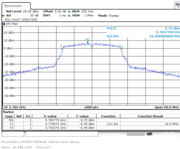
802.11a_5785MHz_Chain 1
