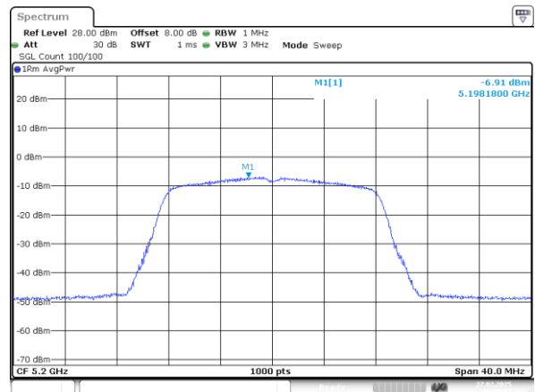
802.11a_5200MHz_Chain 0
