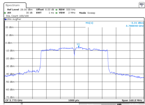
802.11ac80_5775MHz_Chain 1
