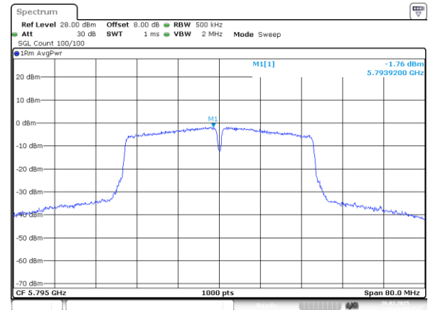
802.11n40_5795MHz_Chain 0
