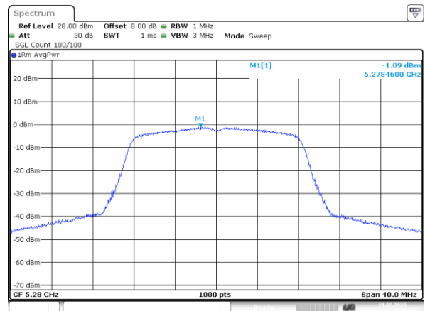
802.11a_5280MHz_Chain 0
