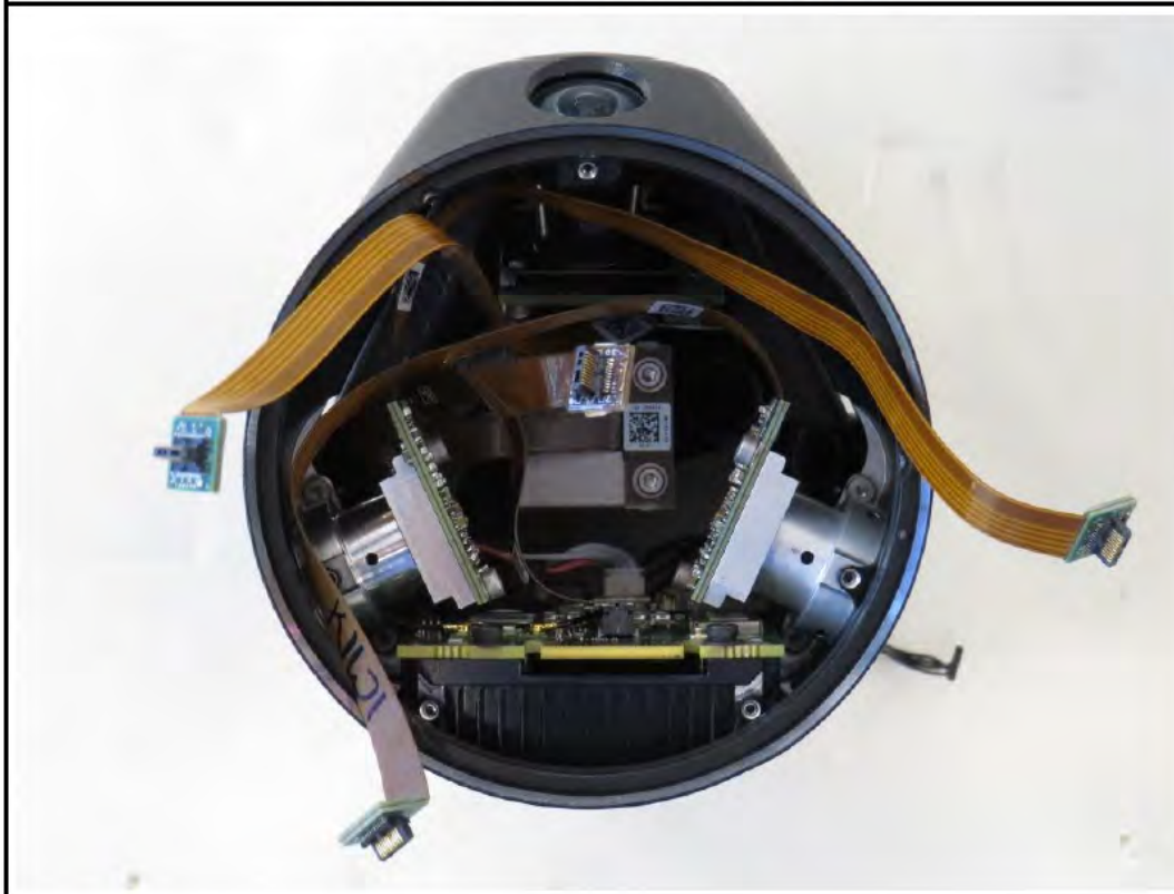
TOP VIEW WITHOUT DOME COVER
