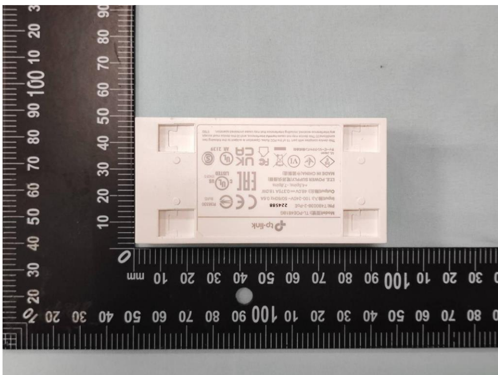
(12) EUT Photo (Brand: tp-link,M/N: TL-POE4818G)
