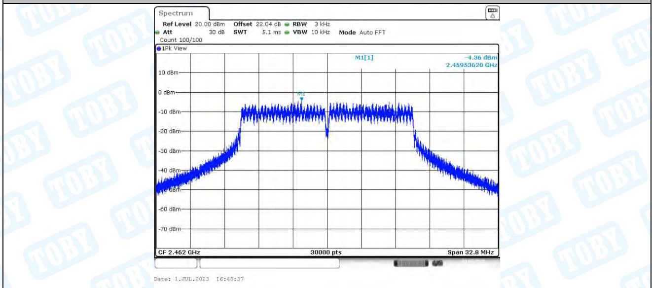
11G_Ant4_2462
