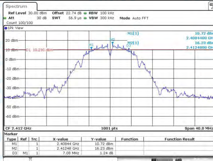
11B_Ant3_2412
