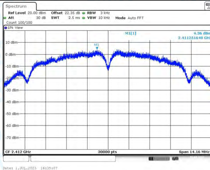
11B_Ant3_2412
