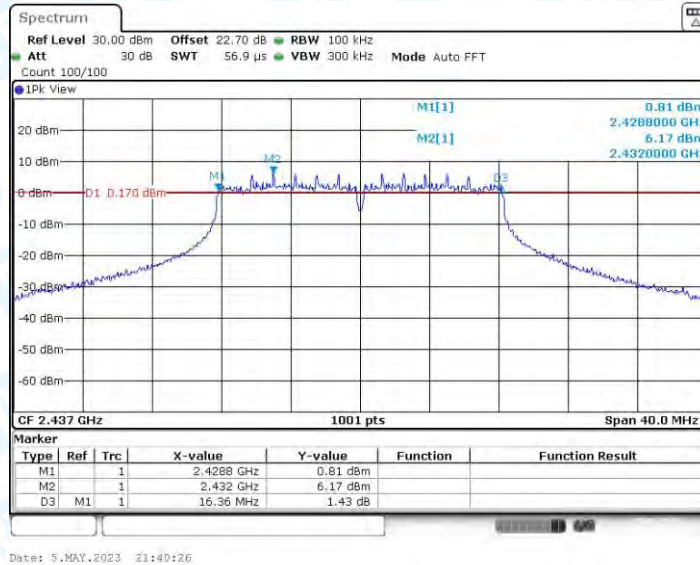
11G_Ant4_2437
