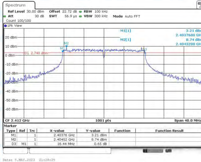
11G_Ant3_2412
