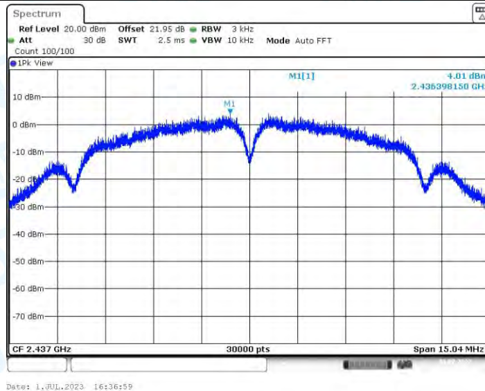
11B_Ant3_2437
