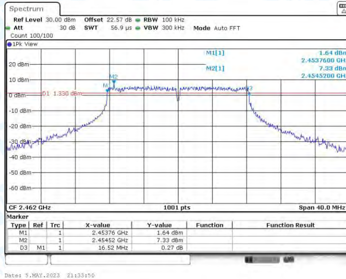
11G_Ant3_2462
