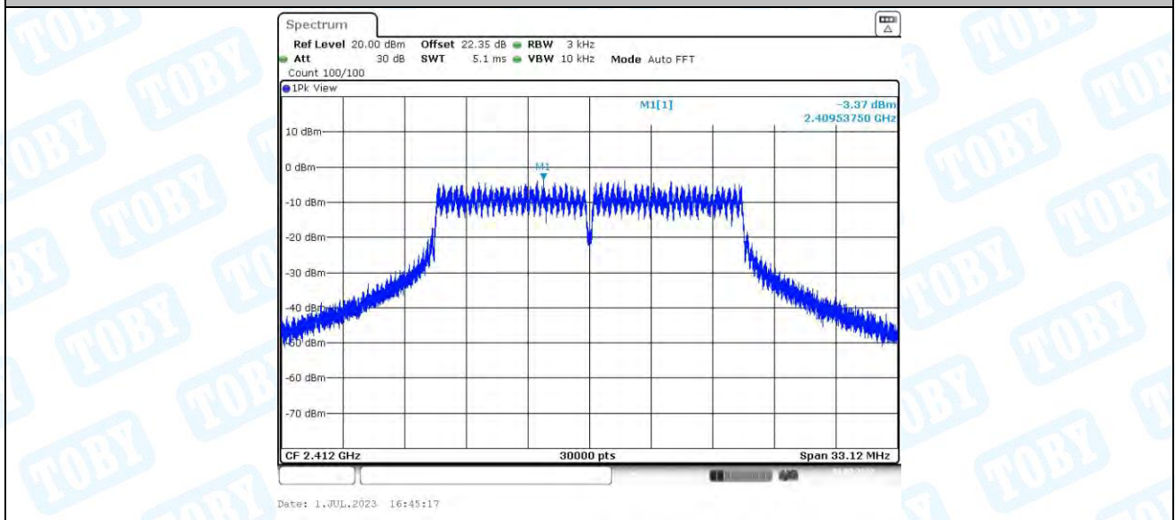
11G_Ant4_2412
