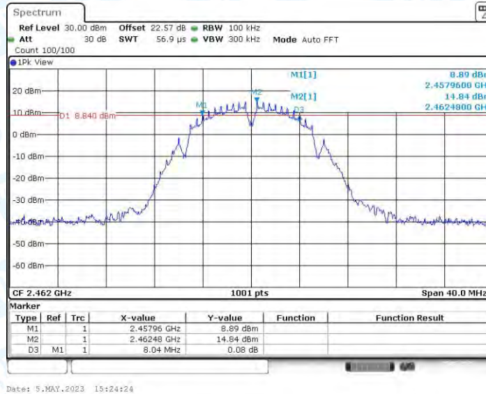
11B_Ant3_2462
