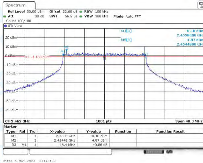
11G_Ant4_2462
