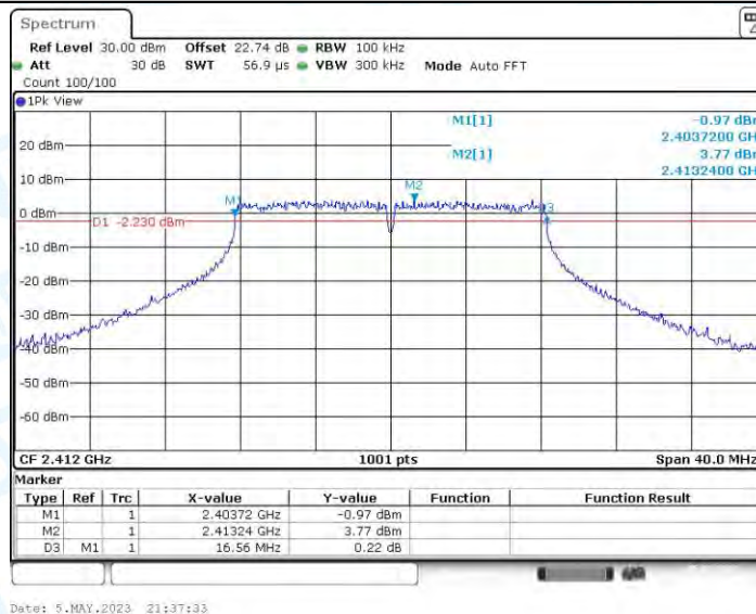
11G_Ant4_2412
