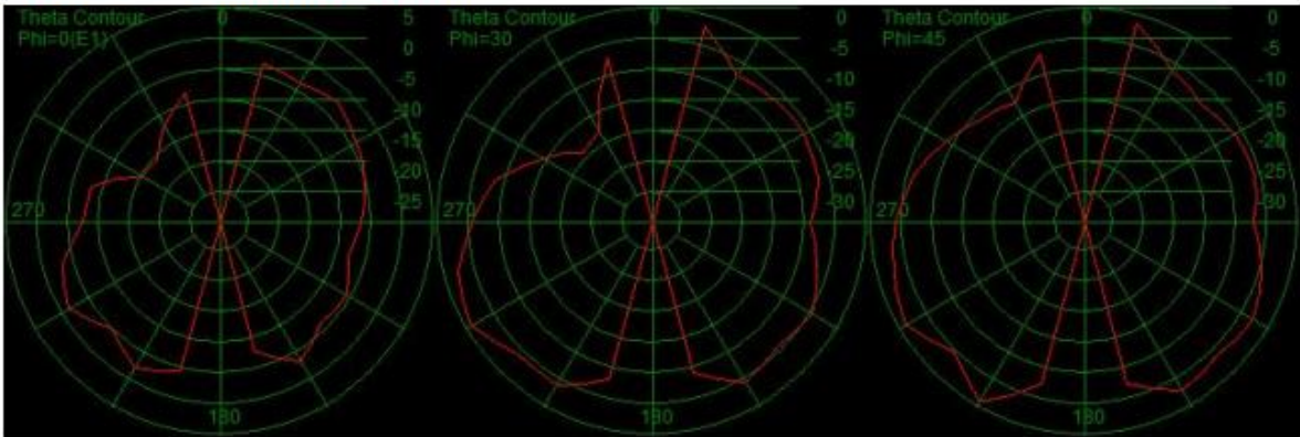
WIFI 2.4G Antenna 2D Pattern
