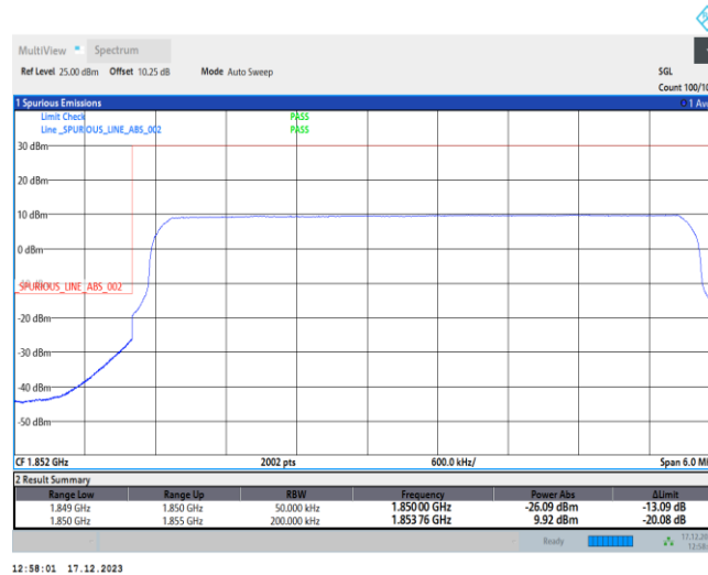
1-N2-PC3-15-5-L-3-DFT-PI2BPSK-Outer_Full-25@0-Ant0-1-seegraph-PASS-see graph
