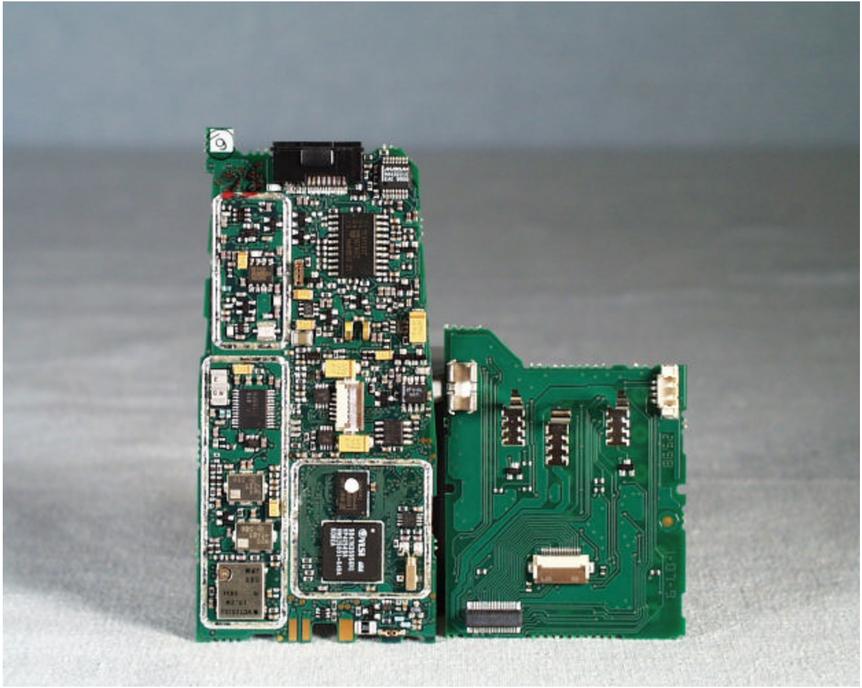
Component side of the interface board (Without RF Cans)
