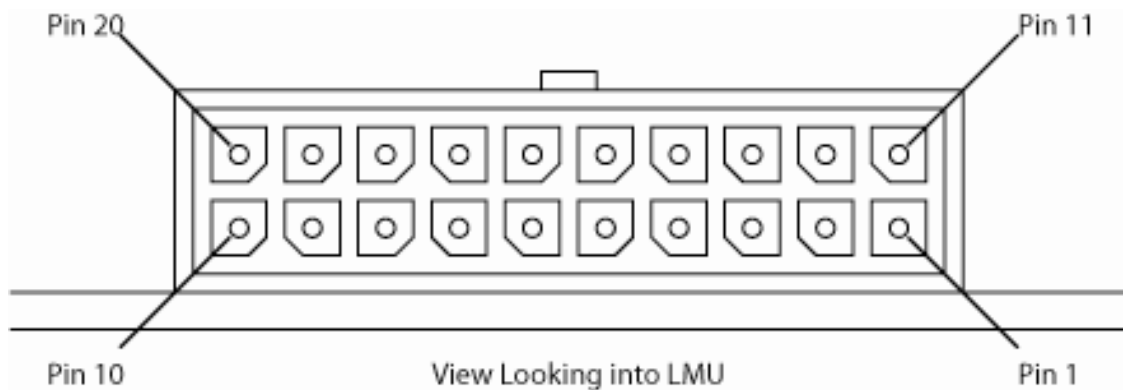
Figure 2 - LMU-2640™ Header
