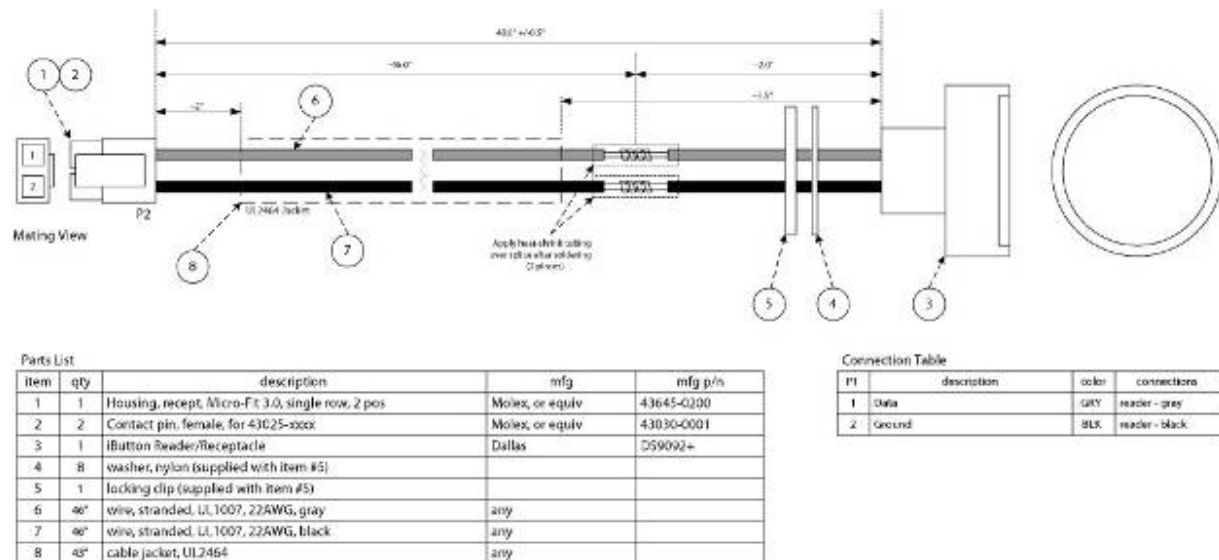
Figure 9 - iButton Reader and Cable Assembly
