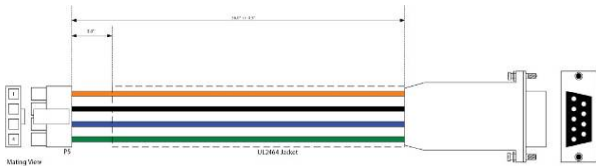
Figure 7 - LMU-2640™ Serial Adapter
