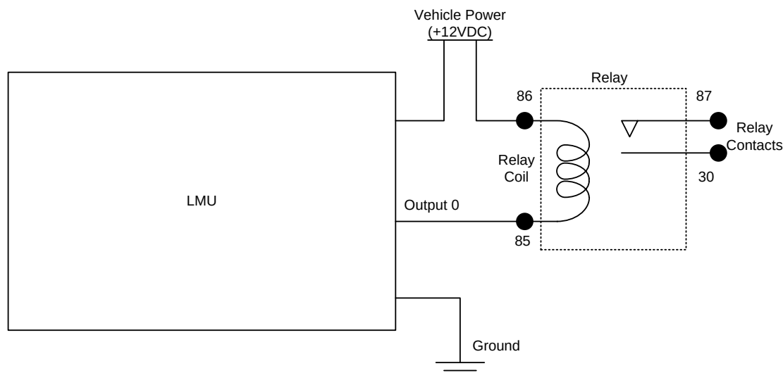
Figure 22 - Sample Relay Wiring
