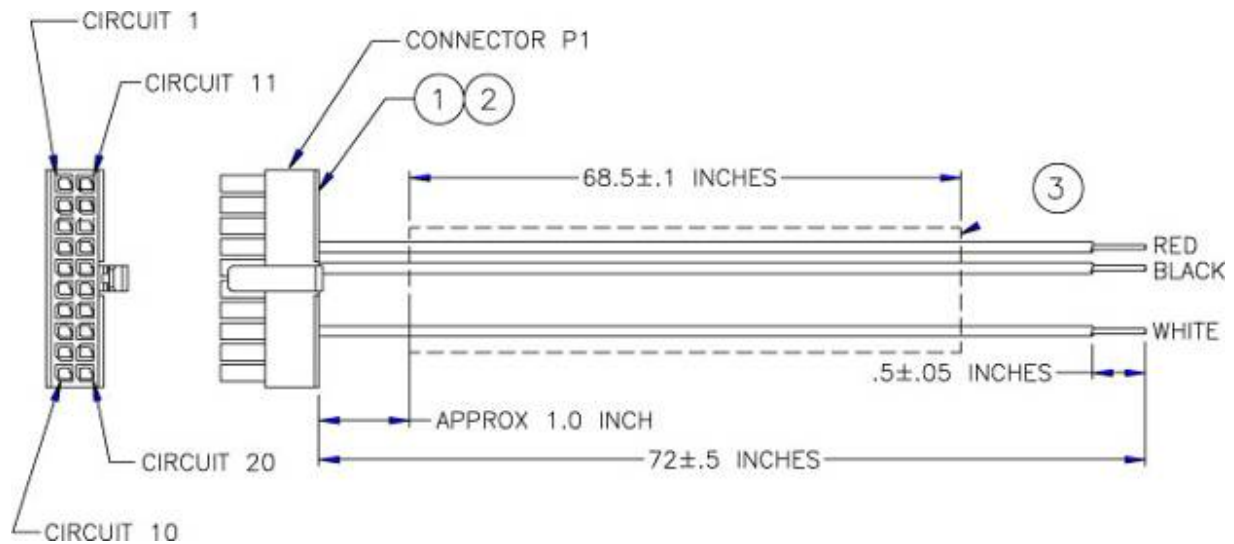
Figure 3 - Basic 3-Wire Power Harness - unfused
