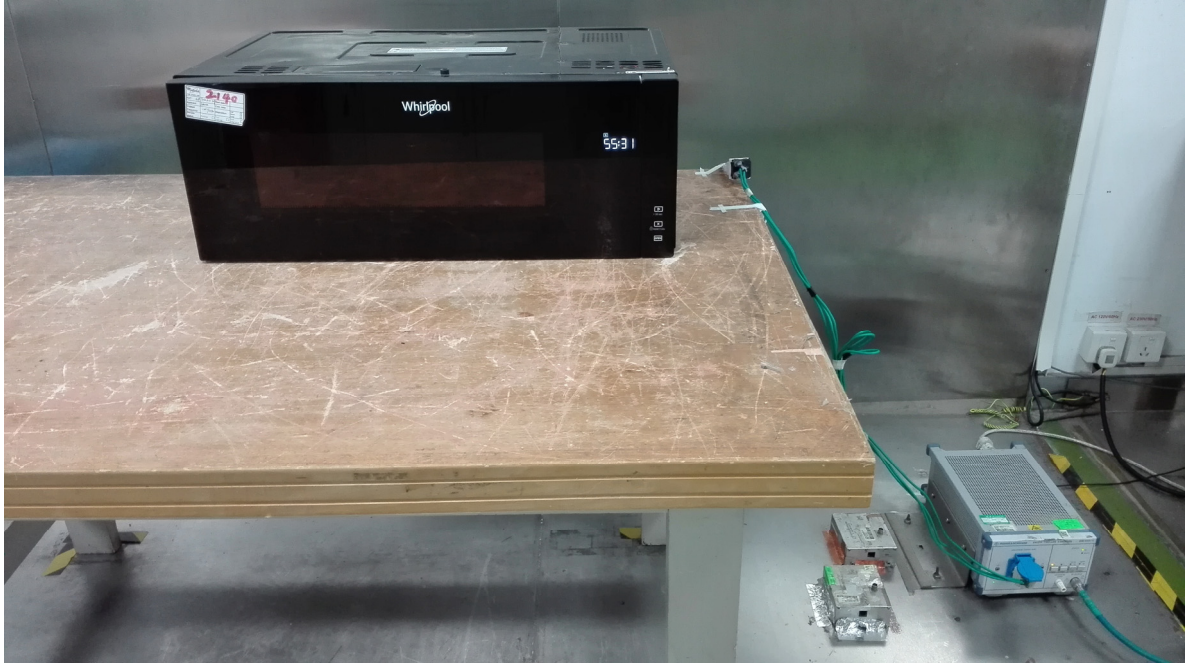
Conducted Emissions - Front View
