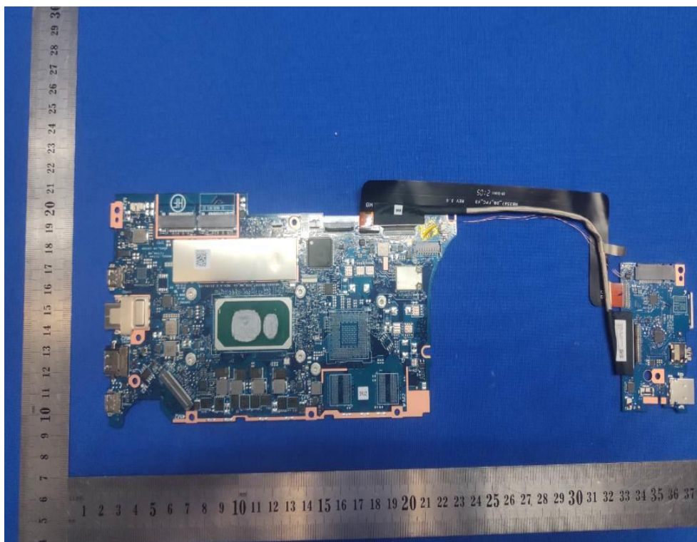
PWB view
