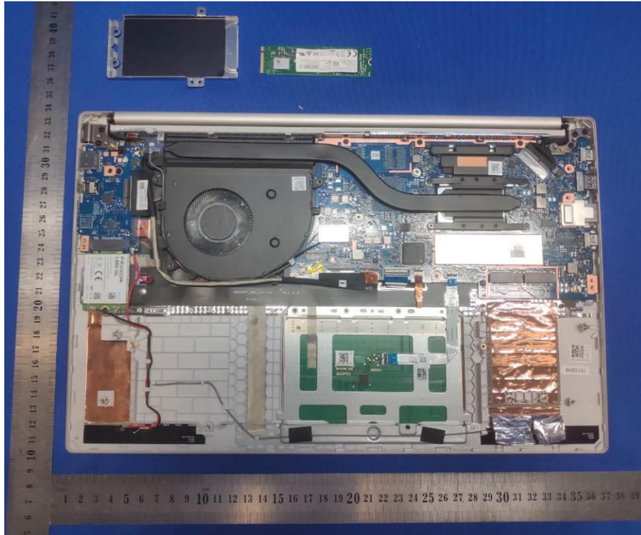
Internal view
