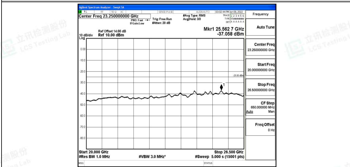
Band7-20MHz-16QAM-21350-1RB#0-Range6:20000~26500MHz
