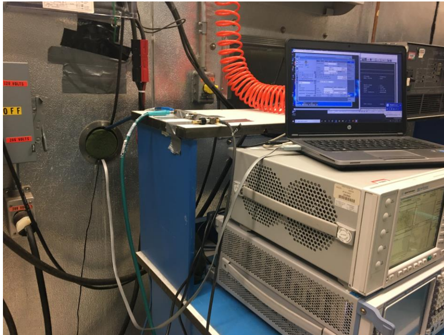
Frequency Stability (Inside the Thermal Chamber)
