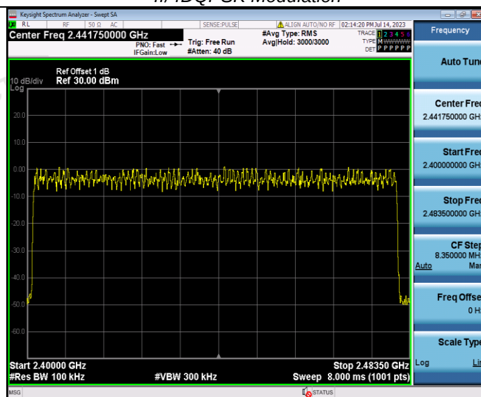
8DPSK Modulation
