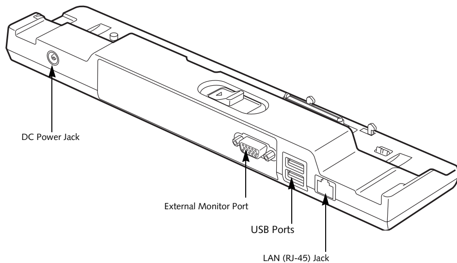
Figure 4-7. Port Replicator rear panel
