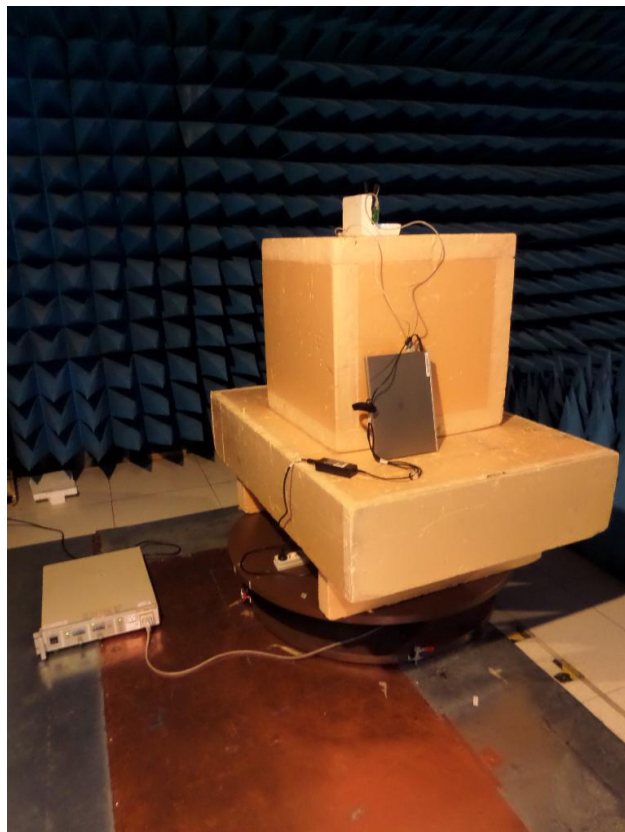
Radiated setup (anechoic chamber)
