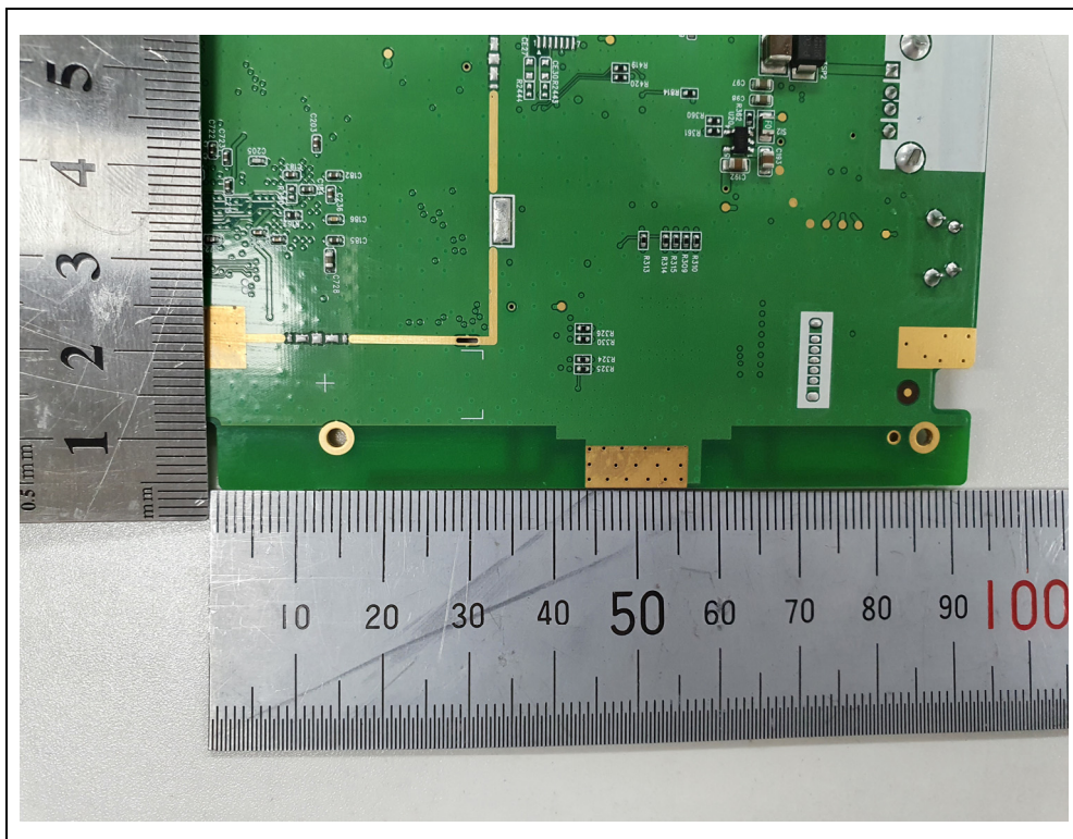
<Antenna _ Back>
