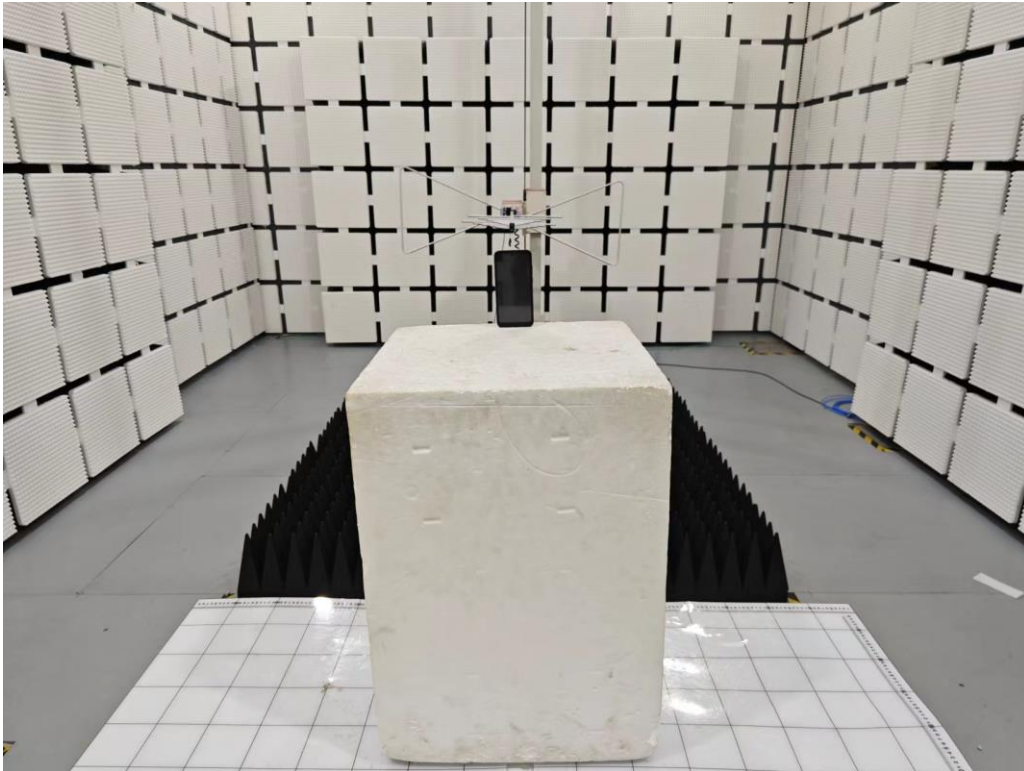
Set-up for Transmitter Spurious Emissions, Below 1GHz
