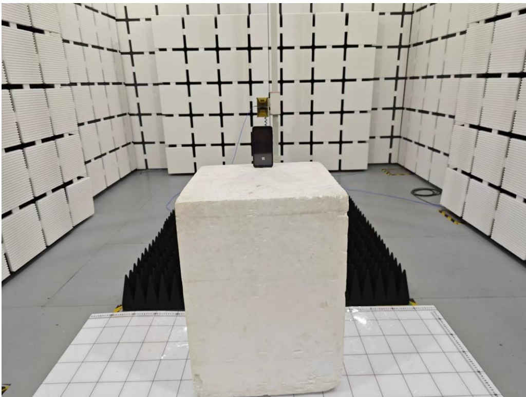
Set-up for Transmitter Spurious Emissions, Above 1GHz
