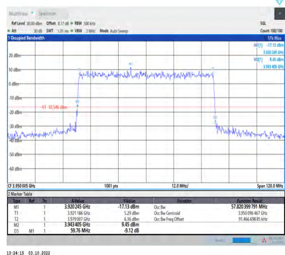
1-N77-3700-3980--30-60-H-6-CP-QPSK-Outer_Full- 162@0-Ant1-57.82-59.760-≤60-PASS
