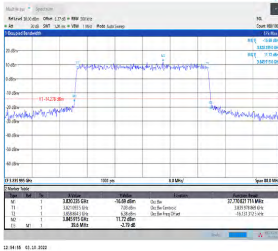
1-N77-3700-3980--30-40-M-6-CP-QPSK-Outer_Full-106@0-Ant1-37.771-39.600-≤40-PASS
