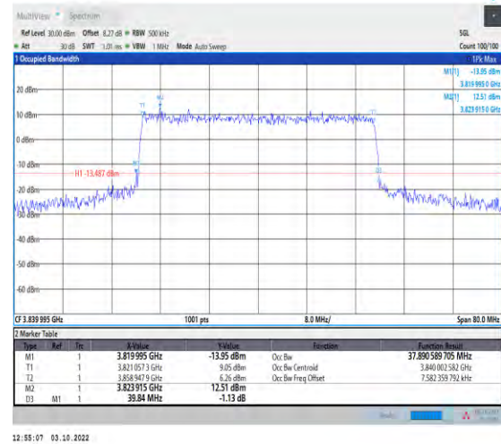
1-N77-3700-3980--30-40-M-7-CP-16QAM-Outer_Ful I-106@0-Ant1-37.891-39.840-≤40-PASS
