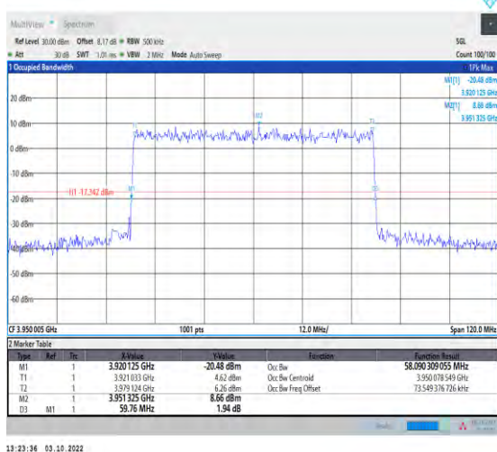
1-N77-3700-3980--30-60-H-5-DFT-256QAM-Outer_F ull-162@0-Ant1-58.09-59.760-≤60-PASS
