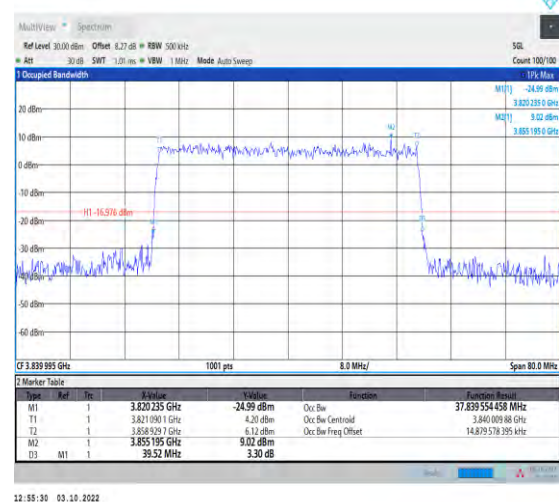
1-N77-3700-3980--30-40-M-9-CP-256QAM-Outer_Full-106@0-Ant1-37.84-39.520-≤40-PASS
