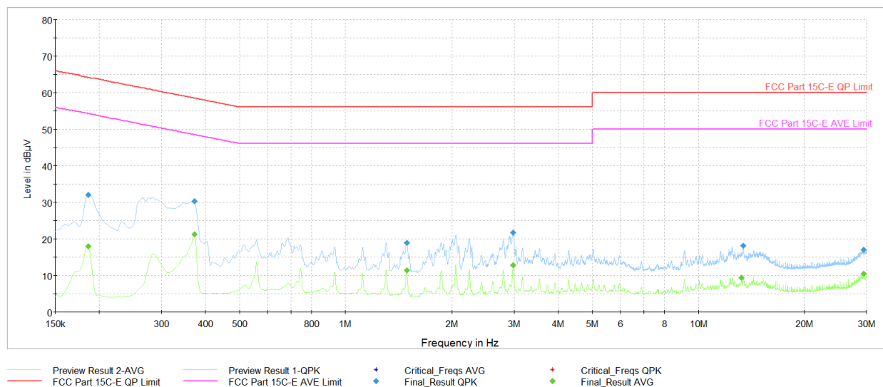
Plot 7-131. AC Line Conducted Plot (NB UNII HDR4 – 5201MHz) (N) with Laptop and USB-C Cable
