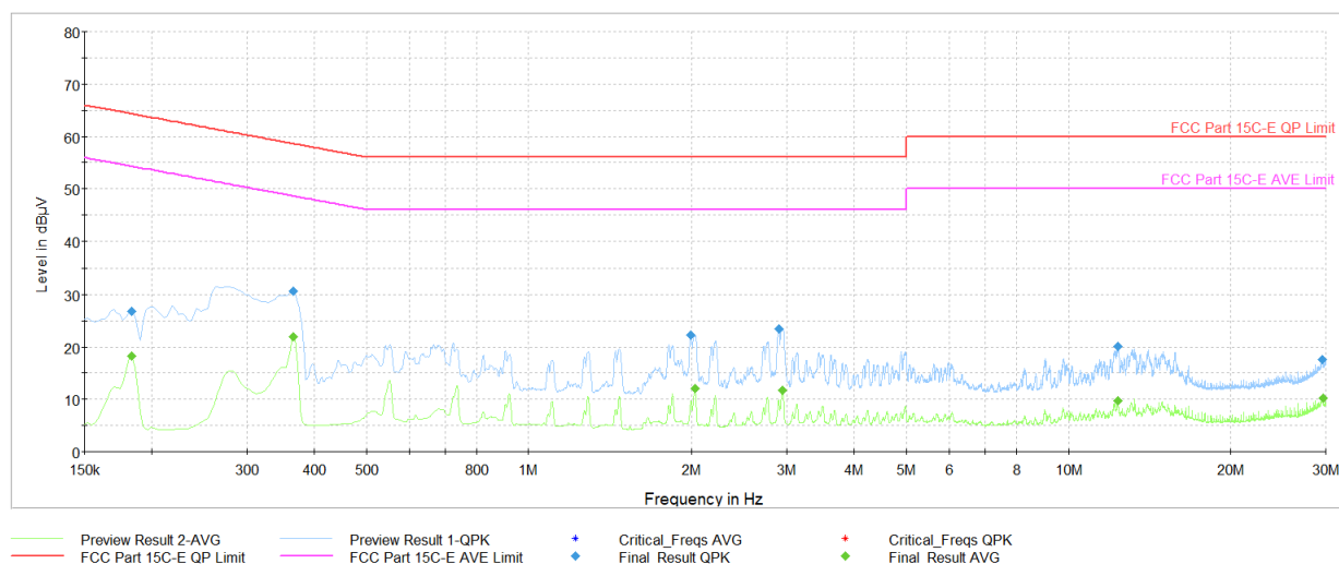
Plot 7-133. AC Line Conducted Plot (NB UNII HDRp4 – 5245MHz) (N) with AC/DC Adapter and USB-C Cable
