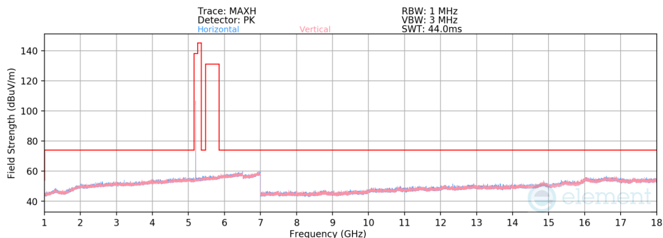
Plot 7-86. Radiated Spurious Emissions 1-18GHz (NB UNII HDRp4 – 5201MHz)
