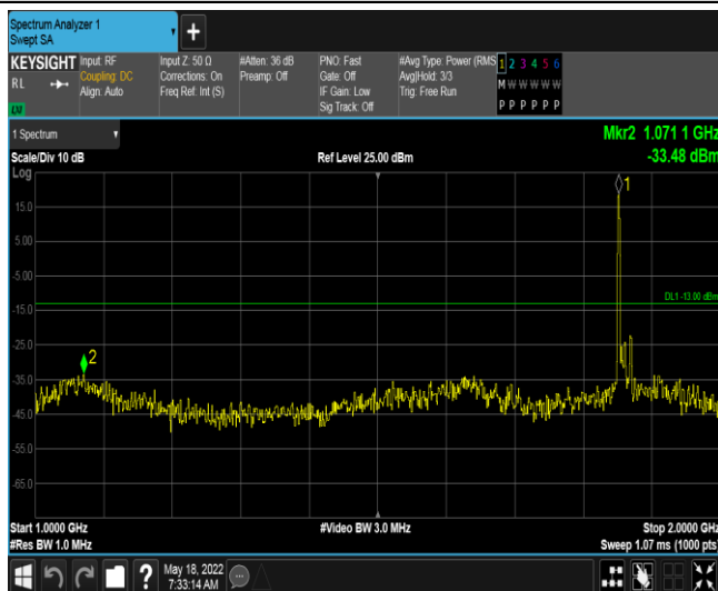
Band2-10MHz-16QAM-18650-1RB#0-Range2:1000~2000MHz
