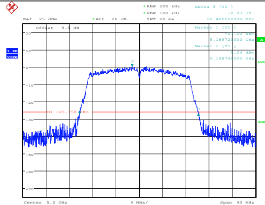
11AC20SISO-Ant1-5200
