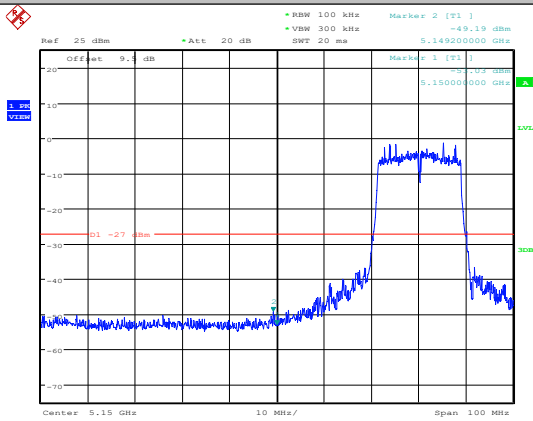
11AC20SISO-Ant1-5180
