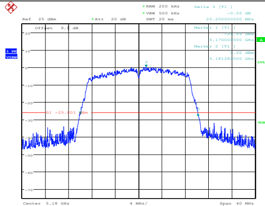
11AC20SISO-Ant1-5180
