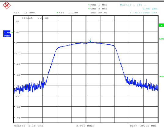
11A-Ant1-5180
