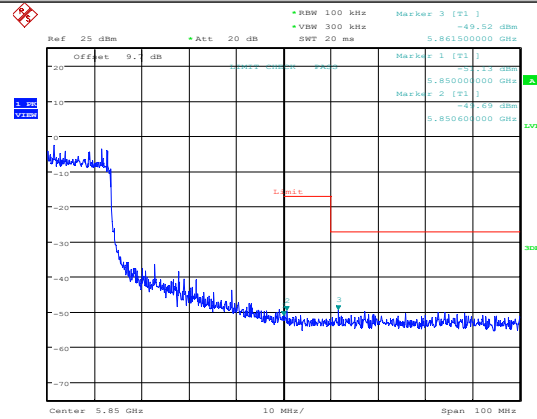
11AC40SISO-Ant1-5795
