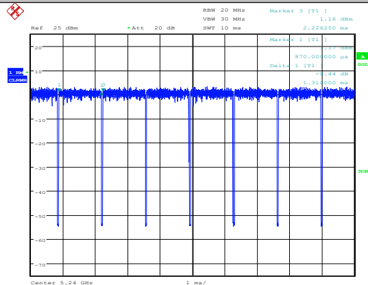
11AC20SISO-Ant1-5240
