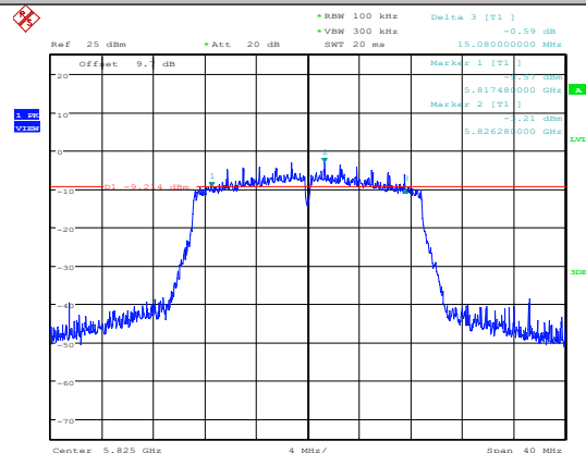
11AC20SISO-Ant1-5825
