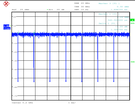
11AC20SISO-Ant1-5200
