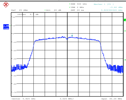
11N20SISO-Ant1-5825
