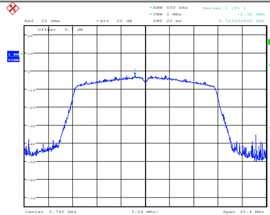
11AC20SISO-Ant1-5745
