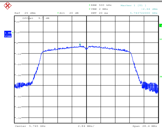
11N20SISO-Ant1-5745
