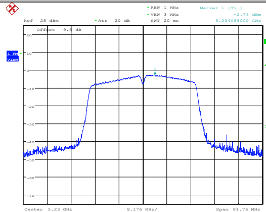
11AC40SISO-Ant1-5230
