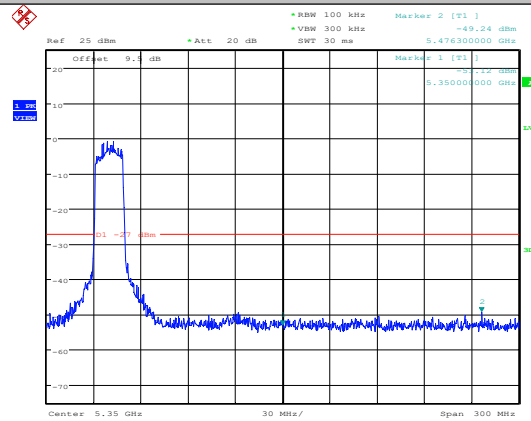
11AC20SISO-Ant1-5240
