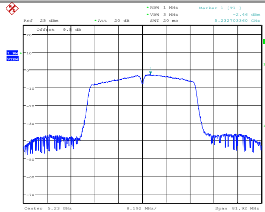
11N40SISO-Ant1-5230
