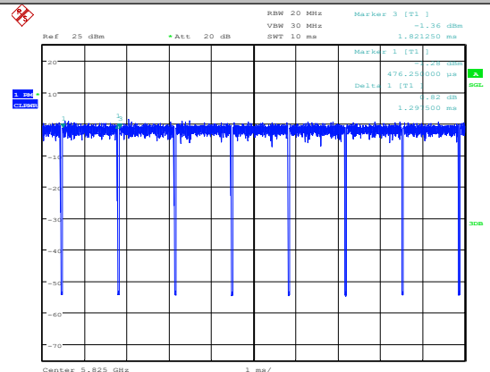
11N20SISO-Ant1-5825
