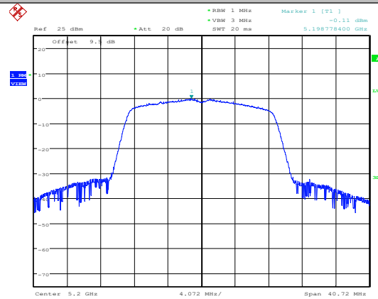
11N20SISO-Ant1-5200
