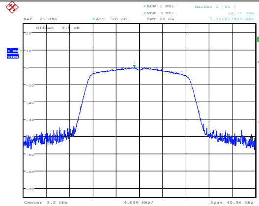
11AC20SISO-Ant1-5200
