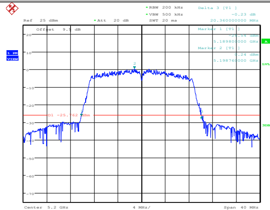
11N20SISO-Ant1-5200
