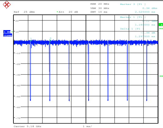
11N20SISO-Ant1-5180
