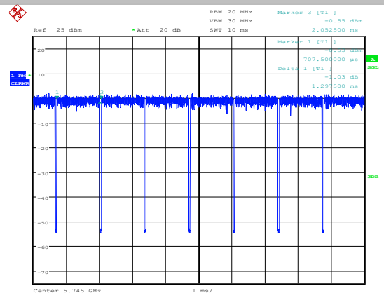
11N20SISO-Ant1-5745
