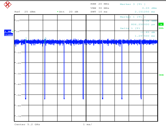
11N20SISO-Ant1-5200
