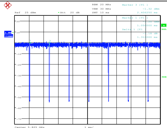
11AC20SISO-Ant1-5825
