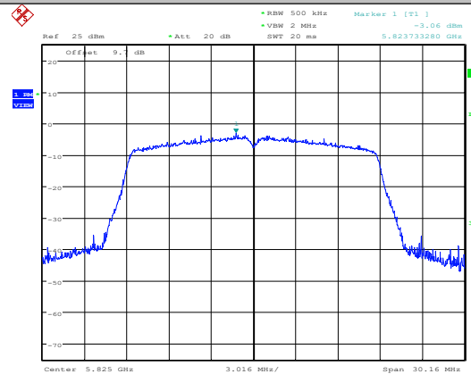
11AC20SISO-Ant1-5825
