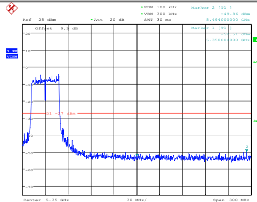
11AC40SISO-Ant1-5230
