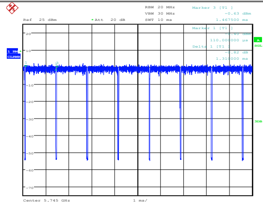
11AC20SISO-Ant1-5745
