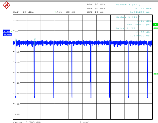
11AC20SISO-Ant1-5785
