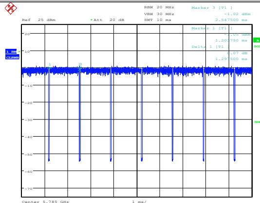
11N20SISO-Ant1-5785
