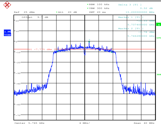
11AC20SISO-Ant1-5745
