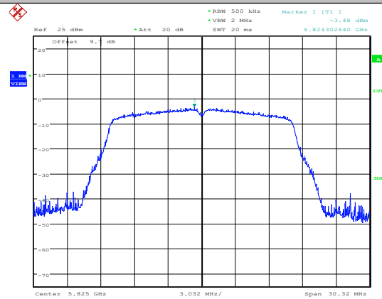
11A-Ant1-5825
