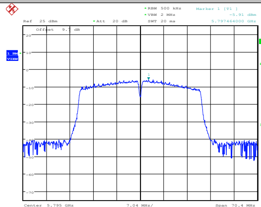
11N40SISO-Ant1-5795
