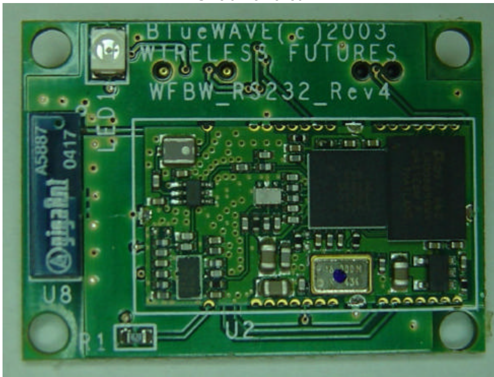
Shield Removed
