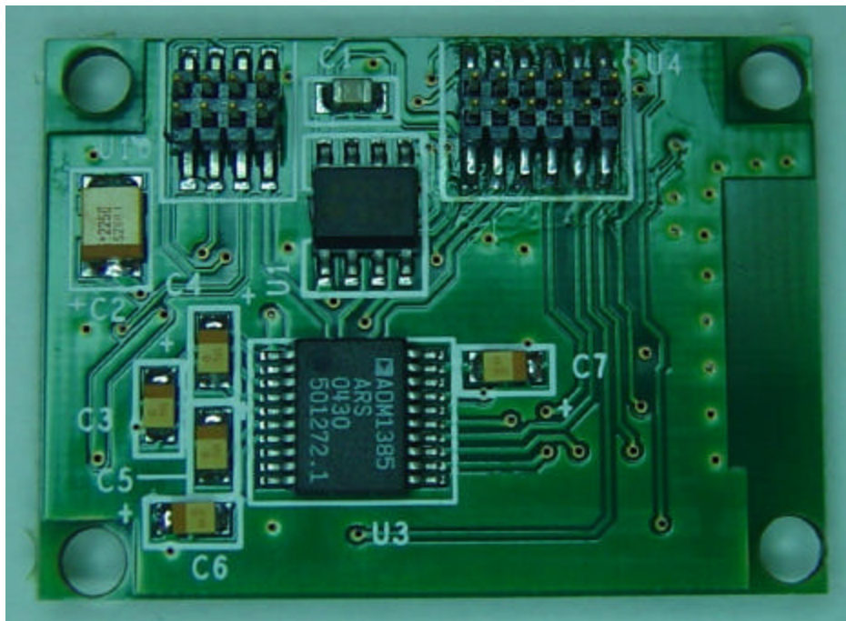
Main board with Reader-Foil Side
