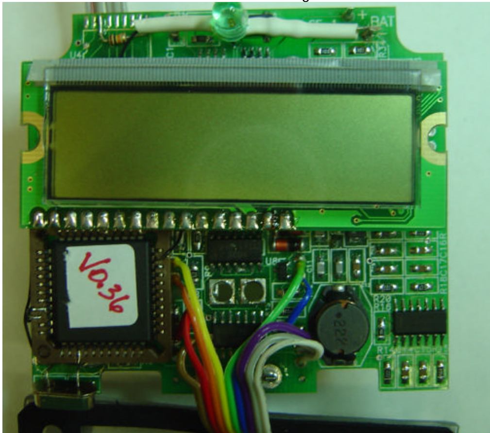
Main Board and LCD together
