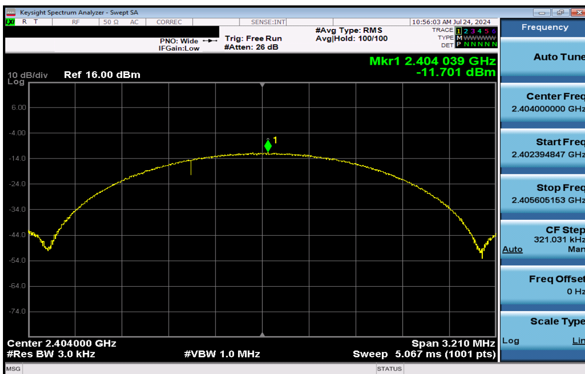
Plot 7-46. Power Spectral Density Plot Antenna WF2 (Bluetooth (LE), 2Mbps, iPA – Ch. 1)
