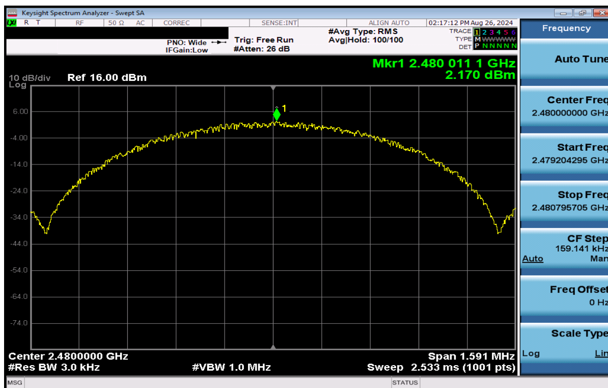
Plot 7-54. Power Spectral Density Plot Antenna WF7 (Bluetooth (LE), 1Mbps, ePA – Ch. 39)
