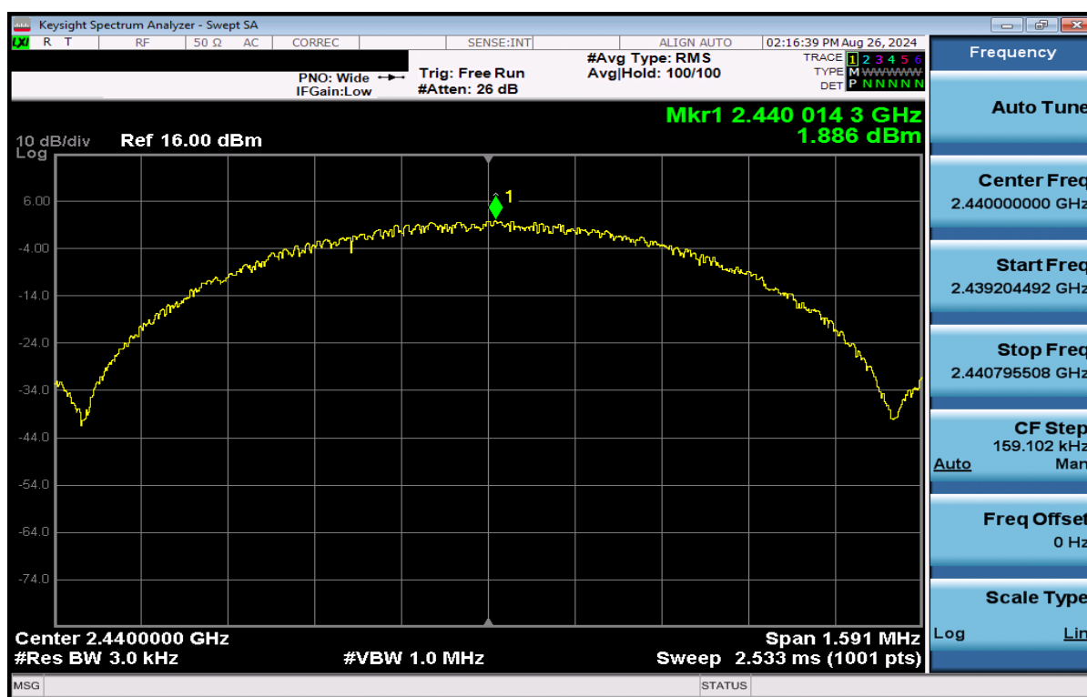
Plot 7-52. Power Spectral Density Plot Antenna WF7 (Bluetooth (LE), 1Mbps, ePA – Ch. 19)
