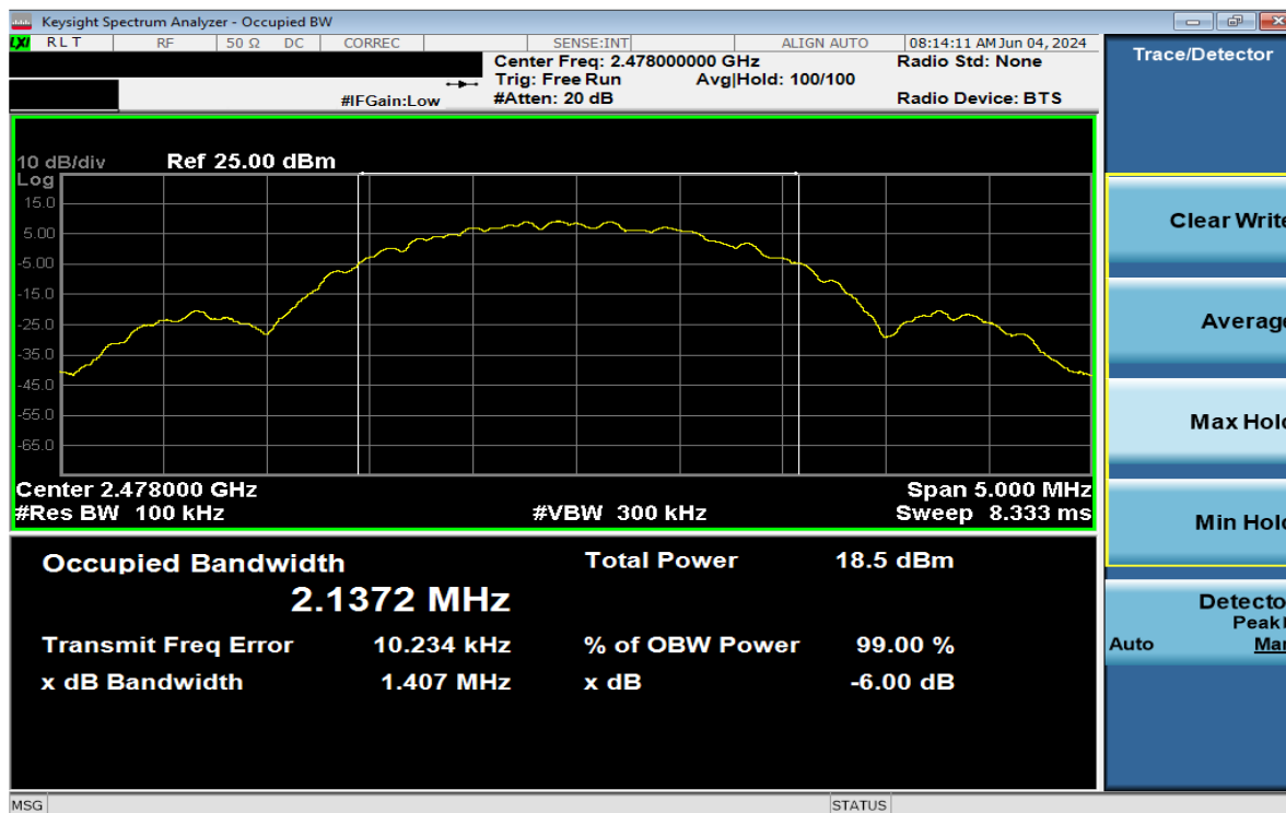
Plot 7-18. 6dB BW & 99% OBW Plot Antenna WF2 (Bluetooth (LE), 2Mbps, iPA – Ch. 38)
