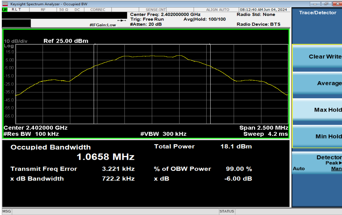
Plot 7-13. 6dB BW & 99% OBW Plot Antenna WF2 (Bluetooth (LE), 1Mbps, iPA – Ch. 0)
