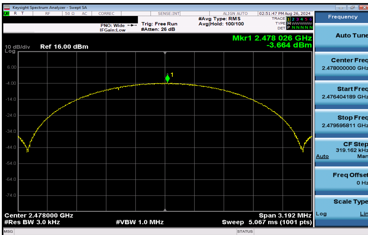
Plot 7-65. Power Spectral Density Plot Antenna WF8 (Bluetooth (LE), 2Mbps, ePA – Ch. 38)
