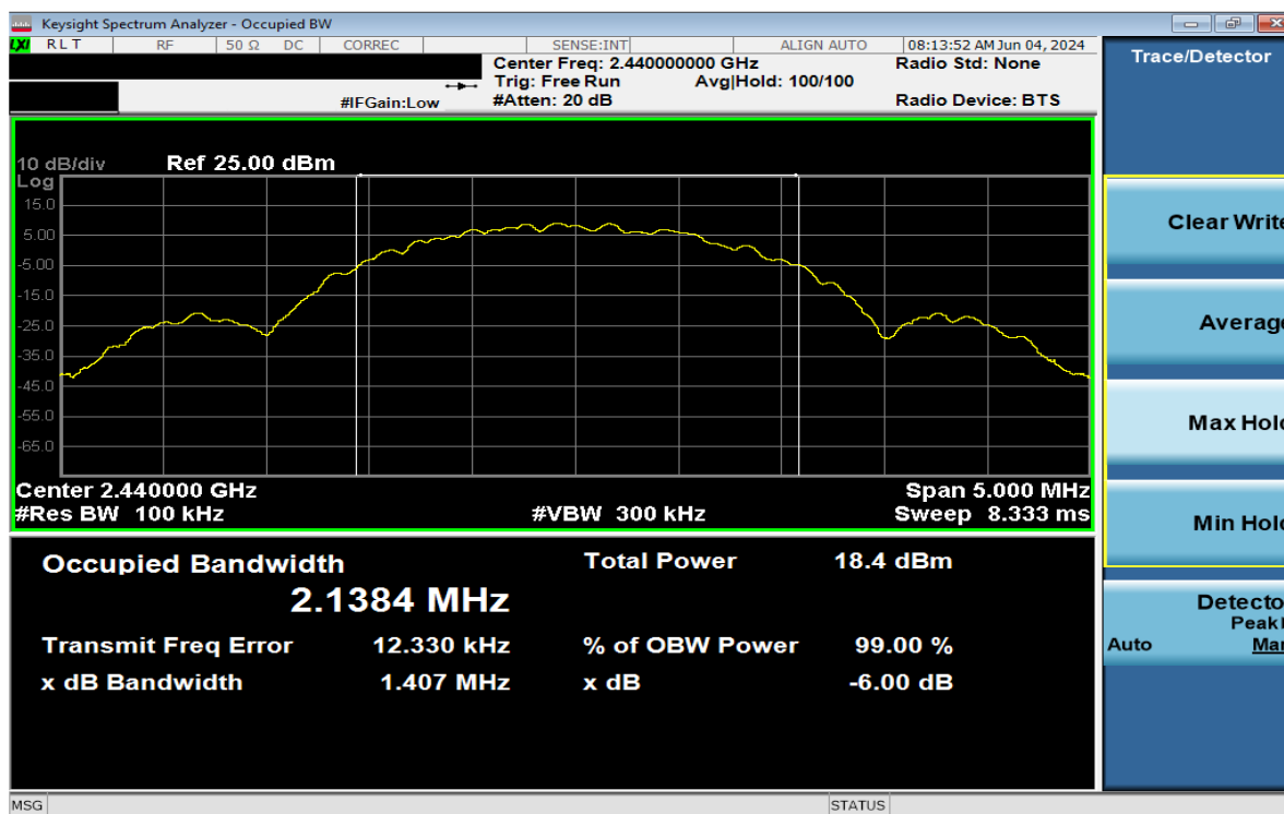
Plot 7-17. 6dB BW & 99% OBW Plot Antenna WF2 (Bluetooth (LE), 2Mbps, iPA – Ch. 19)
