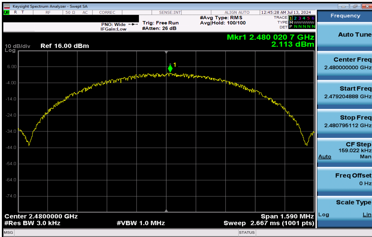
Plot 7-21. Power Spectral Density Plot Antenna WF8 (Bluetooth (LE), 1Mbps, ePA – Ch. 39)
