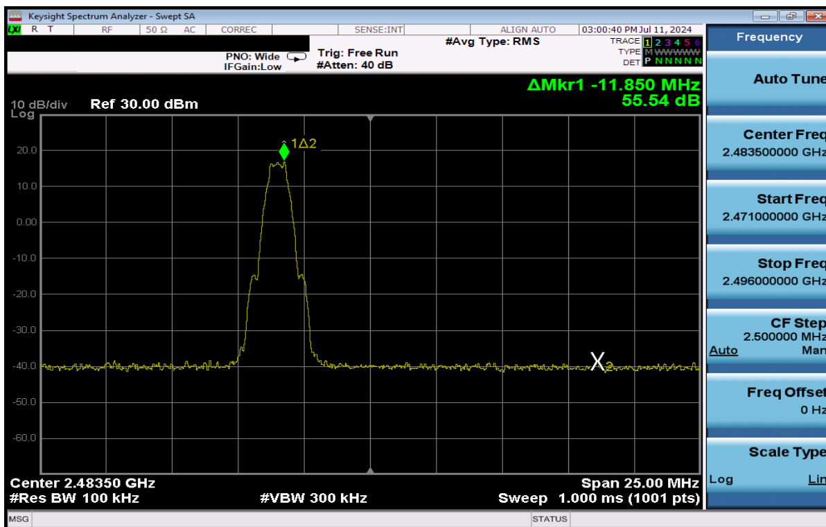
Plot 7-78. Band Edge Plot Antenna WF7 (Bluetooth (LE), 1Mbps, ePA – Ch. 39)
