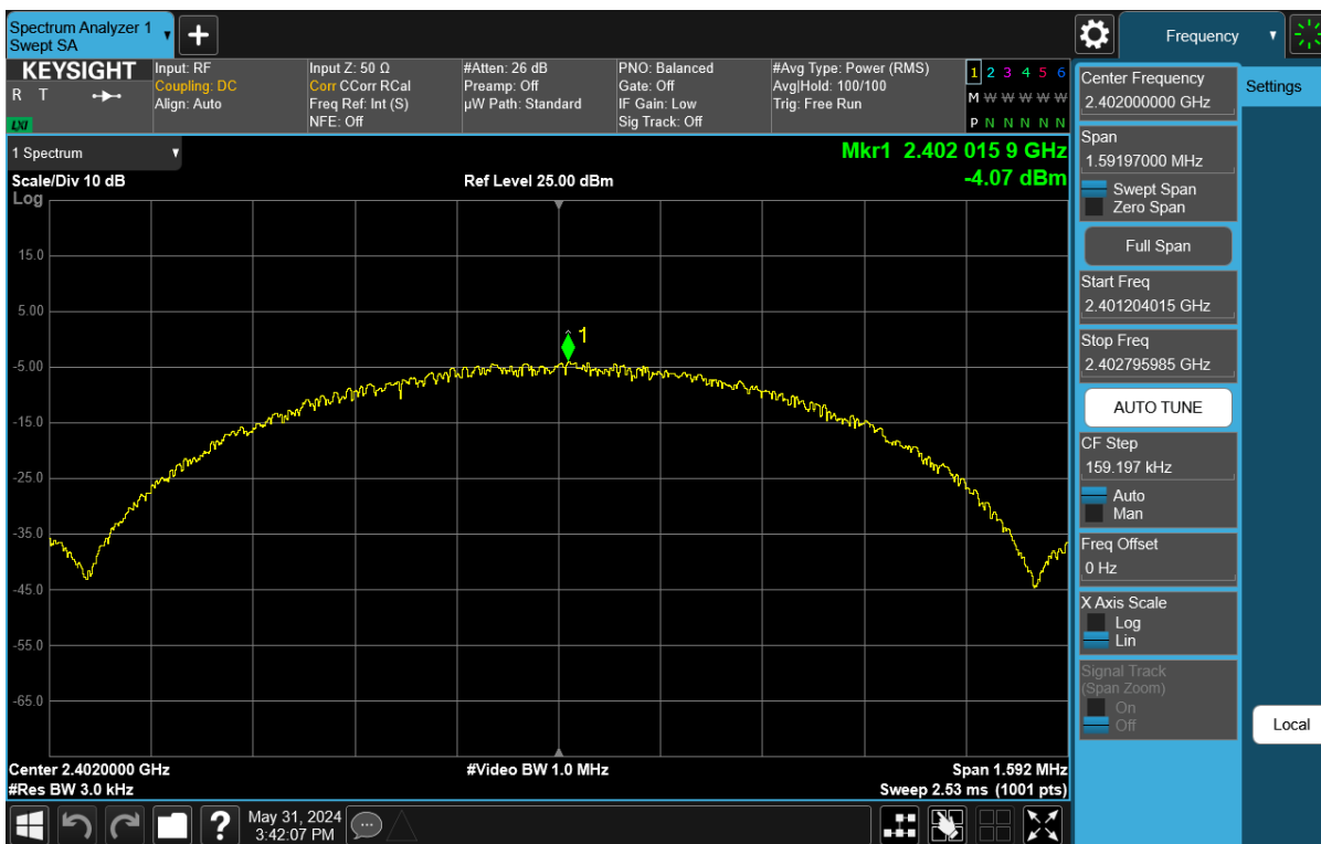
Plot 7-22. Power Spectral Density Plot Antenna WF8 (Bluetooth (LE), 1Mbps, iPA – Ch. 0)
