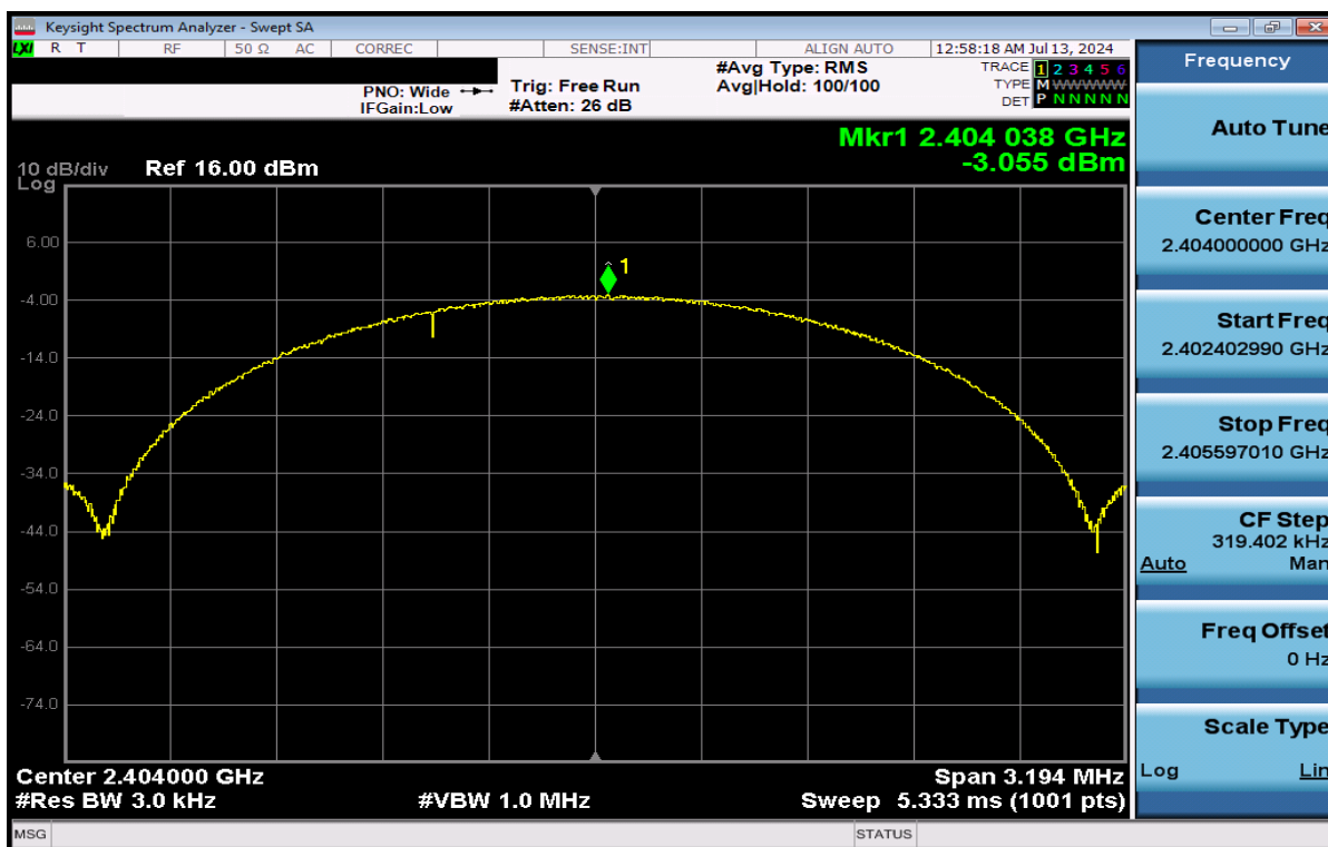
Plot 7-37. Power Spectral Density Plot Antenna WF7 (Bluetooth (LE), 2Mbps, ePA – Ch. 1)
