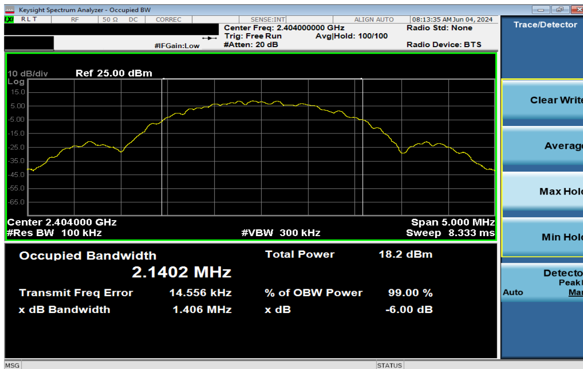
Plot 7-16. 6dB BW & 99% OBW Plot Antenna WF2 (Bluetooth (LE), 2Mbps, iPA – Ch. 1)
