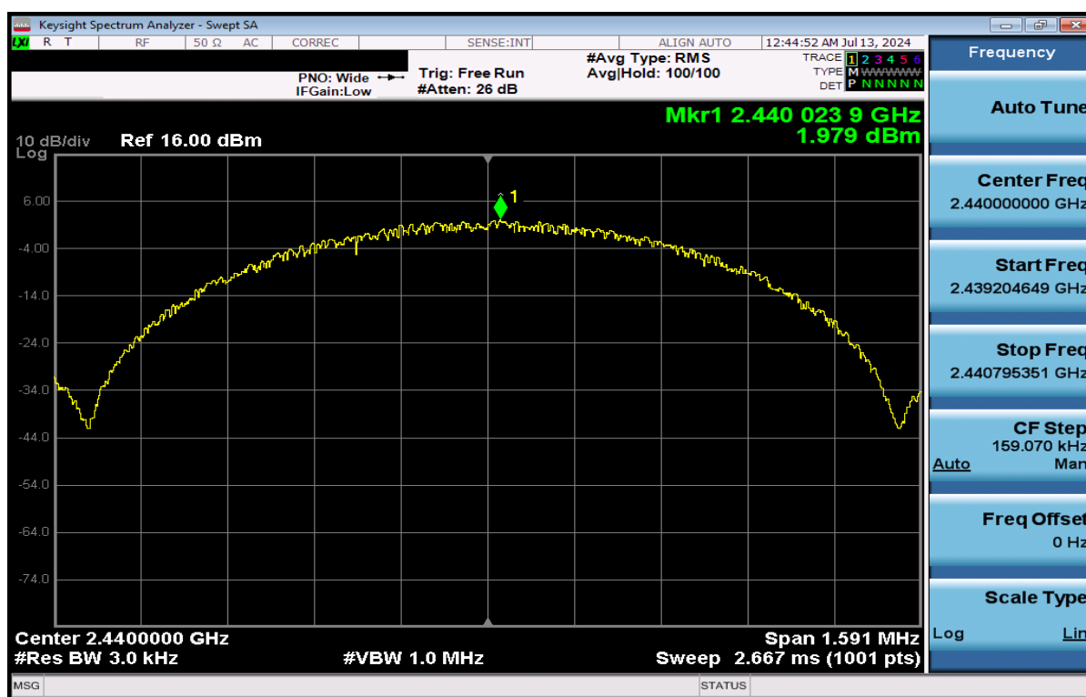
Plot 7-20. Power Spectral Density Plot Antenna WF8 (Bluetooth (LE), 1Mbps, ePA – Ch. 19)
