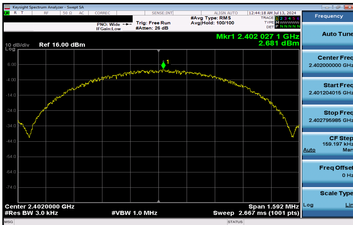
Plot 7-19. Power Spectral Density Plot Antenna WF8 (Bluetooth (LE), 1Mbps, ePA – Ch. 0)
