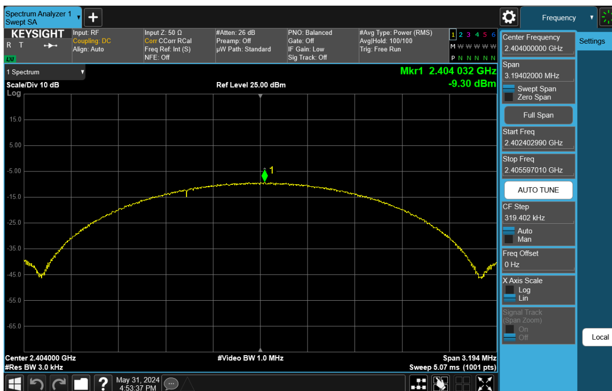
Plot 7-40. Power Spectral Density Plot Antenna WF7 (Bluetooth (LE), 2Mbps, iPA – Ch. 1)
