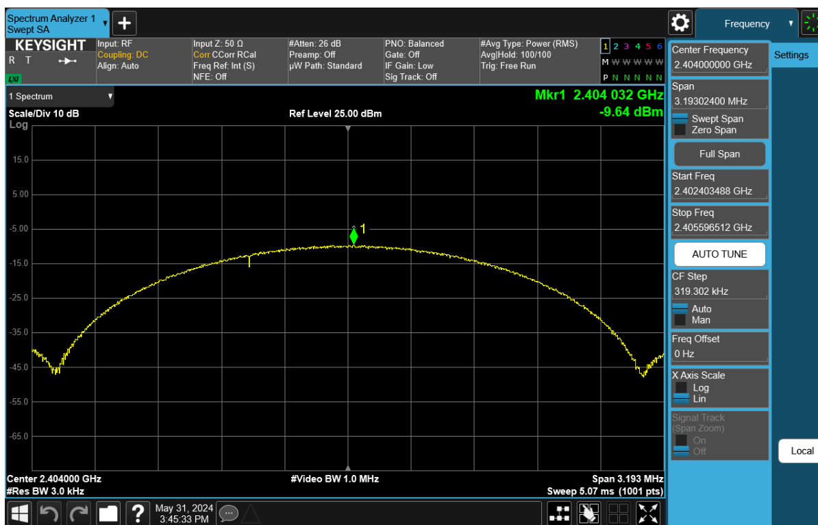
Plot 7-28. Power Spectral Density Plot Antenna WF8 (Bluetooth (LE), 2Mbps, iPA – Ch. 1)
