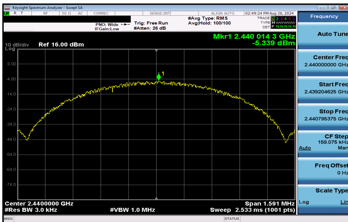
Plot 7-57. Power Spectral Density Plot Antenna WF8 (Bluetooth (LE), 1Mbps, iPA – Ch. 19)
