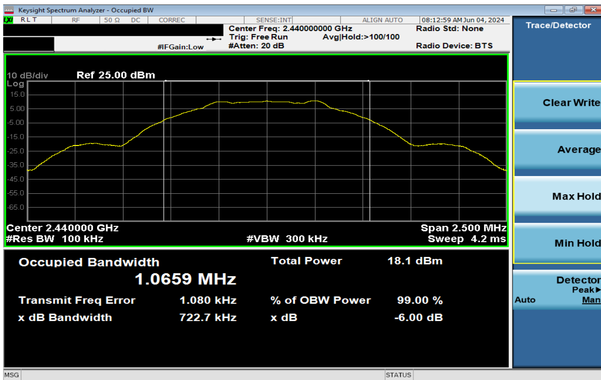
Plot 7-14. 6dB BW & 99% OBW Plot Antenna WF2 (Bluetooth (LE), 1Mbps, iPA – Ch. 19)
