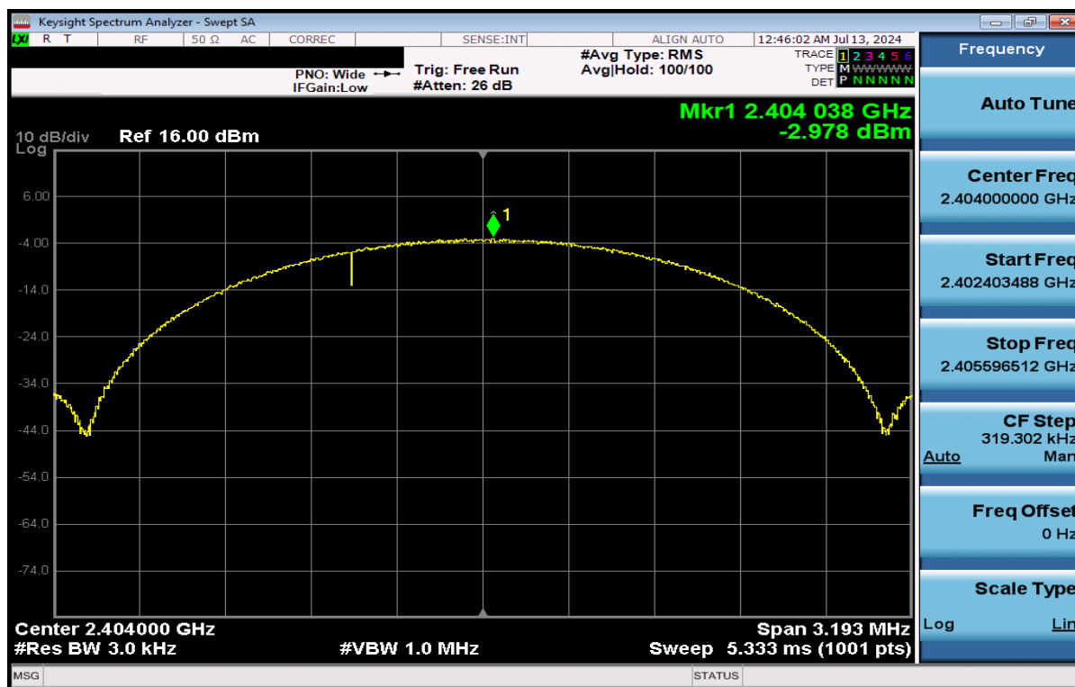
Plot 7-25. Power Spectral Density Plot Antenna WF8 (Bluetooth (LE), 2Mbps, ePA – Ch. 1)
