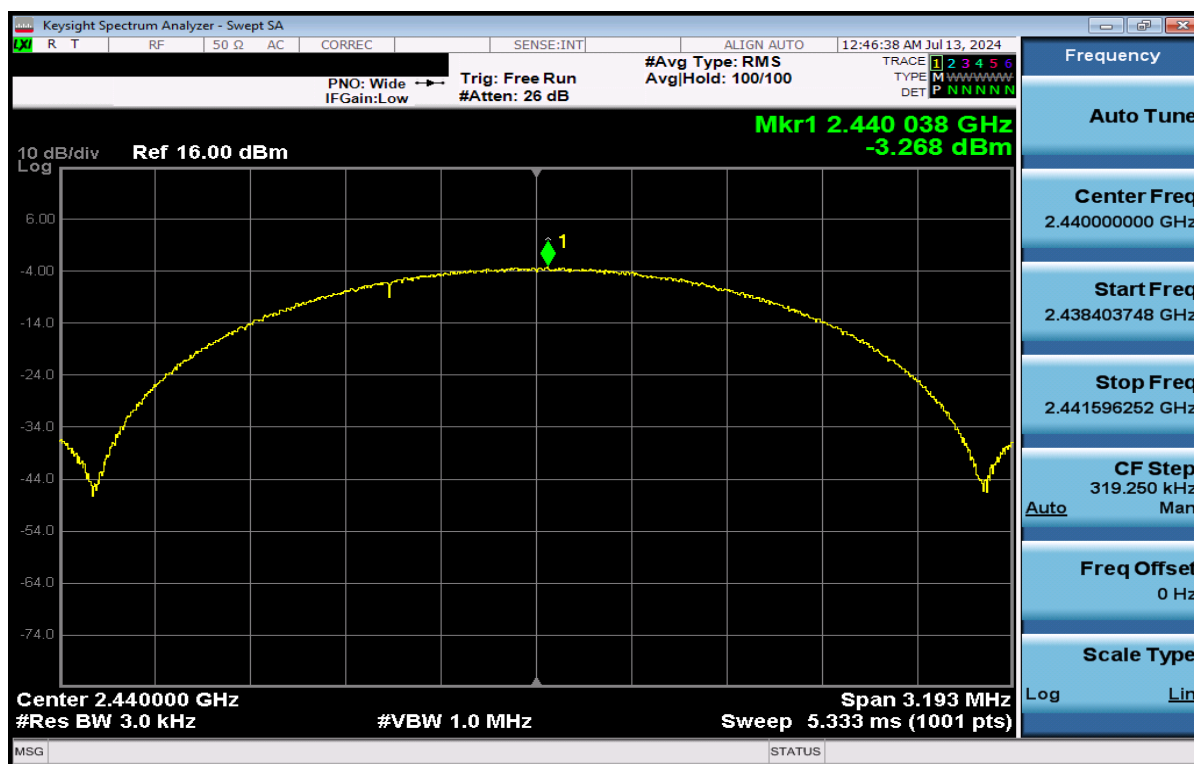
Plot 7-26. Power Spectral Density Plot Antenna WF8 (Bluetooth (LE), 2Mbps, ePA – Ch. 19)
