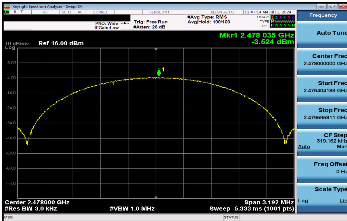
Plot 7-27. Power Spectral Density Plot Antenna WF8 (Bluetooth (LE), 2Mbps, ePA – Ch. 38)
