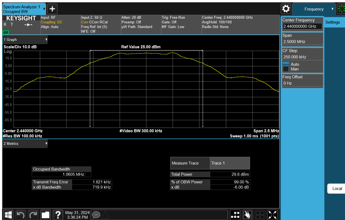
Plot 7-2. 6dB BW & 99% OBW Plot Antenna WF8 (Bluetooth (LE), 1Mbps, ePA – Ch. 19)
