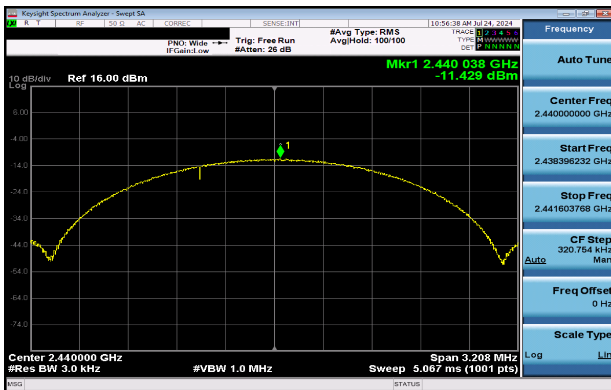
Plot 7-47. Power Spectral Density Plot Antenna WF2 (Bluetooth (LE), 2Mbps, iPA – Ch. 19)
