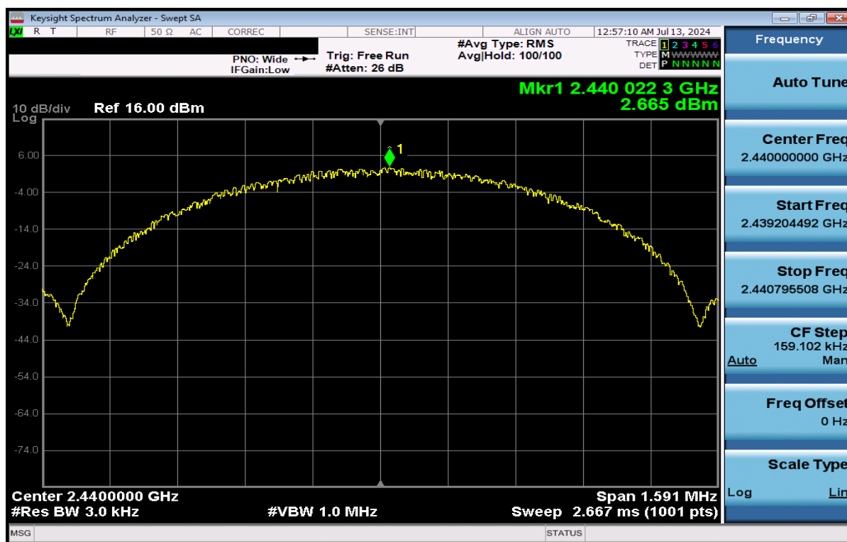
Plot 7-32. Power Spectral Density Plot Antenna WF7 (Bluetooth (LE), 1Mbps, ePA – Ch. 19)
