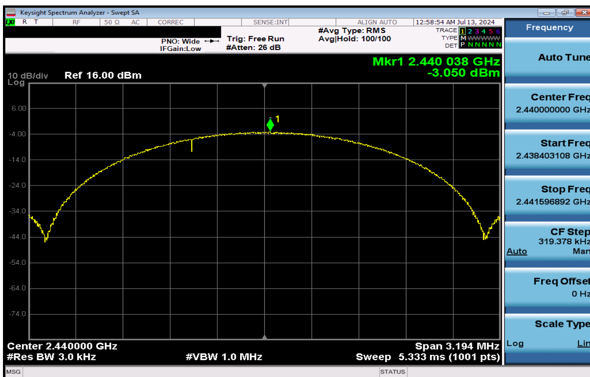
Plot 7-38. Power Spectral Density Plot Antenna WF7 (Bluetooth (LE), 2Mbps, ePA – Ch. 19)
