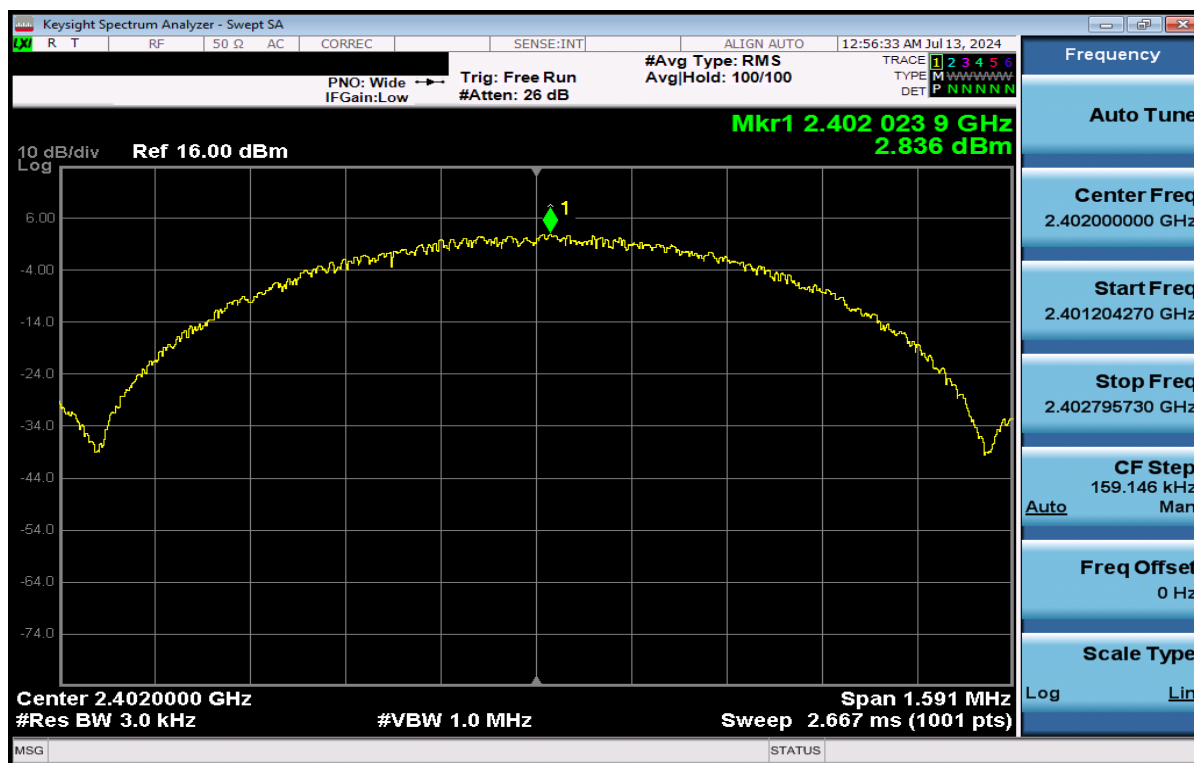
Plot 7-31. Power Spectral Density Plot Antenna WF7 (Bluetooth (LE), 1Mbps, ePA – Ch. 0)
