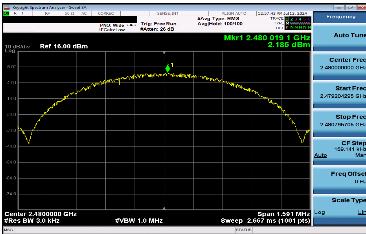
Plot 7-33. Power Spectral Density Plot Antenna WF7 (Bluetooth (LE), 1Mbps, ePA – Ch. 39)
