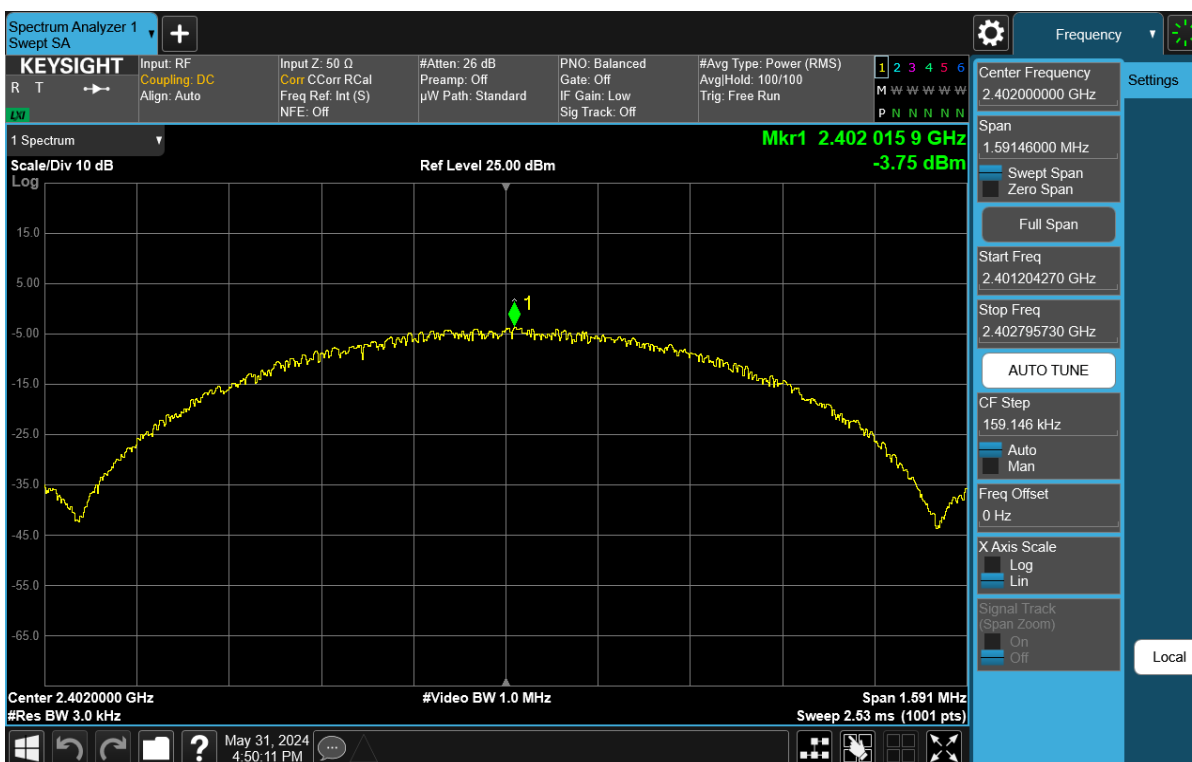
Plot 7-34. Power Spectral Density Plot Antenna WF7 (Bluetooth (LE), 1Mbps, iPA – Ch. 0)
