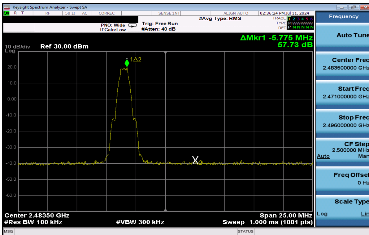
Plot 7-74. Band Edge Plot Antenna WF8 (Bluetooth (LE), 1Mbps, ePA – Ch. 39)
