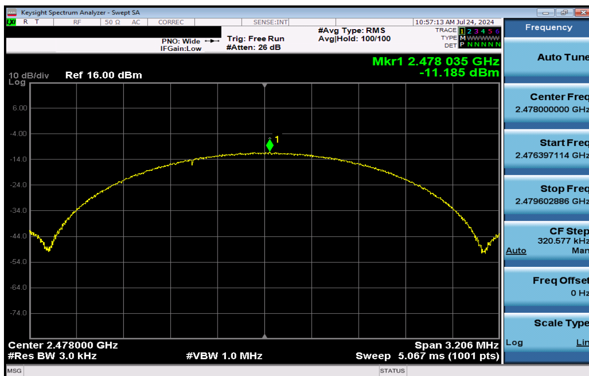
Plot 7-48. Power Spectral Density Plot Antenna WF2 (Bluetooth (LE), 2Mbps, iPA – Ch. 38)
