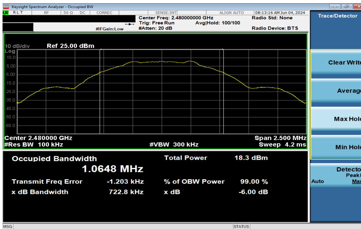
Plot 7-15. 6dB BW & 99% OBW Plot Antenna WF2 (Bluetooth (LE), 1Mbps, iPA – Ch. 39)
