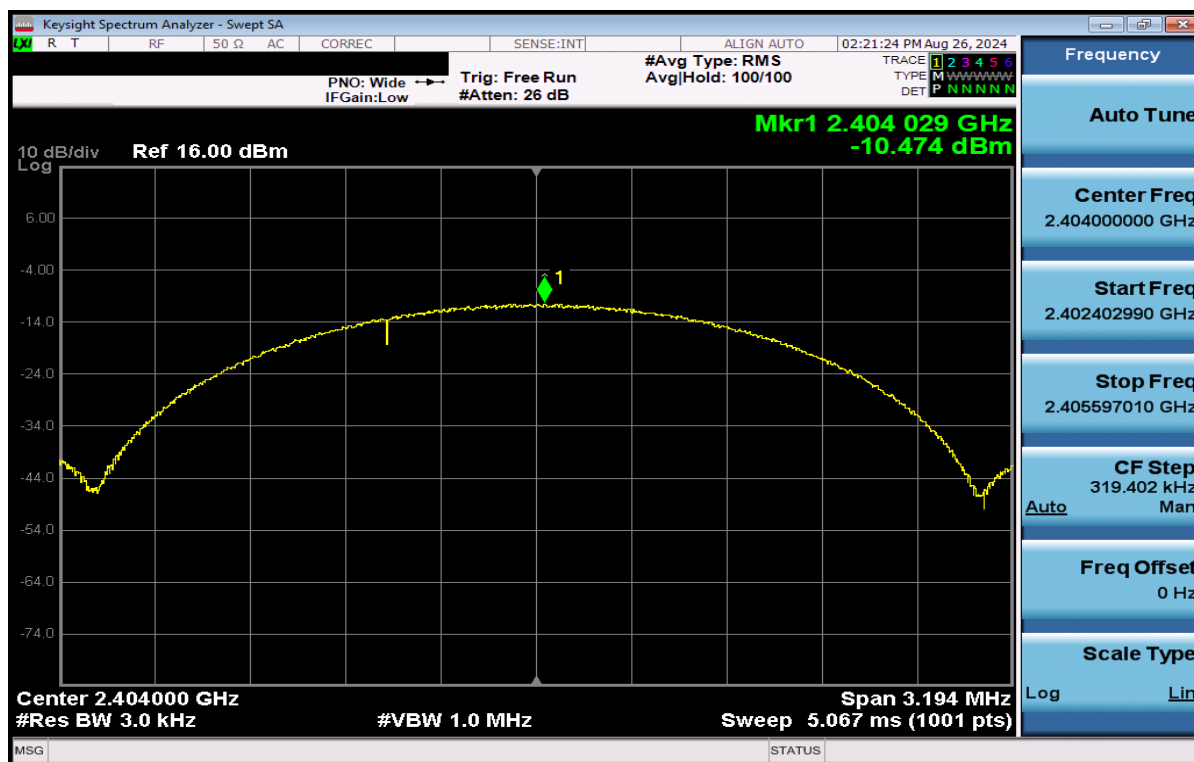
Plot 7-68. Power Spectral Density Plot Antenna WF7 (Bluetooth (LE), 2Mbps, iPA – Ch. 1)
