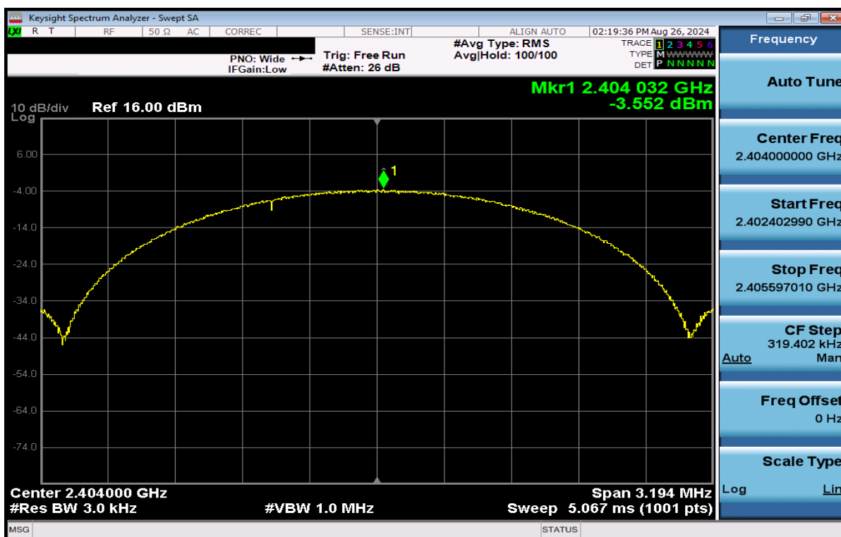
Plot 7-62. Power Spectral Density Plot Antenna WF7 (Bluetooth (LE), 2Mbps, ePA – Ch. 1)
