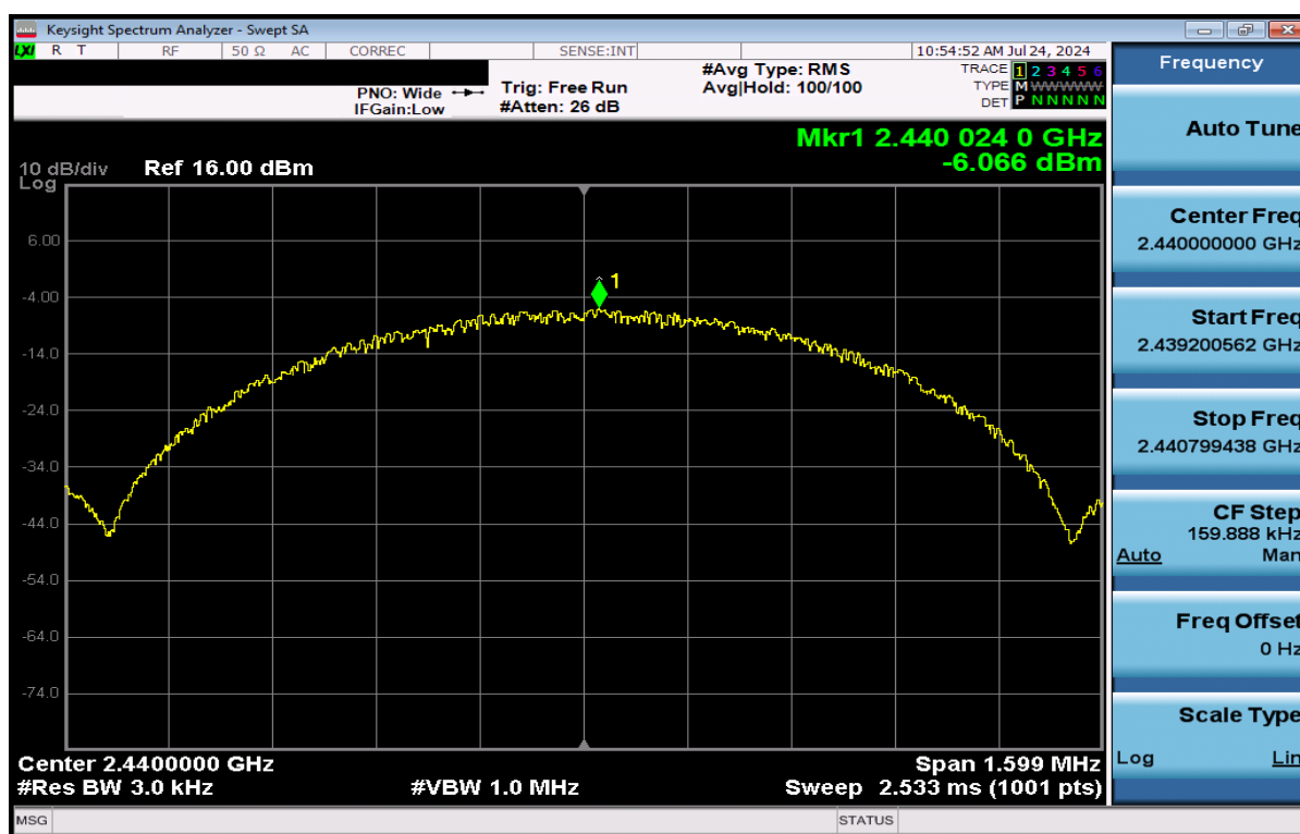
Plot 7-44. Power Spectral Density Plot Antenna WF2 (Bluetooth (LE), 1Mbps, iPA – Ch. 19)
