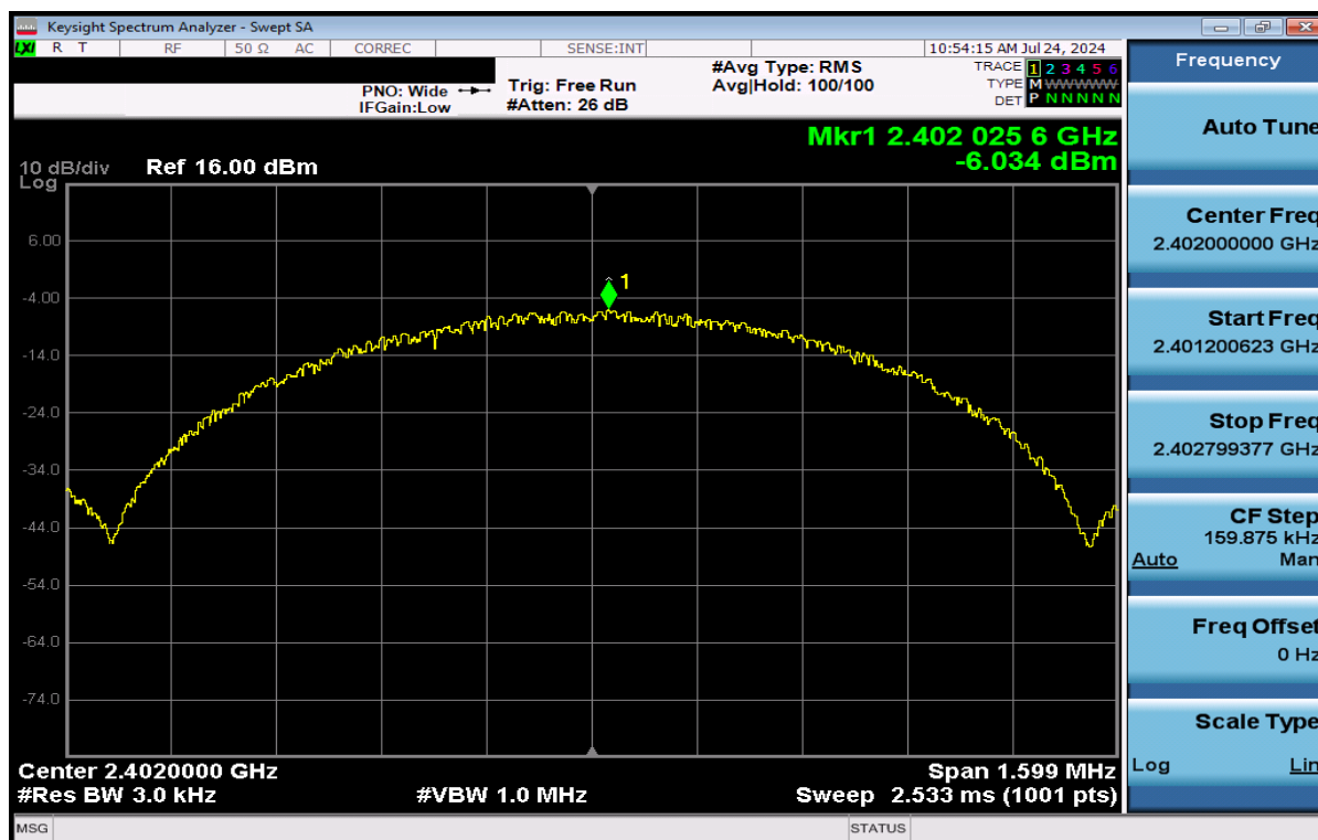
Plot 7-43. Power Spectral Density Plot Antenna WF2 (Bluetooth (LE), 1Mbps, iPA – Ch. 0)
