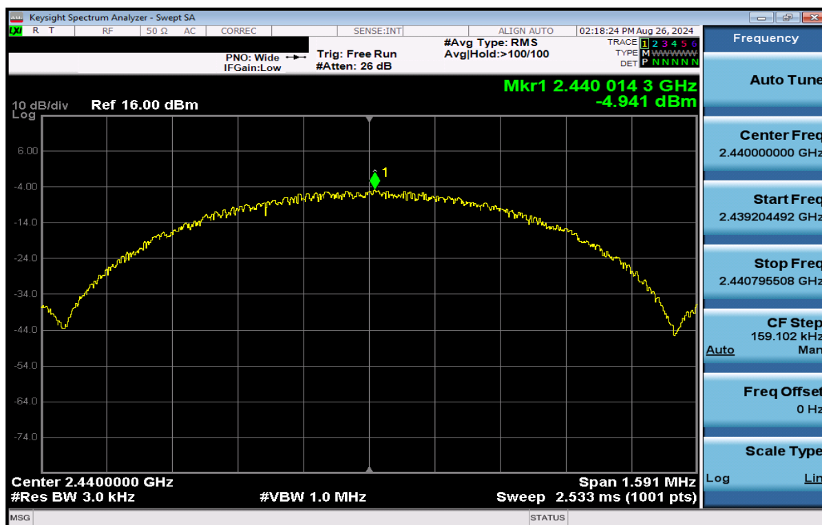
Plot 7-58. Power Spectral Density Plot Antenna WF7 (Bluetooth (LE), 1Mbps, iPA – Ch. 19)
