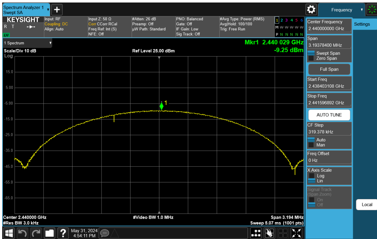
Plot 7-41. Power Spectral Density Plot Antenna WF7 (Bluetooth (LE), 2Mbps, iPA – Ch. 19)
