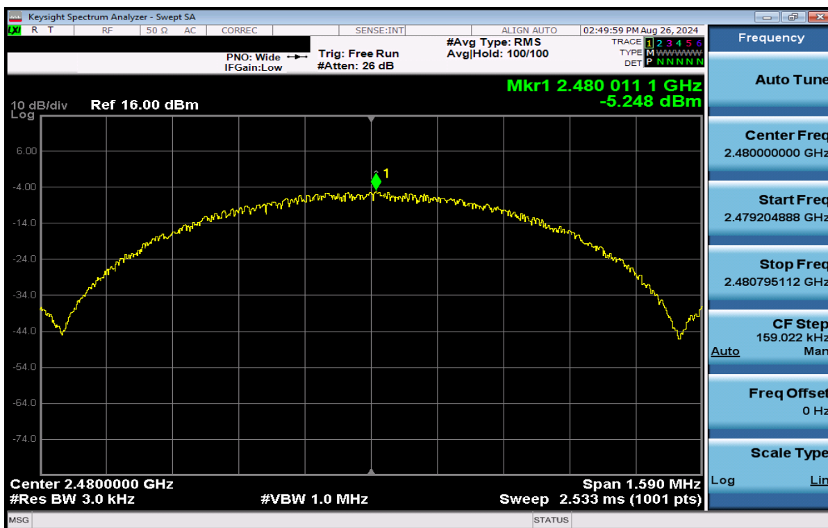
Plot 7-59. Power Spectral Density Plot Antenna WF8 (Bluetooth (LE), 1Mbps, iPA – Ch. 39)
