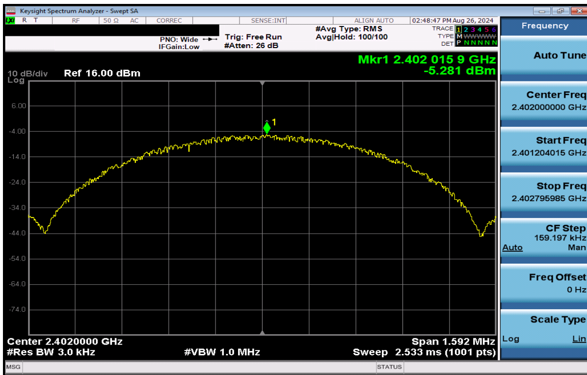
Plot 7-55. Power Spectral Density Plot Antenna WF8 (Bluetooth (LE), 1Mbps, iPA – Ch. 0)
