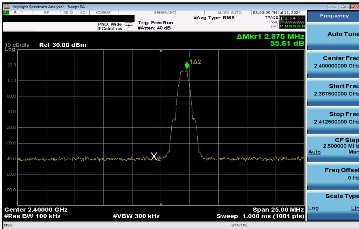
Plot 7-77. Band Edge Plot Antenna WF7 (Bluetooth (LE), 1Mbps, ePA – Ch.0)
