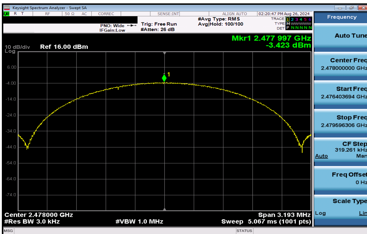
Plot 7-66. Power Spectral Density Plot Antenna WF7 (Bluetooth (LE), 2Mbps, ePA – Ch. 38)
