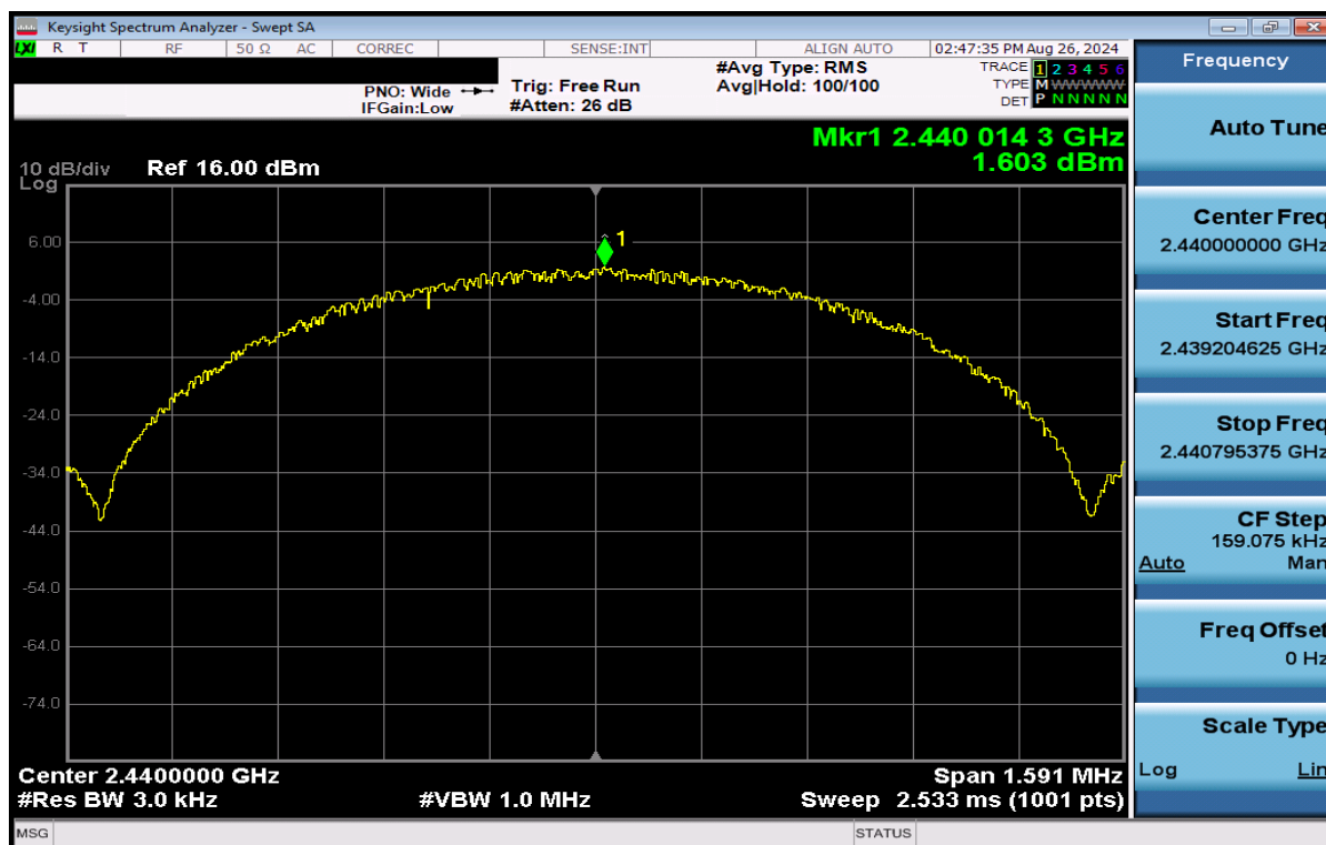
Plot 7-51. Power Spectral Density Plot Antenna WF8 (Bluetooth (LE), 1Mbps, ePA – Ch. 19)
