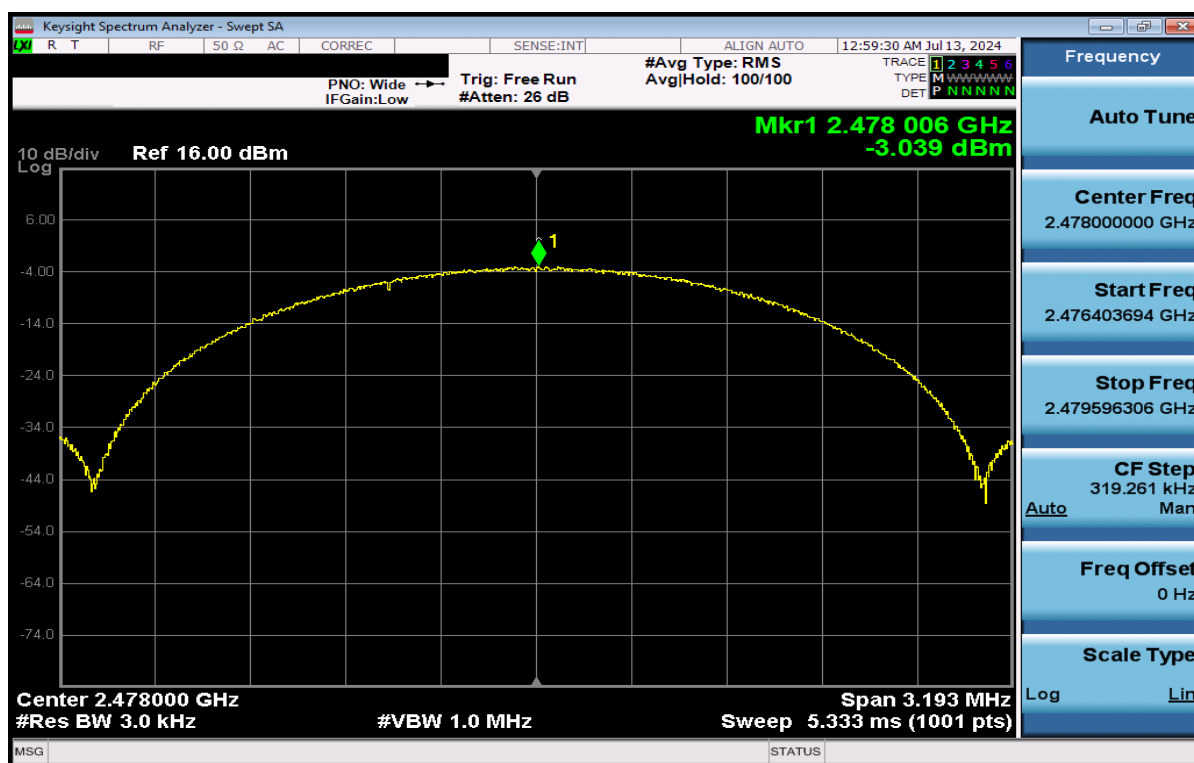
Plot 7-39. Power Spectral Density Plot Antenna WF7 (Bluetooth (LE), 2Mbps, ePA – Ch. 38)
