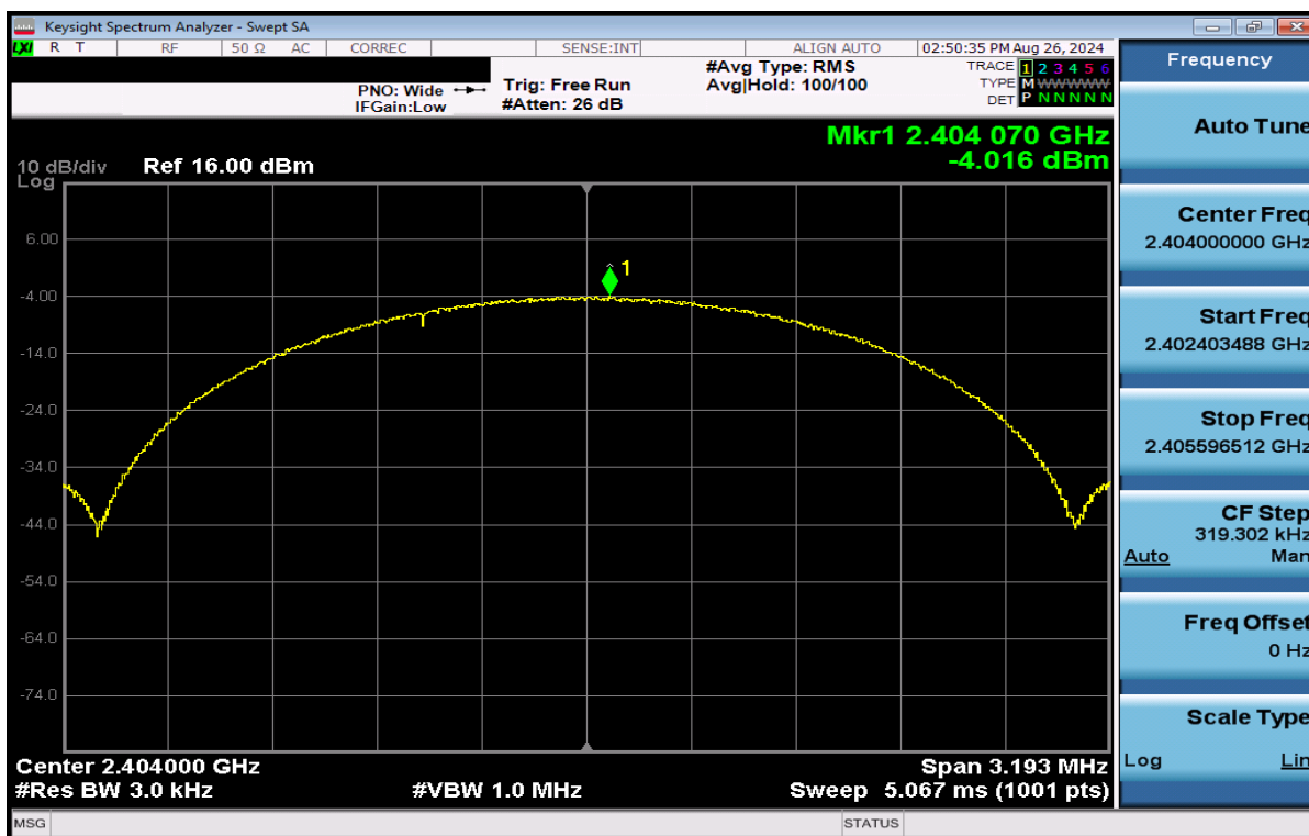
Plot 7-61. Power Spectral Density Plot Antenna WF8 (Bluetooth (LE), 2Mbps, ePA – Ch. 1)
