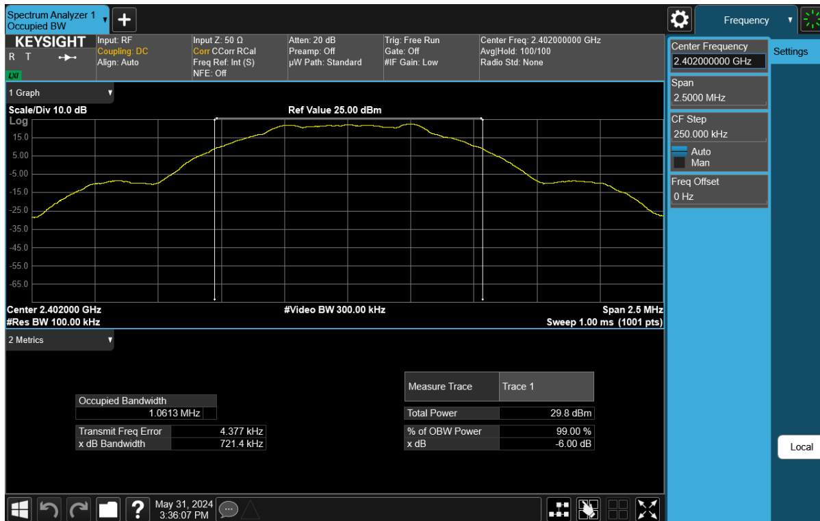
Plot 7-1. 6dB BW & 99% OBW Plot Antenna WF8 (Bluetooth (LE), 1Mbps, ePA – Ch. 0)
