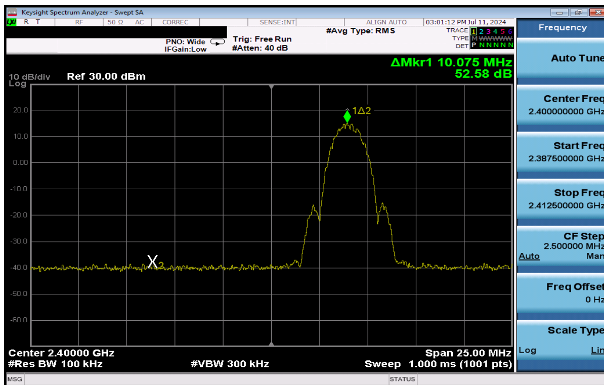
Plot 7-79. Band Edge Plot Antenna WF7 (Bluetooth (LE), 2Mbps, ePA – Ch. 1)
