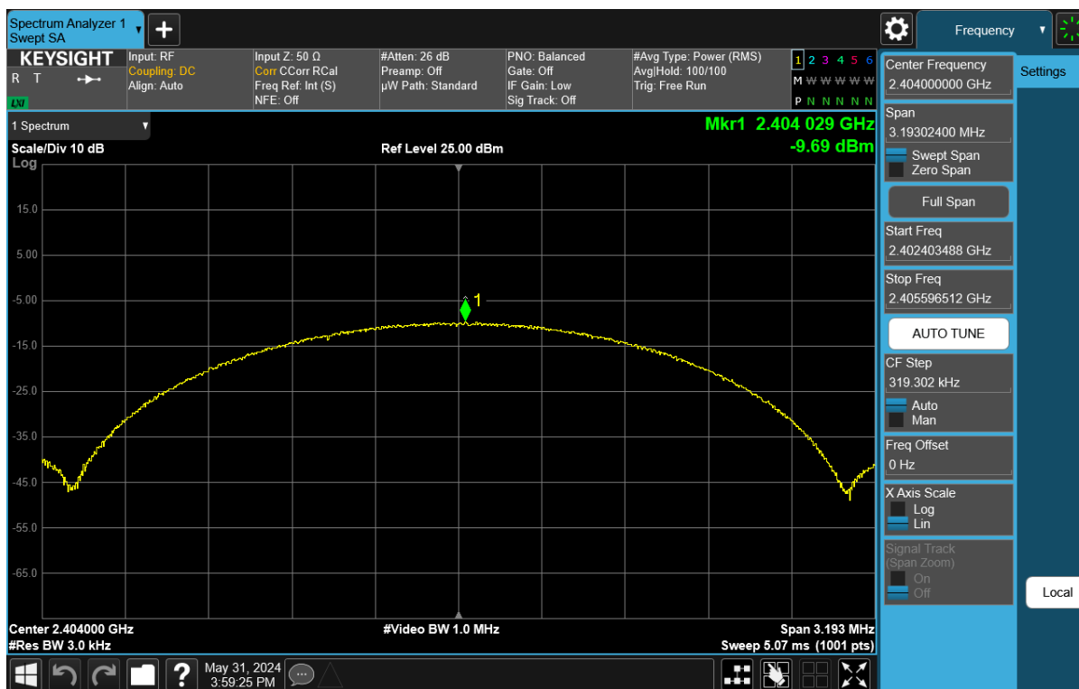
Plot 7-67. Power Spectral Density Plot Antenna WF8 (Bluetooth (LE), 2Mbps, iPA – Ch. 1)
