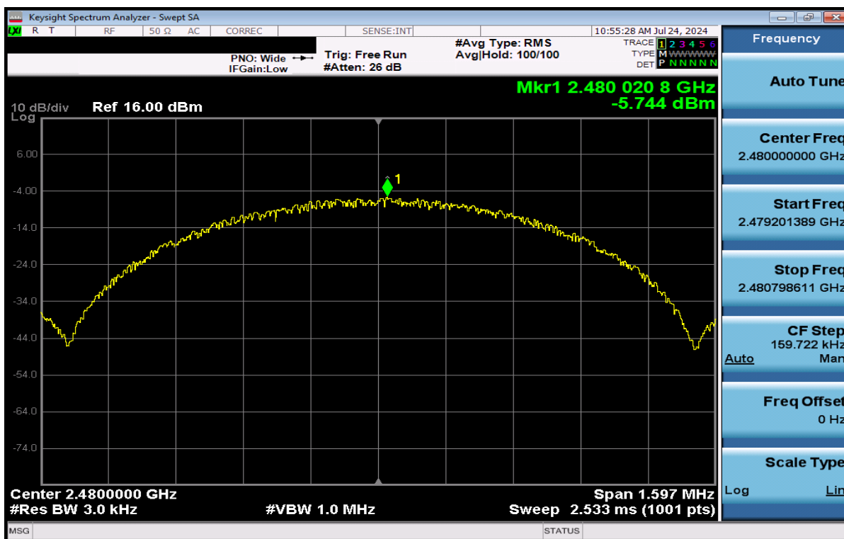
Plot 7-45. Power Spectral Density Plot Antenna WF2 (Bluetooth (LE), 1Mbps, iPA – Ch. 39)
