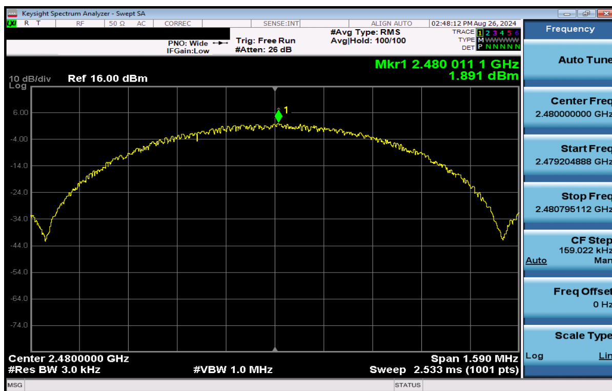
Plot 7-53. Power Spectral Density Plot Antenna WF8 (Bluetooth (LE), 1Mbps, ePA – Ch. 39)
