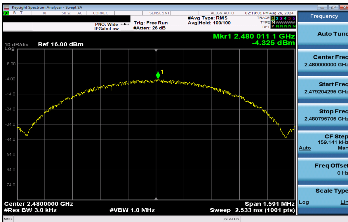
Plot 7-60. Power Spectral Density Plot Antenna WF7 (Bluetooth (LE), 1Mbps, iPA – Ch. 39)
