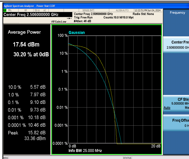
Band41-20MHz-16QAM-39750-100RB#0-PASS
