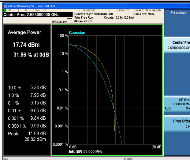
Band41-10MHz-16QAM-41540-50RB#0-PASS
