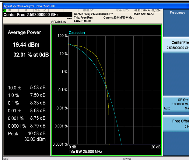
Band41-5MHz-16QAM-40620-1RB#0-PASS
