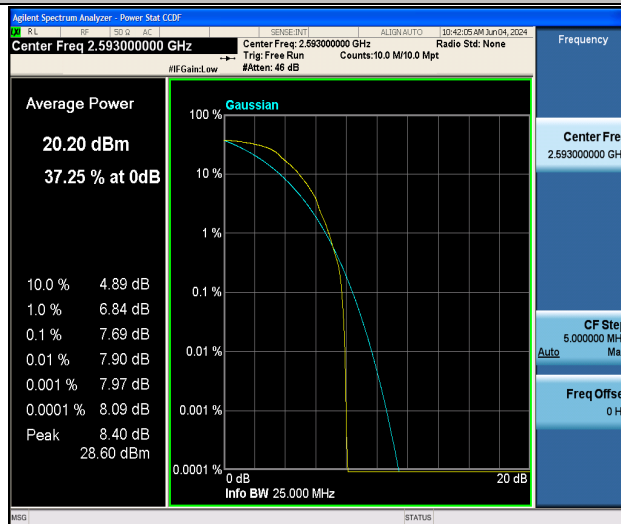
Band41-10MHz-QPSK-40620-1RB#0-PASS
