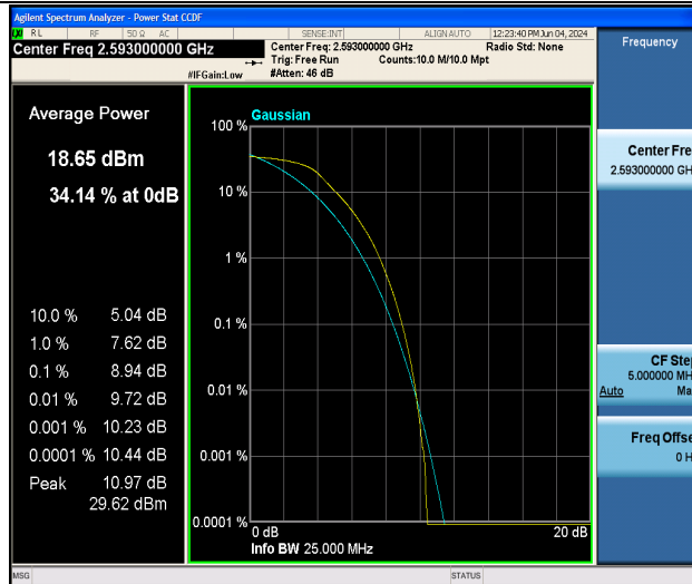
Band41-20MHz-QPSK-40620-100RB#0-PASS
