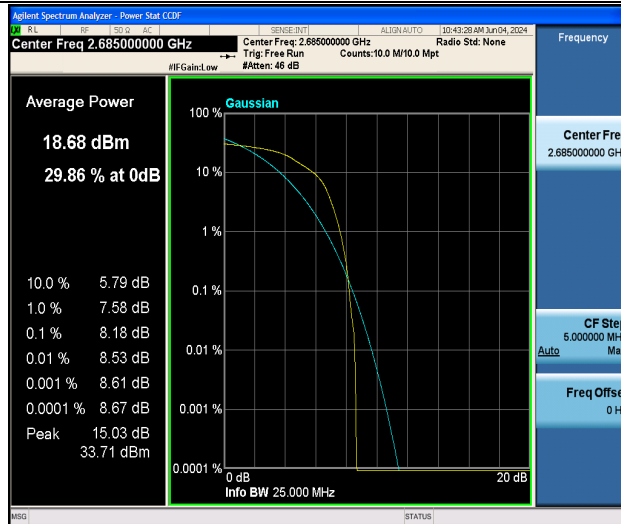
Band41-10MHz-16QAM-41540-1RB#0-PASS
