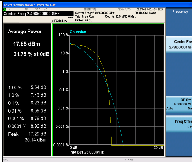
Band41-5MHz-16QAM-39675-25RB#0-PASS
