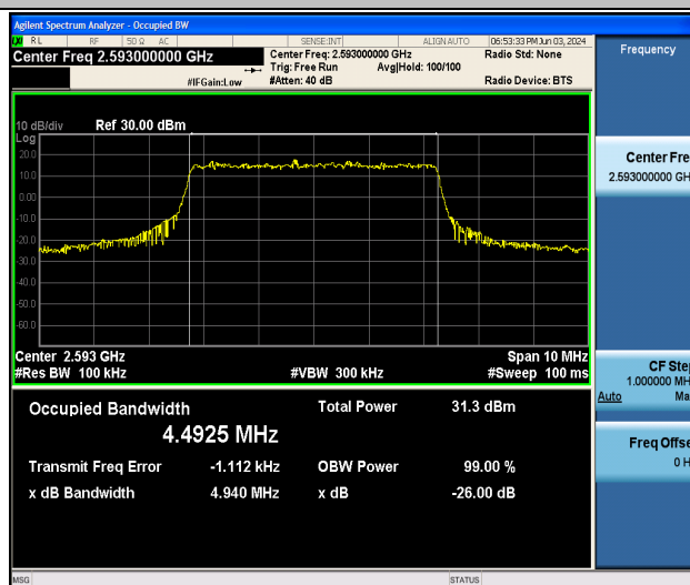
Band41-5MHz-QPSK-40620-25RB#0-PASS
