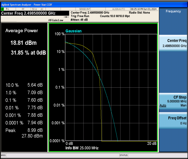
Band41-5MHz-16QAM-39675-1RB#0-PASS
