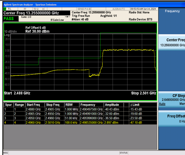
Band41_5MHz_QPSK_39675_25RB#0
