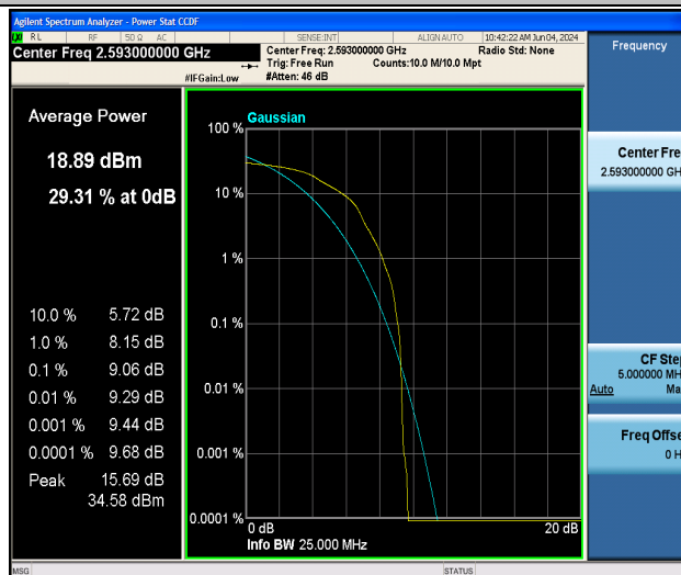
Band41-10MHz-16QAM-40620-1RB#0-PASS
