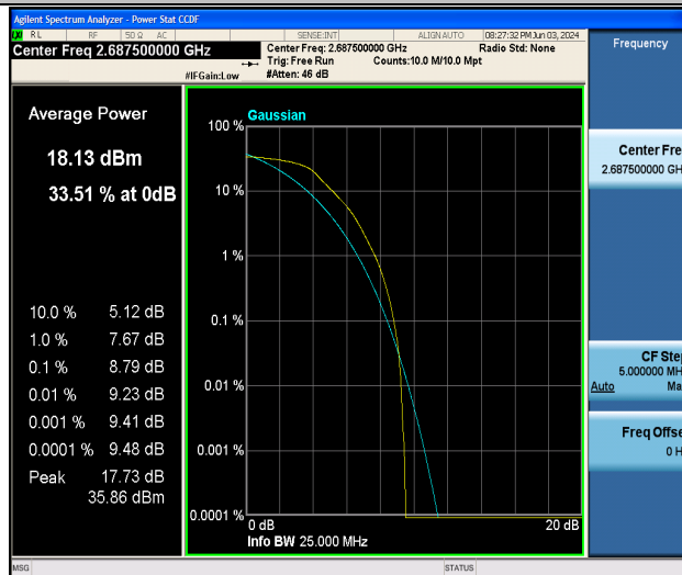
Band41-5MHz-QPSK-41565-25RB#0-PASS
