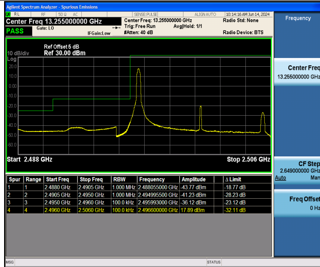
Band41_10MHz_16QAM_39700_1RB#0
