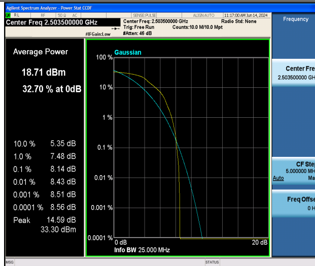
Band41-15MHz-QPSK-39725-1RB#0-PASS
