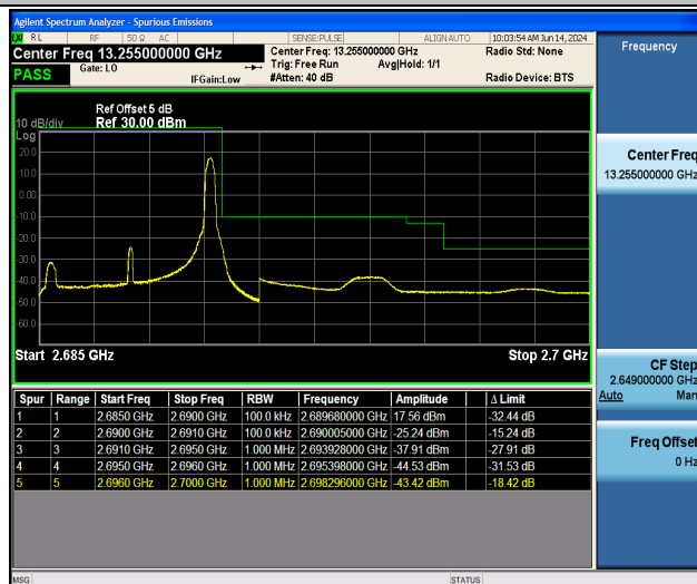
Band41_5MHz_16QAM_41565_1RB#24
