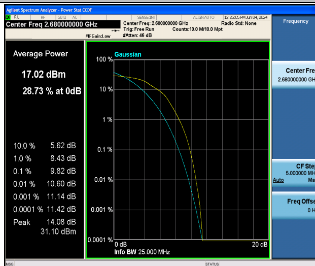
Band41-20MHz-16QAM-41490-100RB#0-PASS
