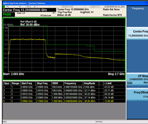
Band41_5MHz_QPSK_41565_25RB#0
