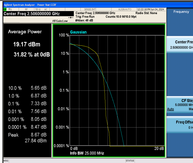
Band41-20MHz-16QAM-39750-1RB#0-PASS
