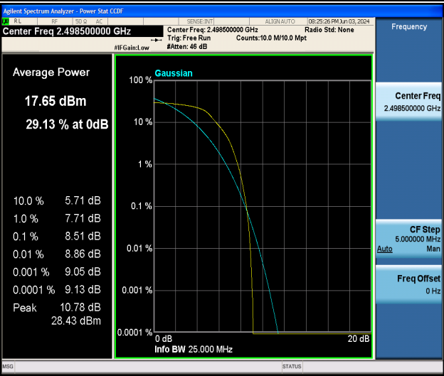
Band41-5MHz-QPSK-39675-25RB#0-PASS
