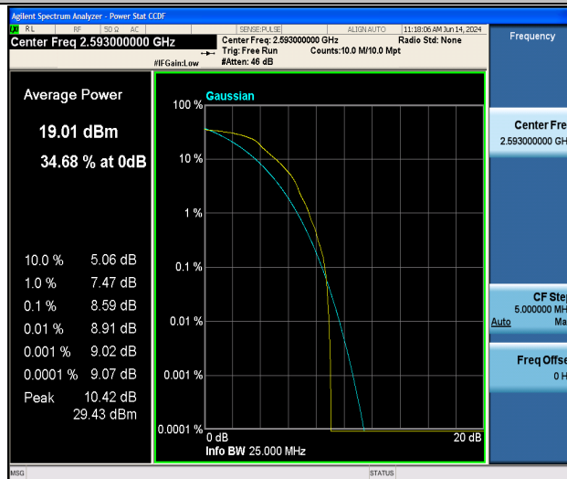
Band41-15MHz-QPSK-40620-1RB#0-PASS
