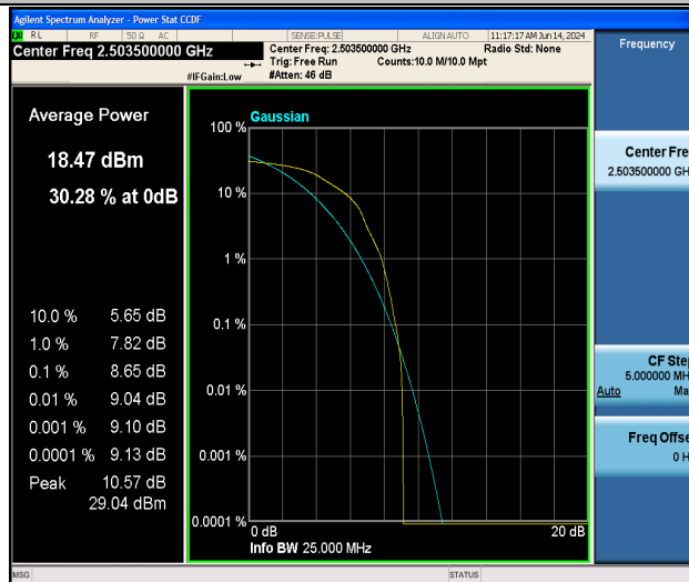
Band41-15MHz-16QAM-39725-1RB#0-PASS
