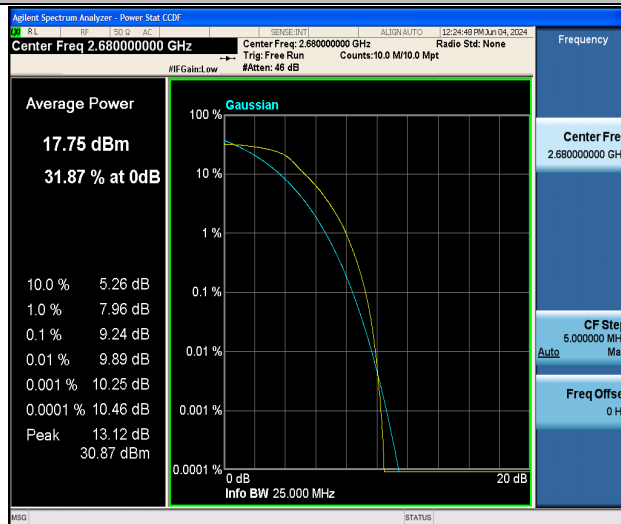
Band41-20MHz-QPSK-41490-100RB#0-PASS
