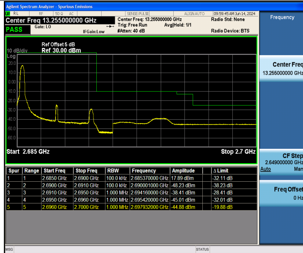
Band41_5MHz_16QAM_41565_1RB#0
