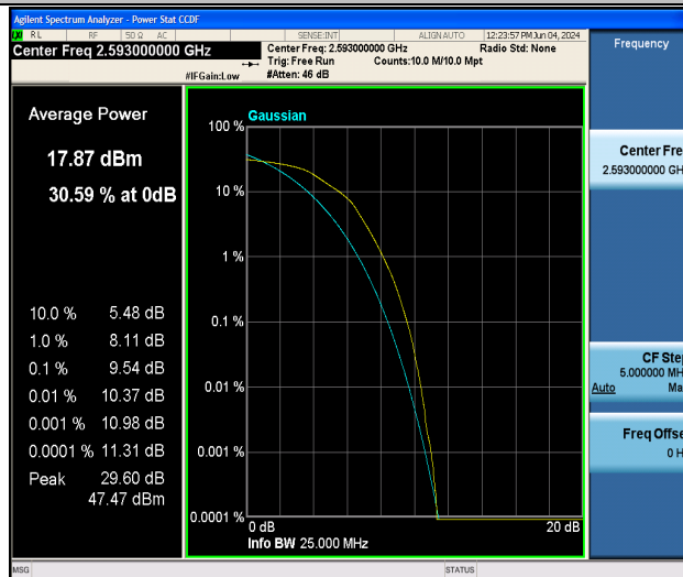
Band41-20MHz-16QAM-40620-100RB#0-PASS
