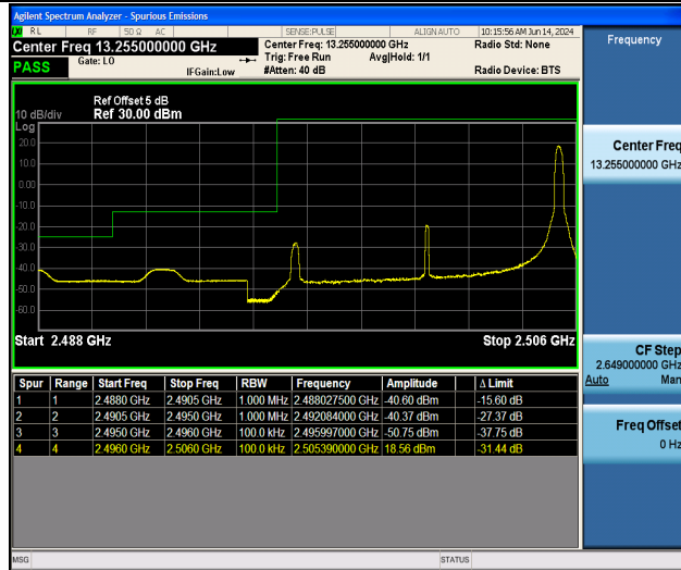
Band41_10MHz_QPSK_39700_1RB#49
