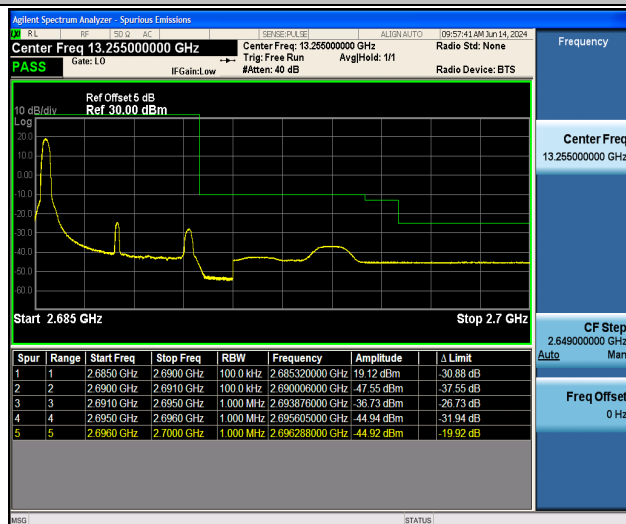
Band41_5MHz_QPSK_41565_1RB#0
