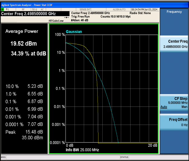
Band41-5MHz-QPSK-39675-1RB#0-PASS
