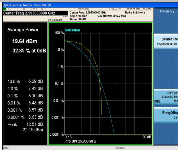
Band41-5MHz-QPSK-40620-1RB#0-PASS
