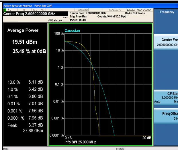
Band41-20MHz-QPSK-39750-1RB#0-PASS
