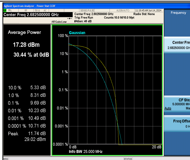
Band41-15MHz-QPSK-41515-75RB#0-PASS
