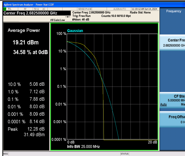
Band41-15MHz-QPSK-41515-1RB#0-PASS
