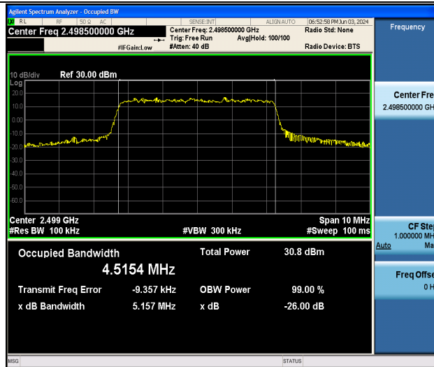
Band41-5MHz-QPSK-39675-25RB#0-PASS
