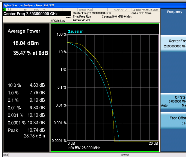
Band41-15MHz-QPSK-40620-75RB#0-PASS
