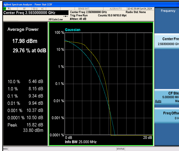
Band41-10MHz-QPSK-40620-50RB#0-PASS
