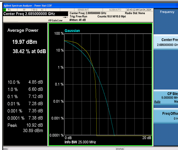
Band41-10MHz-QPSK-41540-1RB#0-PASS
