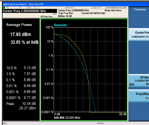
Band41-10MHz-QPSK-41540-50RB#0-PASS
