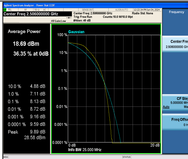
Band41-20MHz-QPSK-39750-100RB#0-PASS
