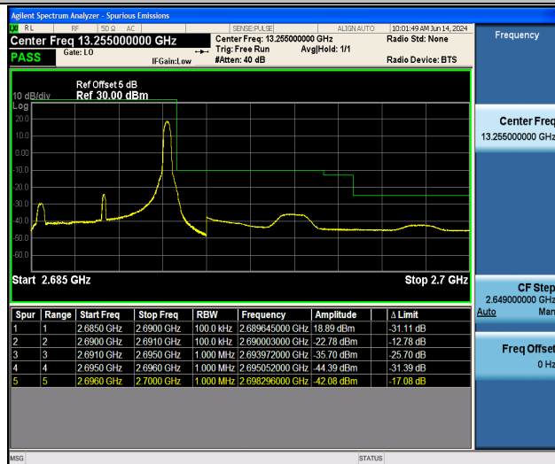
Band41_5MHz_QPSK_41565_1RB#24
