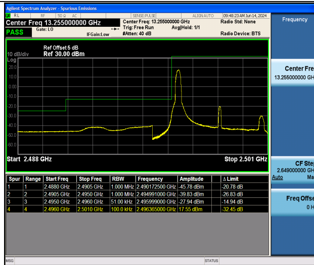
Band41_5MHz_16QAM_39675_1RB#0
