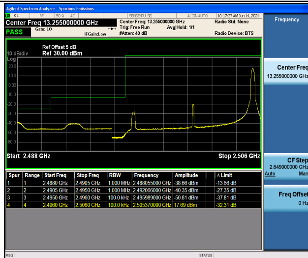
Band41_10MHz_16QAM_39700_1RB#49
