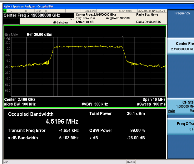
Band41-5MHz-16QAM-39675-25RB#0-PASS
