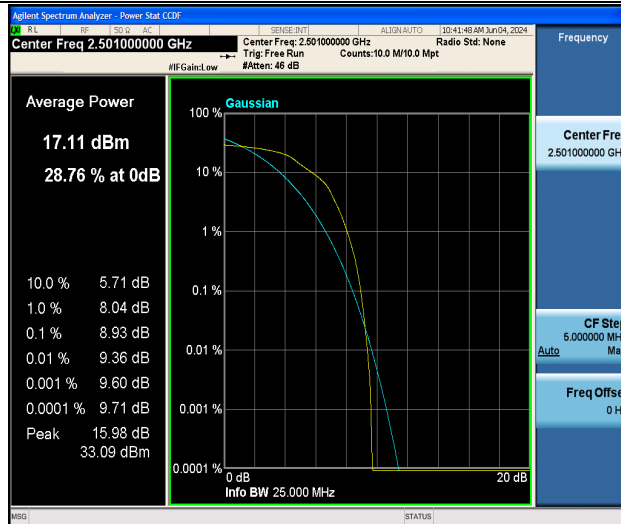
Band41-10MHz-16QAM-39700-50RB#0-PASS
