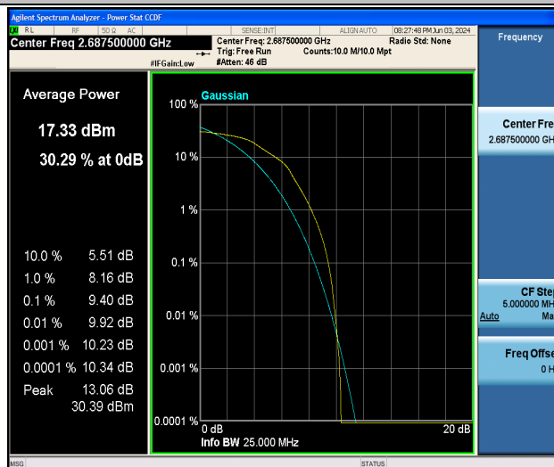
Band41-5MHz-16QAM-41565-25RB#0-PASS
