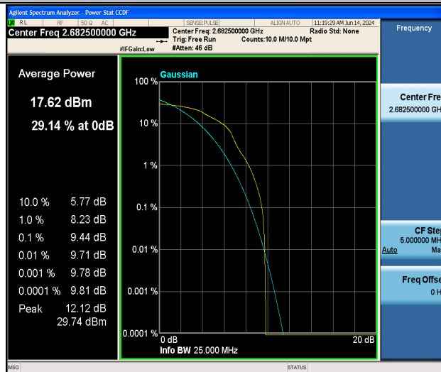
Band41-15MHz-16QAM-41515-1RB#0-PASS
