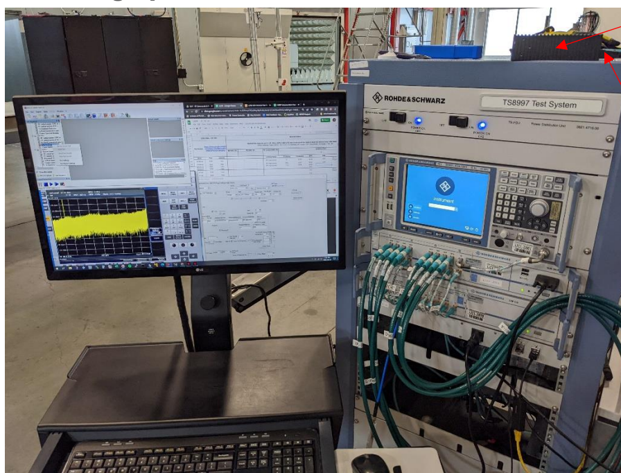
Photograph 4: Test Set Up Direct Connect
